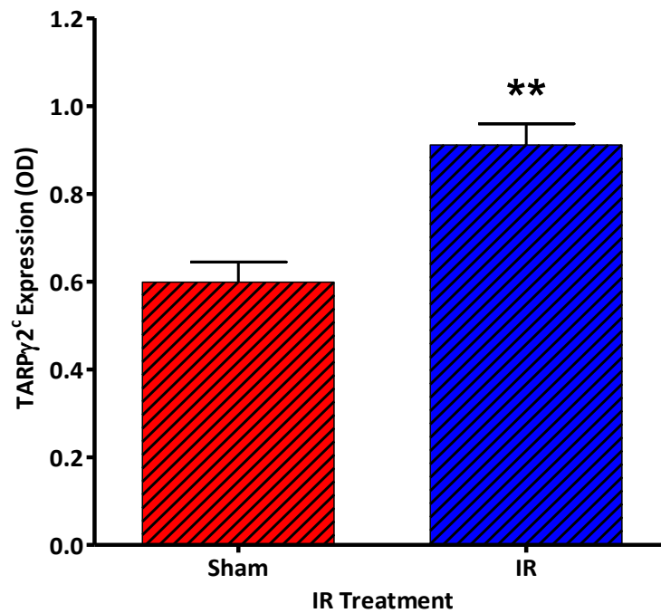
Figure 5.11. TARP \gamma 2 expression in chronic IR1072 preconditioned ( in vivo ) 13 month CD-1 male mice and Sham age matched controls. Each lane in A) demonstrates an individual mouse (n=4 for each condition) and B) represents quantitative analysis of TARP \gamma 2 expression, demonstrating a significant increase in TARP \gamma 2 expression following chronic IR1072 treatment, compared to sham treated animals, **p<0.01, Mean \pm SEM. Abbreviations: TARP \gamma 2, Transmembrane AMPA regulatory protein; OD, optical density.
