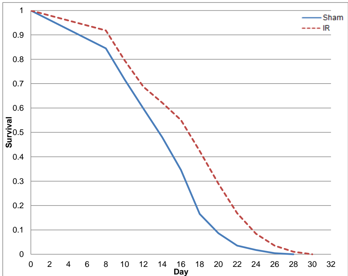
Figure 7.5. Lifespans of SS104, glp-4 (bn2)I , nematodes exposed to IR1072 as described in 2.9.3, and sham treated controls, n=2 repeat lifespans.
