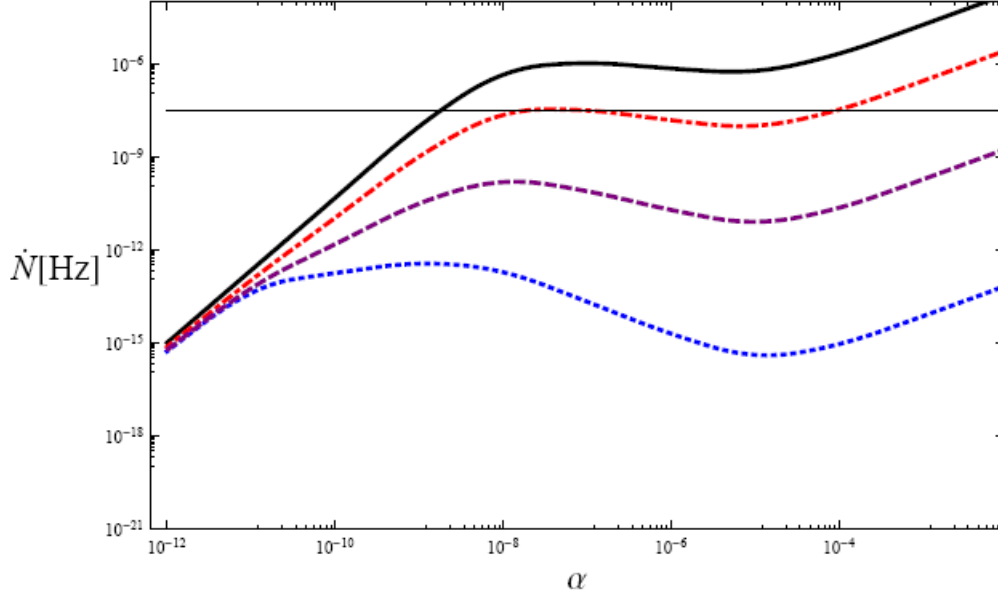
Figure 4.8: The rate of gravitational wave bursts at the LIGO frequency, f = 150\text{Hz} , at the amplitude 10^{-21}s^{-1/3} . \Delta_0 is fixed at 10^{-3} . From the top line, moving downwards, we have n = 0, 1, 3 and 6 . As above, P = 10^{-3} , and the horizontal line is a rate of 1 per year. Figure from [126].
