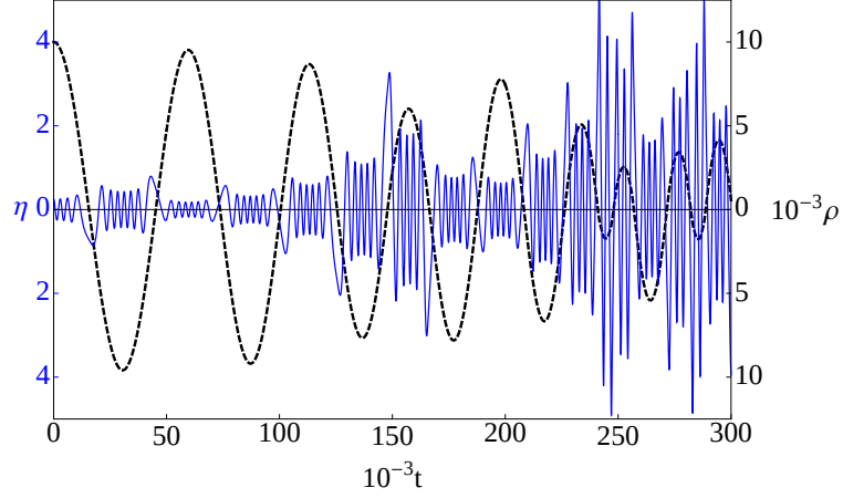
Figure 5.7: Including the gravitational radiation damping into the circular loops of section 5.1.2. The loop shown has no angular momentum, and corresponds to the damped version of the first plot in Figure 5.1. A rather large value of damping was chosen, corresponding to a halving of E_0 by the end of the integration.
