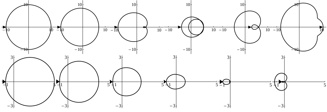
Figure 5.3: From left to right, snapshots of a string loop at evenly spaced time intervals, the upper sequence showing the loop in the external dimensions, and the lower sequence in the internal dimensions. This solution demonstrates how the circular shape is distorted by internal motion, and develops apparent kinks and crossings (although the loop does not self intersect as it misses in the internal dimensions). The arrow denotes the position on the loop where \zeta = 0 for comparison of the location of the features.
