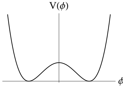
Figure 2.1: Potential for the \phi^4 -kink.
