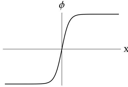
Figure 2.2: The \phi^4 -kink.
