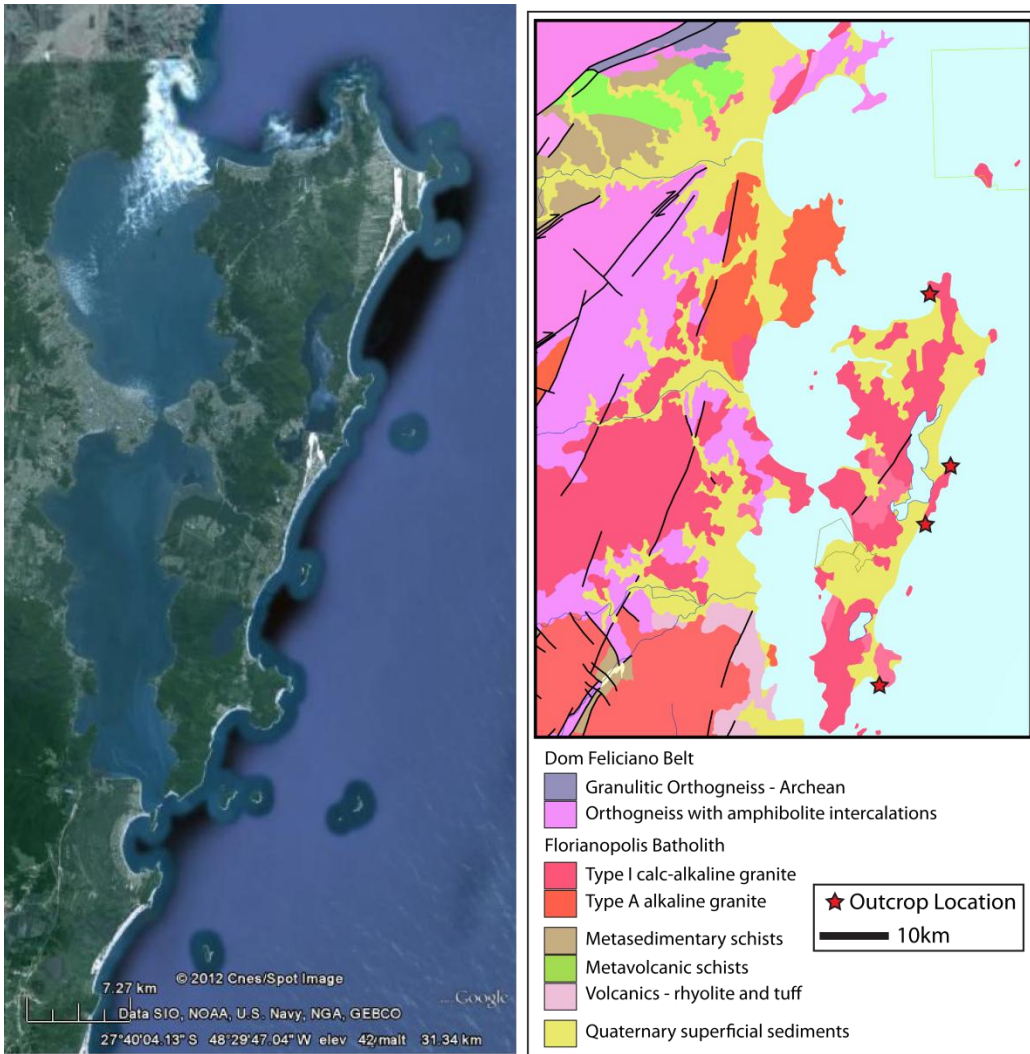
Figure 5.58 A. A Google earth aerial image of the island of Florianopolis, where 4 of the outcrops from the Florianopolis dyke swarm are located. B. Geological map of the study area, showing key lithologies and structures (black lines).
