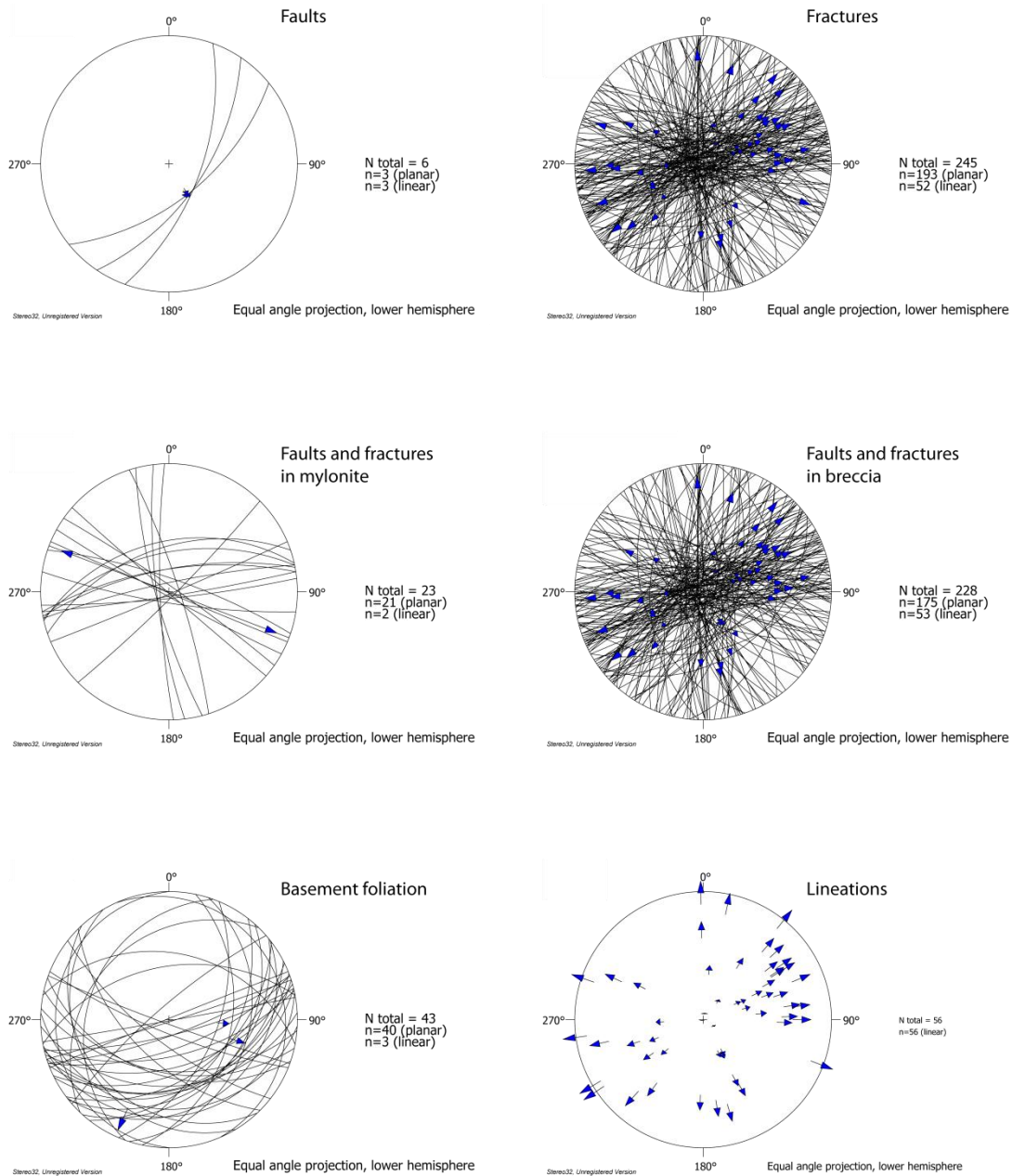
Figure 5.24 Stereonets of structural data collected from Quatis. Equal angle projections. Planes are shown as black lines, and lineations as blue arrows.
