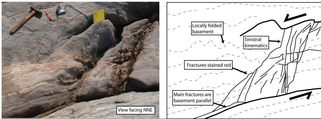
Figure 5.19A. A sinistral dilational step between two basement parallel fractures at Mambucaba. While it is difficult to make direct observations of offsets along these structures, due to their basement parallel nature, and low displacements, geometries such as these are useful in establishing kinematics. Red staining like this is typical of fractures across the region.
