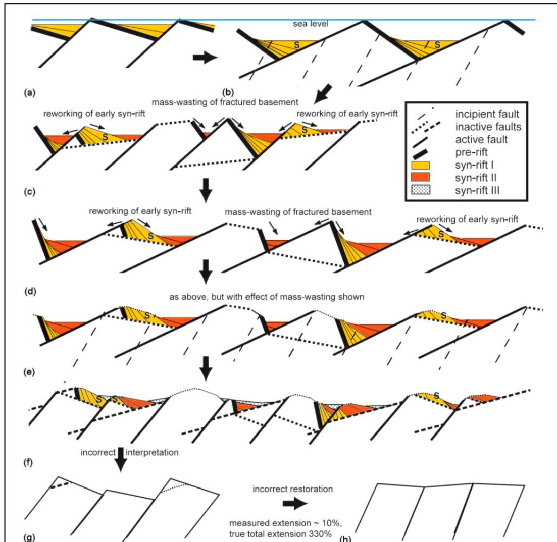
Figure 3.23. The 'fault rotation model' (Reston, 2009). Whilst not incompatible with other models for hyperextension, this model predicts multiple phases of rifting on structures which form due to pre-existing structures rotating to angles at which they are unable to slip. Careful attention needs to be paid to restoring such models, as their complex geometries are often difficult to interpret.
