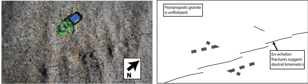
Figure 5.61A. NNE-SSW trending en-echelon fractures within the granite at Praia Galhetas. These individual fractures do not accommodate any apparent offset, but their geometry suggests dextral kinematics.
