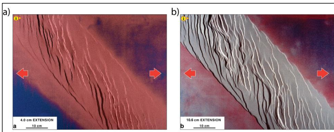
Figure 3.3 – Analogue models of oblique rifting, at \alpha = 45^\circ . As rifting progresses, faults in the rift appear to form at 90^\circ to the extension direction, whilst transfer zones, parallel to the rift margins form (McClay et al., 2002).
