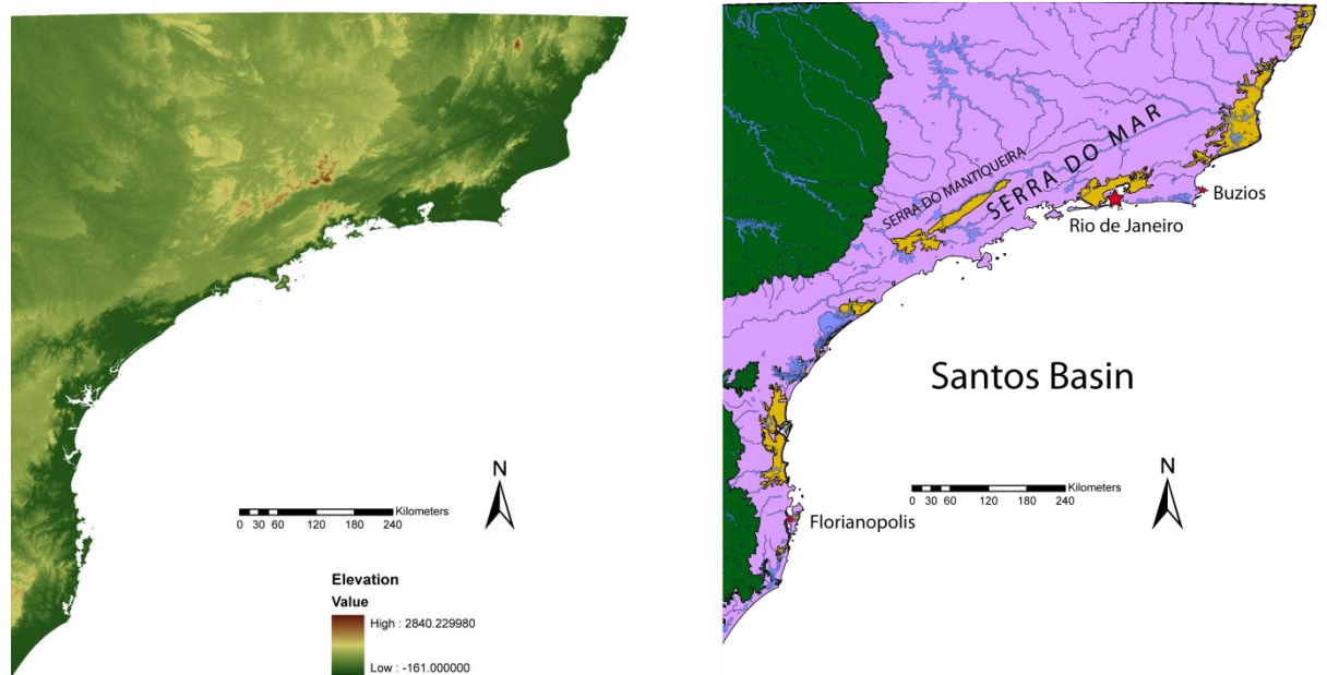
Figure 2.5 – Topography and simplified geology of the study area. The topographic map clearly shows the NE-SW trending mountain belts and basins (marked in yellow) formed during post-rift uplift. The geology map shows the Paraná basin marked in green, whilst the majority of basement – Brasiliano and older crystalline rocks, are marked in pink. Note the strong coast-parallel drainage patterns. The onshore study area extends between Buzios to the northeast, and Florianopolis to the southwest. Geology modified from Davison et al (1999).
