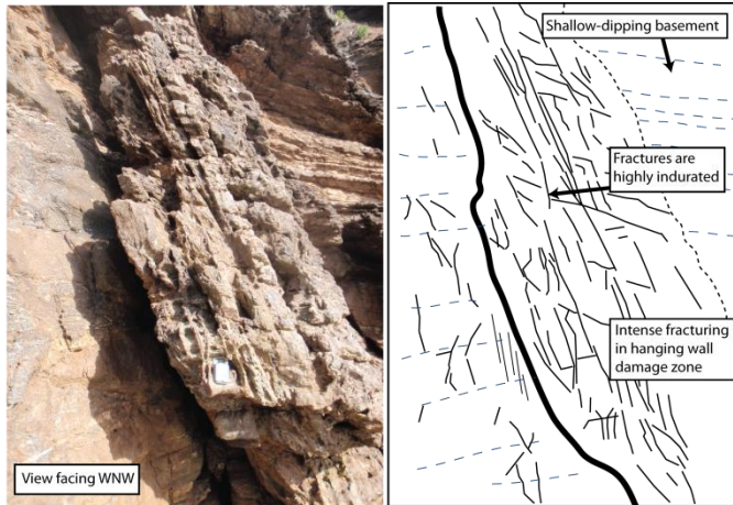
Figure 5.5a. The large fault at the southeast of Praia de Focas outcrop, cutting shallowly dipping basement foliation. The fault and fractures are highly indurated with silica rich material. Complex fracture networks in the hanging wall contrast with relatively little fracturing in the footwall. Oblique slip slickensides suggest dextral-normal kinematics. Compass for scale in bottom-centre of image.
