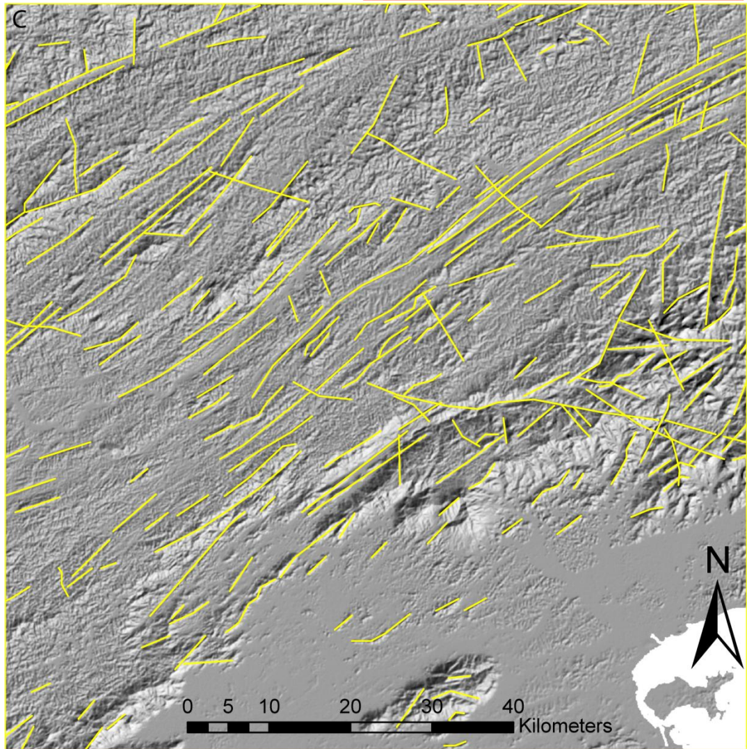
Figure 4.4 – The same region of hillshaded data shown at 1:3,000,000 scale (A), 1:1,000,000 scale (B), and 1:500,000 scale (C), along with lineaments picked at those scales.
