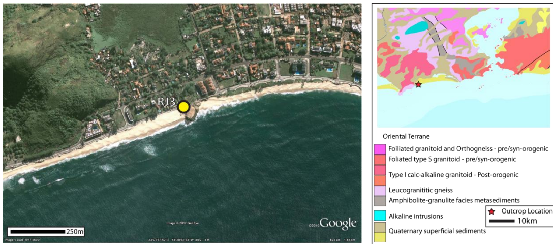
Figure 5.15 A. Google earth aerial photograph of the outcrop region around Grumari, showing the locations of outcrops visited (yellow circles). B. geological map of the area, showing key basement lithologies and structures (black lines).
