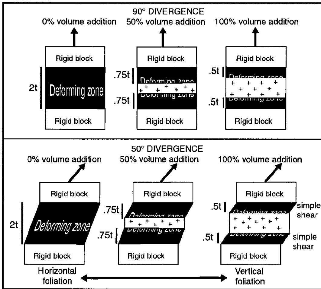
Figure 3.7 – Volume addition during transtension. The deforming region has an initial width ‘t’ As volume is added into a transtensional system (bottom of diagram), deformation focuses on refines with smaller values of ‘t’. Deforming regions therefore become more wrench dominated in order to accommodate the oblique component of extension. (Teyssier and Tikoff, 1999).
