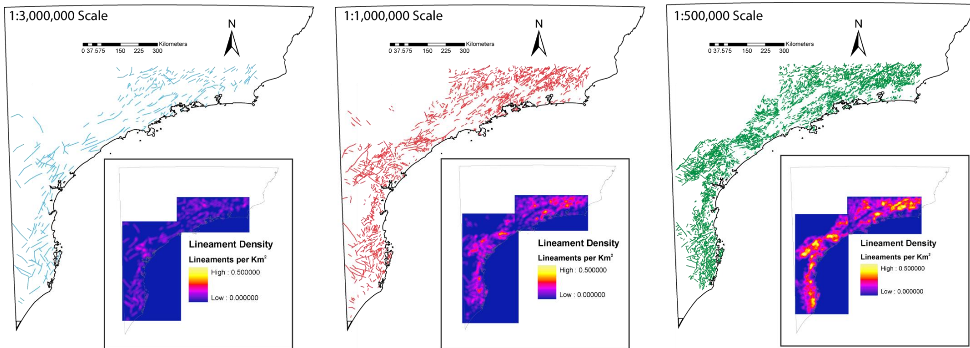
Figure 4.5. Lineaments picked from the SRTM data for SE Brazil, at 1:3,000,000, 1:1,000,000 and 1:500,000 scales. The insets show the density of the lineaments across the area. Many more lineaments are picked at smaller scales, however, lineament trends remain relatively similar, as do their density variations. Lineaments are typically less dense in the Cenozoic sedimentary basins than in the mountainous regions that surround them, due largely to the lack of topography in the basins. The Cabo Frio terrane, to the east of the area is almost devoid of lineaments at all scales.
