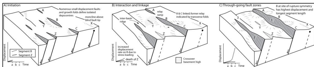
Figure 3.25 - Fault linkage and propagation during early rifting (Gawthorpe and Leeder, 2000).
