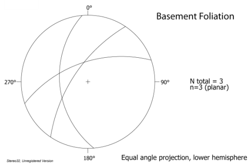
Figure 5.53. Stereonets of structural data collected at Guaratuba. Equal angle projections. Planes are shown as black lines, and lineations as blue arrows.
