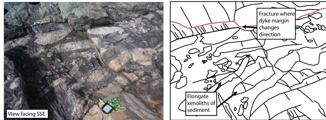
Figure 5.73C. These xenoliths form an 'intrusion breccia', consisting of a number of pieces of basement, with a wide array of sizes, situated around the dyke margins at Pantano do Sul. The xenoliths are tabular in shape, and oriented parallel to the dyke margins. They consist mainly of clasts of the volcanoclastics seen at this outcrop, but occasionally clasts of granite can be seen.
