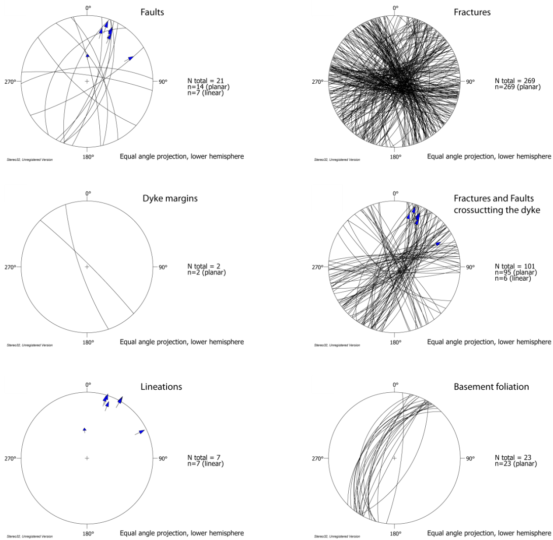
Figure 5.50. Stereonets of structural data collected on Ilha do Mel. Equal angle projections. Planes are shown as black lines, and lineations as blue arrows.
