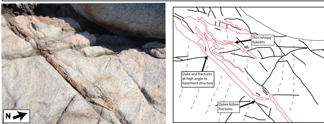
Figure 5.9C. Smaller dykes seen at Praia das Conchas. While the larger of the small dykes in this image trends closely parallel to brittle fractures, there is a significant population of smaller dykes and dyke branches that show a more chaotic geometry,
