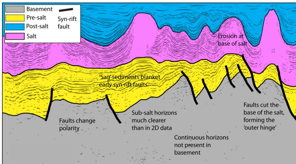
Figure 6.6. The 'outer hinge' in a line through the 3D seismic data. The 3D data typically offers higher quality imaging in the sub-salt section and much higher spatial resolution. Many more faults can be picked in this data than the 2D data and correlating structures between lines is easier. To the W, tilted fault blocks are seen in the basement immediately beneath the base of the salt. The presence of truncated syn-rift reflectors beneath the salt is good evidence for the basement having been sub-aerially exposed and eroded prior to the deposition of the salt. To the west towards the centre of the basin, faults are blanketed by a layer of sediments, with a relatively consistent thickness. These sediments are the sag horizons, deposited during thermal subsidence of the basin. Image is approx 35km wide, with approx. 6s TWTT vertical extent. Data Courtesy of CGG
