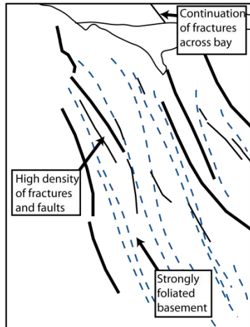
Figure 5.42A - Brittle fracturing and basement fabrics are strongly parallel at Guarujá, and basement fractures are planar. Across the bay, a continuation of this structure can be seen directly along strike.
