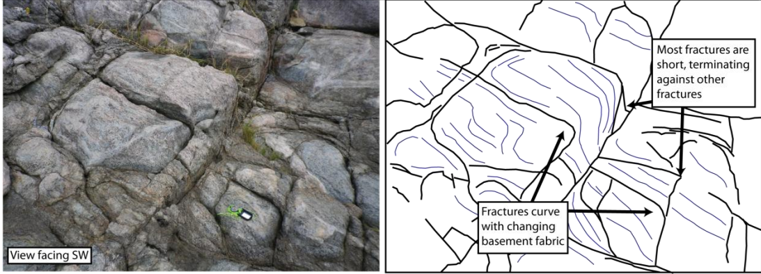
Figure 5.30C. At wpU1, local basement influence can be seen at Ponta Grossa, with complex basement structure affecting the outcrop pattern of fractures. Where basement is strongly foliated, fractures curve parallel to the foliation. Where foliation is weak or non-existent, fractures tend to be more continuous and less curved. Many smaller fractures appear to terminate against one another, rather than being crosscut.
