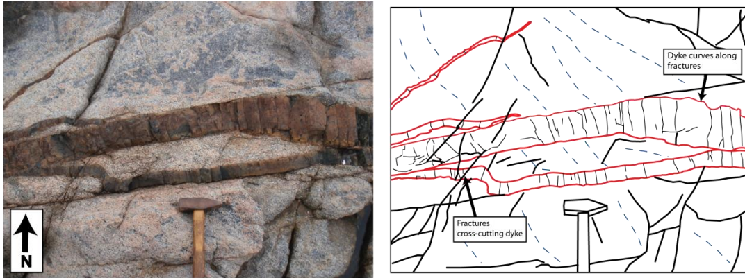
Figure 5.9A. A small dyke branching around a block of basement gneiss at Praia das Conchas. The dyke clearly follows fractures in the basement, branching between two NE-SW trending fractures. NNE-SSW fractures later crosscut the dyke. The dyke and fractures clearly crosscut the NNW-SSE trending basement,
