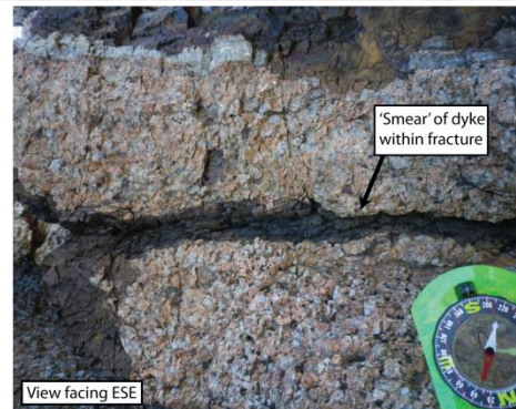
Figure 5.62C (above). Within the fault zone, smears of dyke material can be seen within the fractures, highlighting the fact that these fractures were present before the intrusion of the dyke, and that dyke material was clearly able to infill them.
