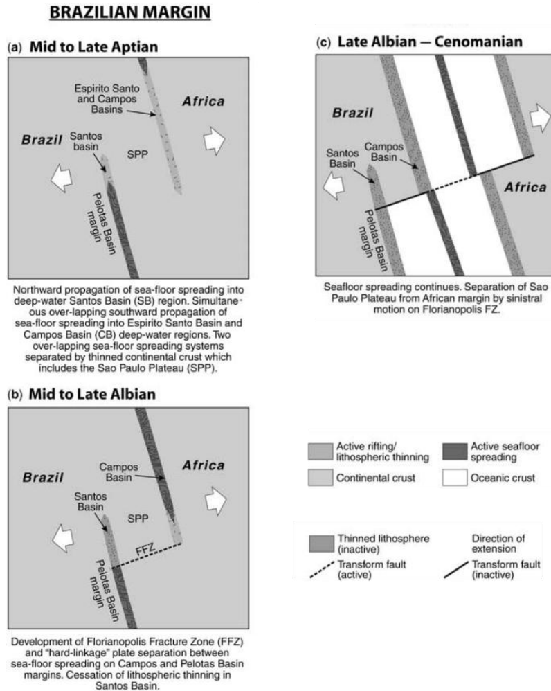
Figure 2.20. Ocean spreading in the South Atlantic, modified from Scotchman et al, 2010. Spreading initially propagates northwards into the Santos basin, before jumping to its current position in the central Atlantic.
