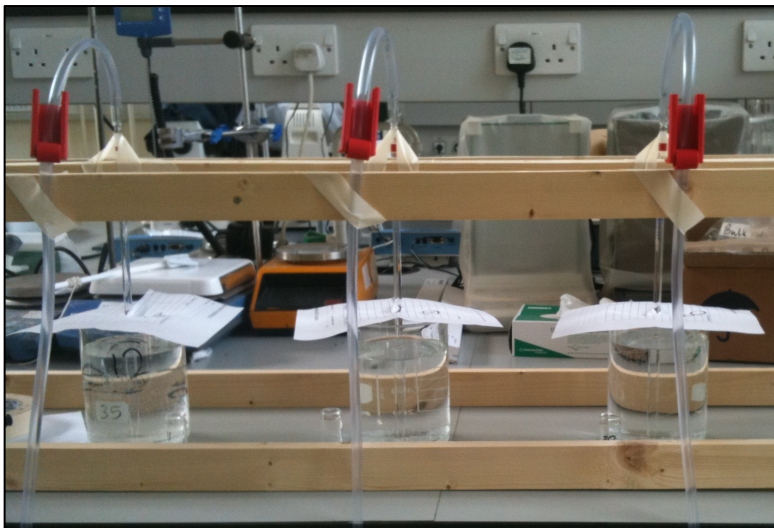
B Figure 3.2 A) Image of several of diatom absolute abundance apparatus running simultaneously. B) Close-up image of coverslips at bottom of beaker, with the pipette through the central hole of an inverted petri dish.
