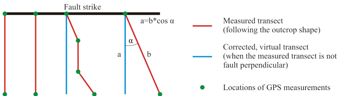
Figure 1.1 - 1D quantitative analysis
