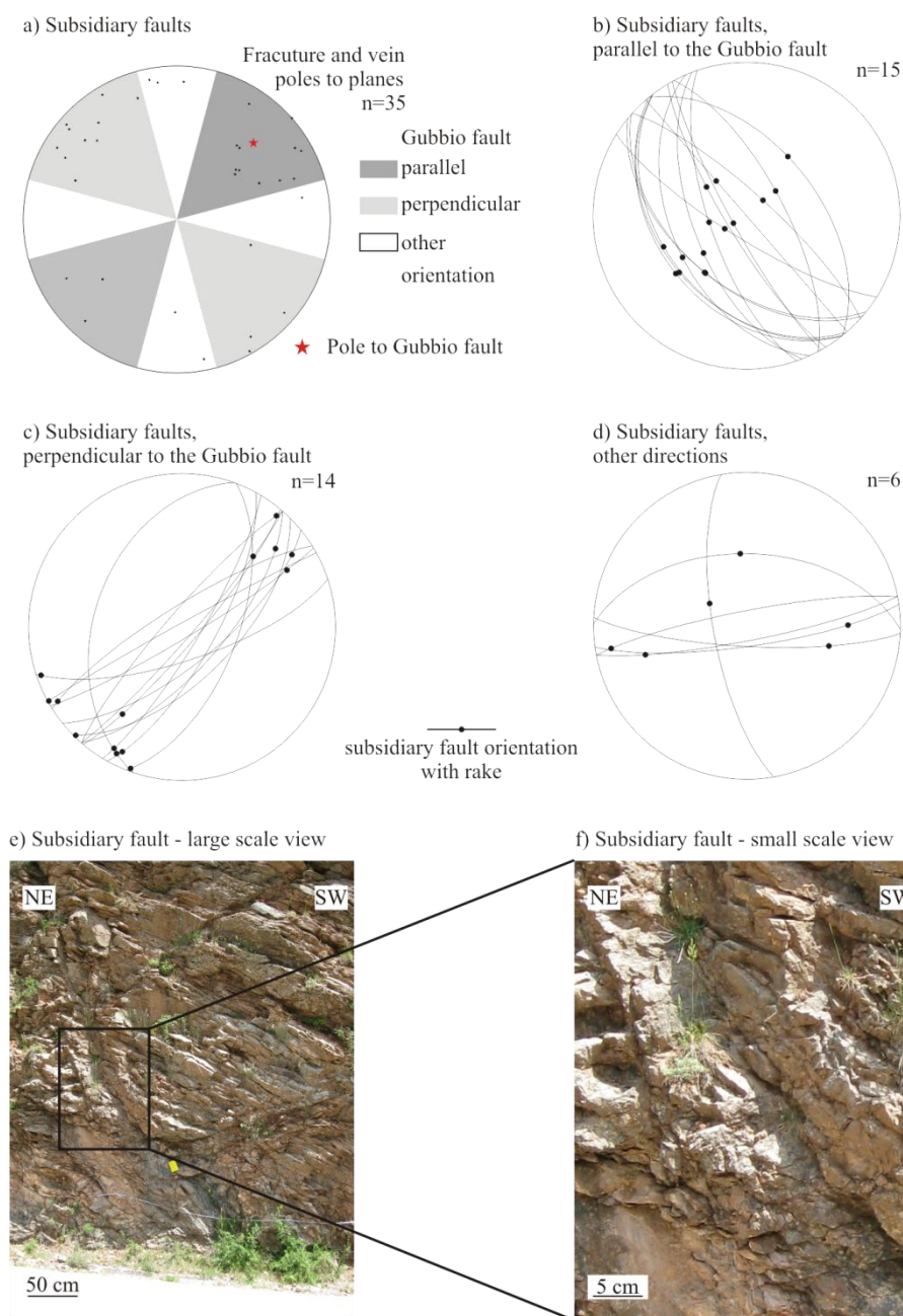
Figure 4.12 - The damage zone at L2 – subsidiary faults in the Scaglia Rossa formation
