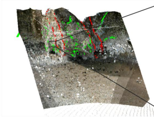
c) cells of the geocellular model intersected by the IBZ and FC boundaries
