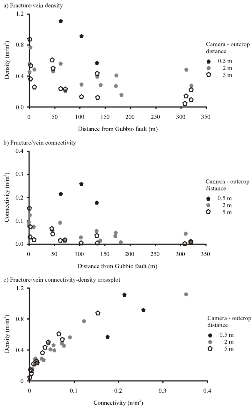
Figure 4.24 - Outcrop scale image analysis results by different camera-outcrop distance a) Fracture/vein density across the damage zone; b) Fracture/vein connectivity across the damage zone; c) Fracture/vein connectivity density crossplot across the damage zone
