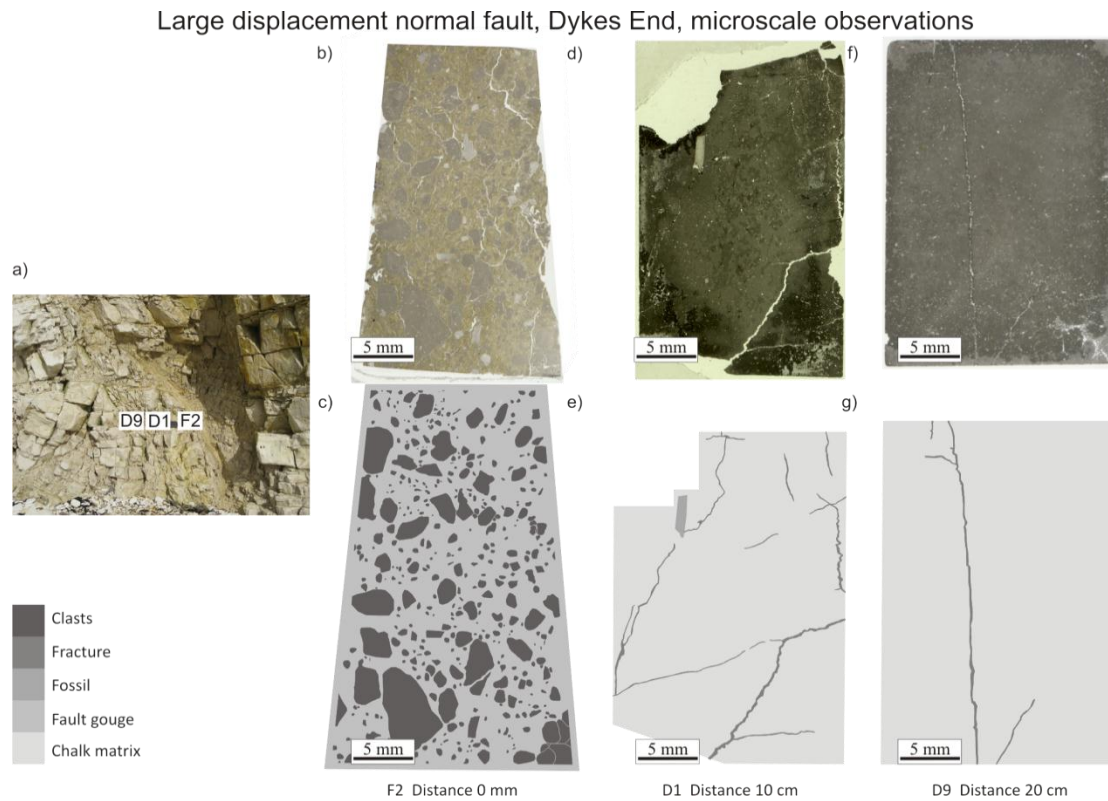
Figure 3.7 - Large displacement normal faults at Dykes End– microscale
