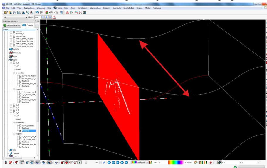
c) A fault parallel slice of the Sgrid with parts of a region highlighted
