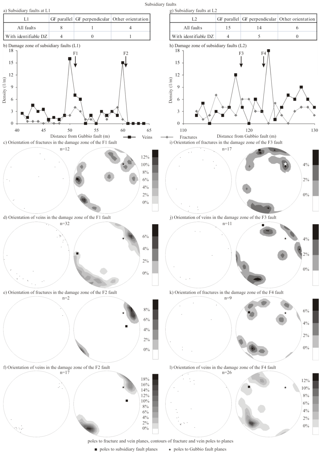
Figure 4.21 - Subsidiary faults
