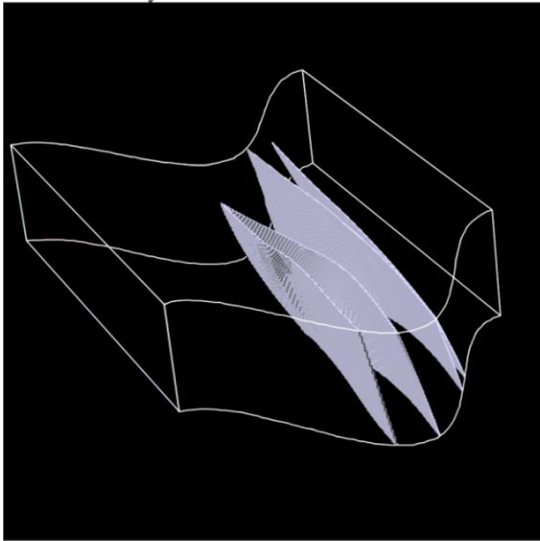
e) cells of the geocellular model intersected by intersection curves
