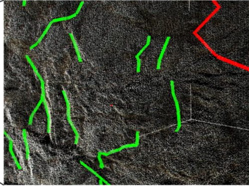
d) cells of the geocellular model intersected by fractures
