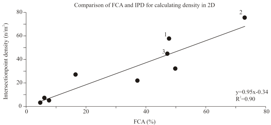
Figure 1.3 - Correlation between the two methods (IDP and FCA) to quantify fracture and vein connectivity in 2D
