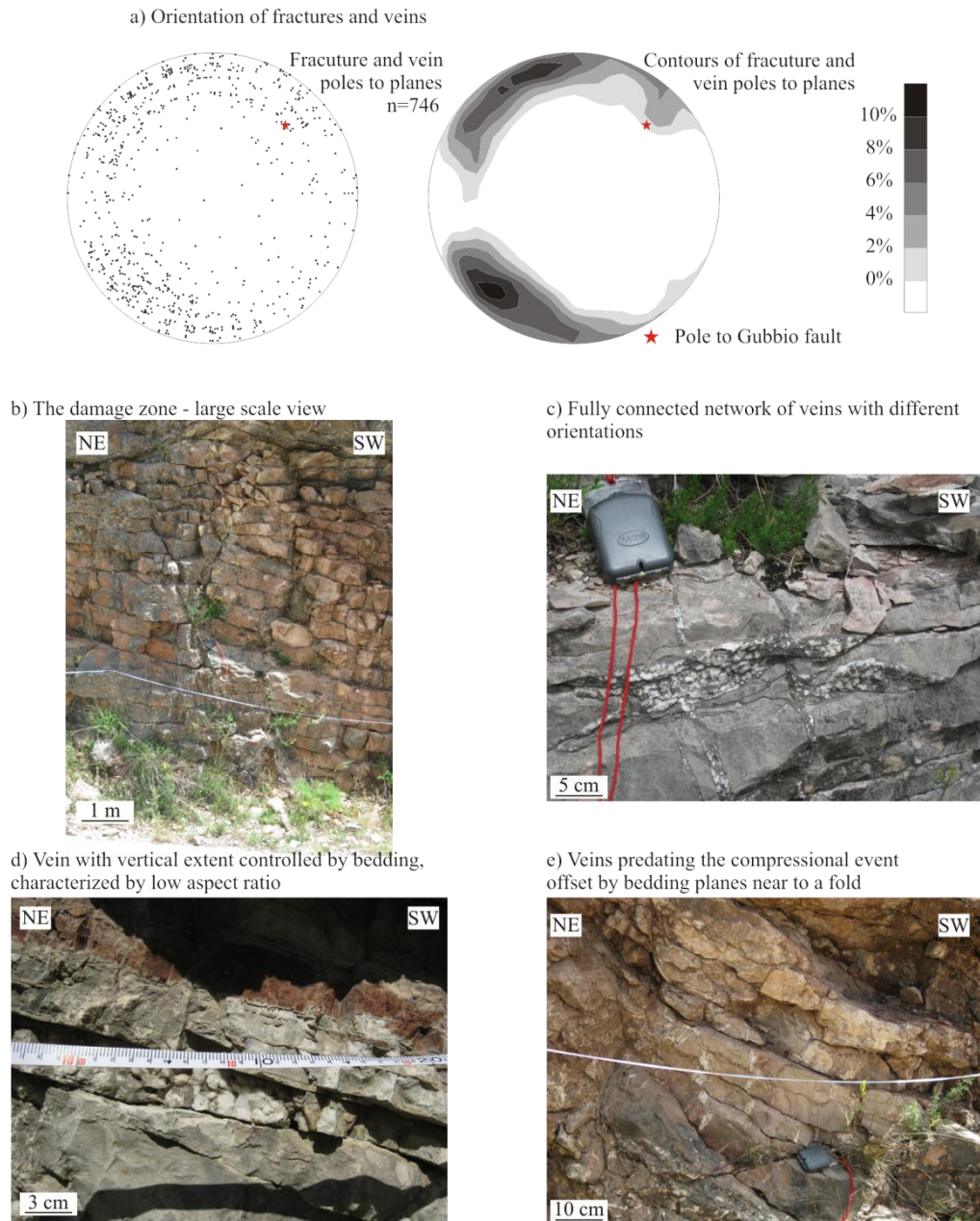
Figure 4.11 - The damage zone at L2 – fractures and veins in the Scaglia Rossa formation
