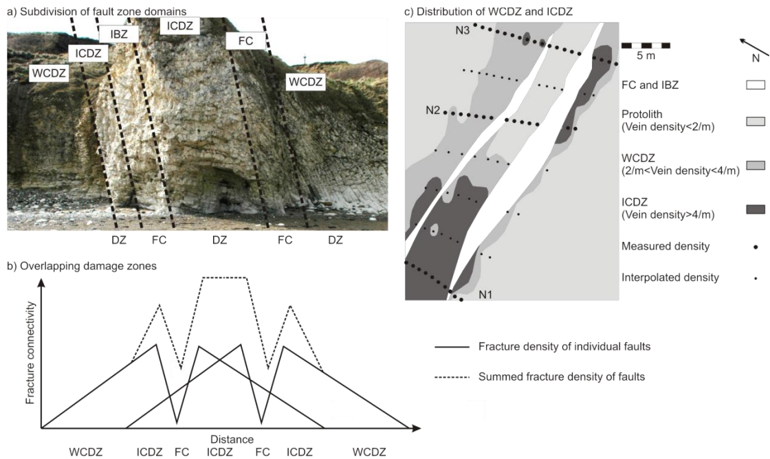
Figure 3.20 - Subdivision of the Selwick bay large displacement normal faults a) damage zones separated into WCDZ and ICDZ on the cliff, b) interpretation for the development of the WCDZ and ICDZ: ICDZs are the results of two overlapping damage zones, c) damage zones separated into WCDZ (light grey areas) and ICDZ (dark grey areas) on the cliff and on the wave-cut platform
