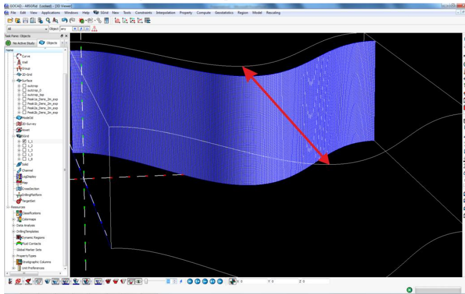
b) Cells of Sgrid intersected by fractures
