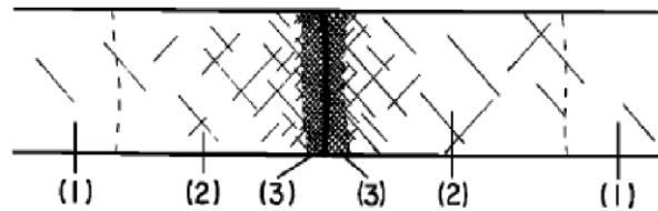
Figure 2.5 - Internal structure of faults
