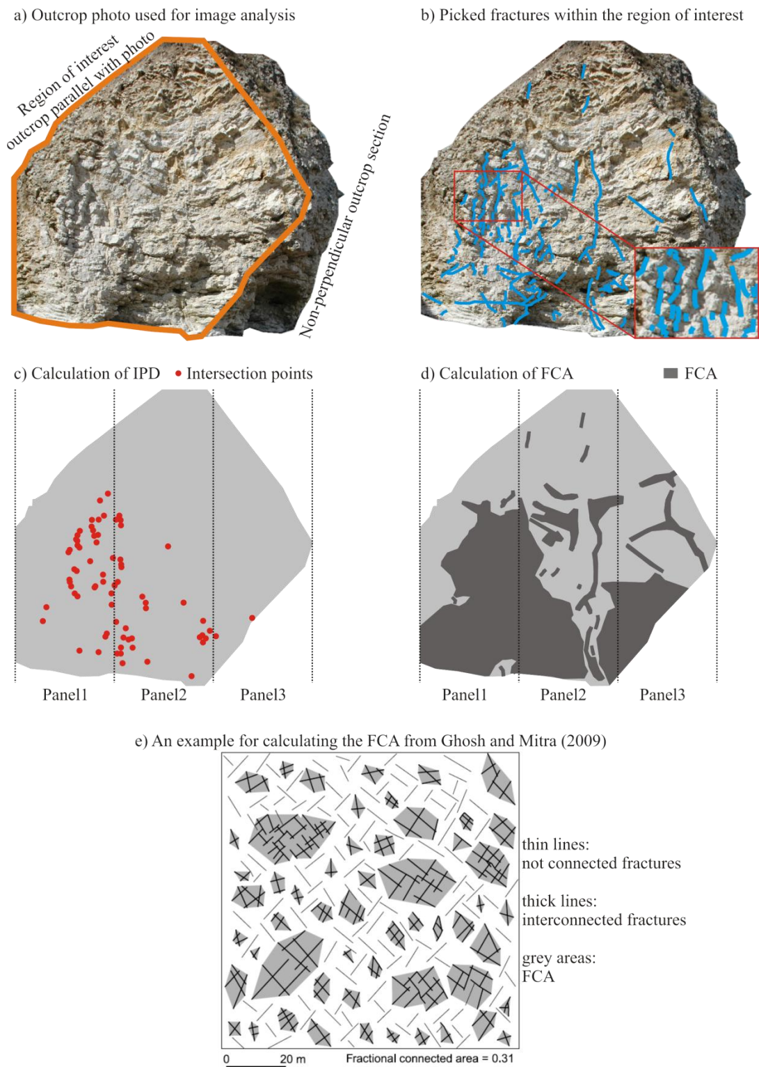
Figure 1.2 - 2D quantitative analysis
