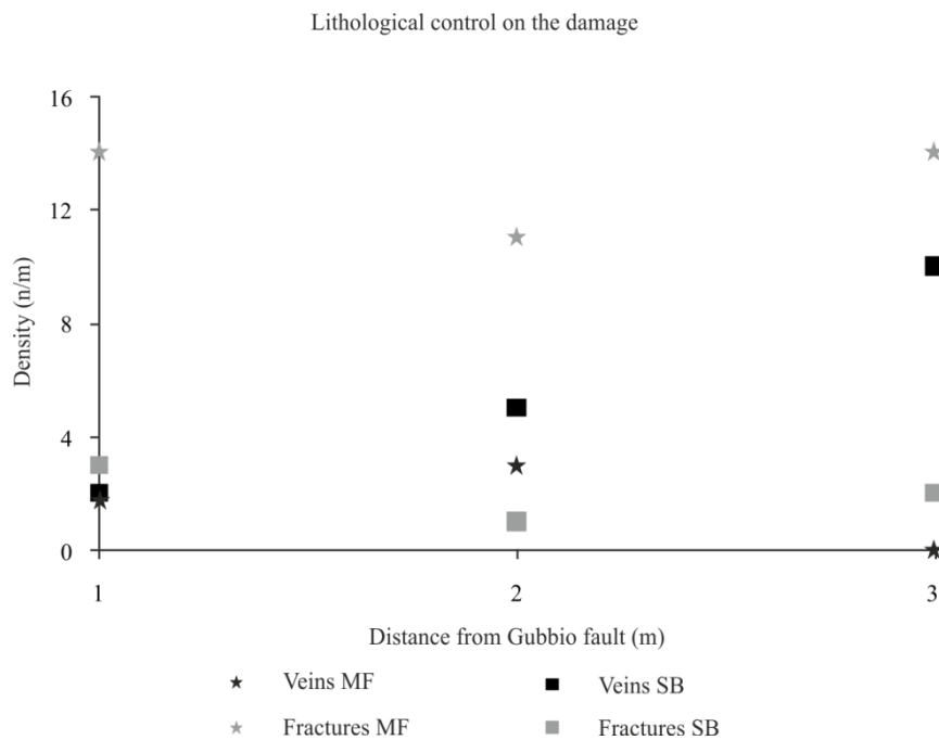
Figure 4.20 - Lithological control on the damage comparison of fracture and vein density values within the Scaglia Bianca and Marne a Fucoidi formations
