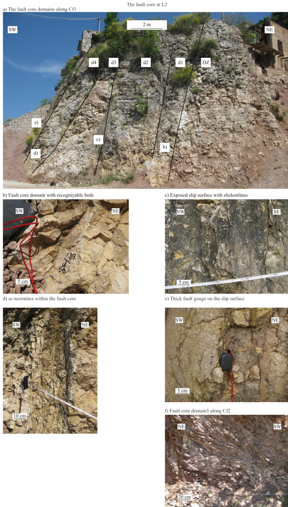
Figure 4.14 - The fault core at L2
