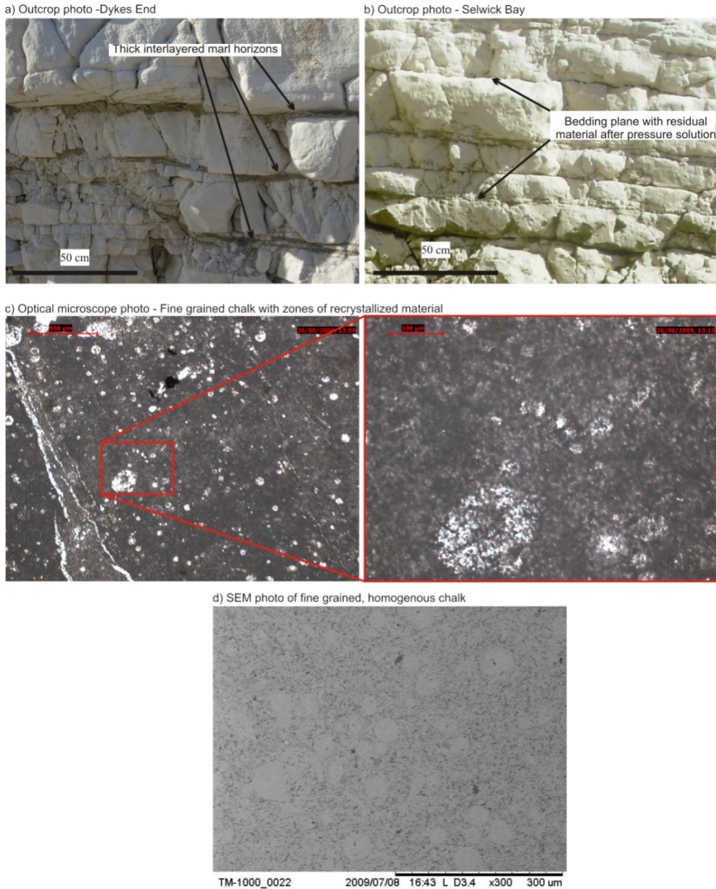
Figure 3.2 - The protolith
