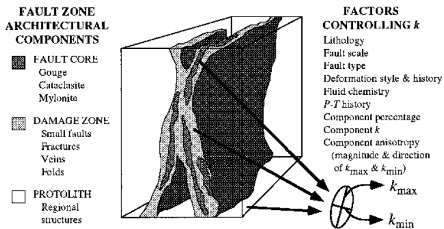
Figure 2.16 - Conceptual model of fault zone with protolith removed (after Chester and Logan, 1986; Smith et al., 1990). Ellipse represents relative magnitude and orientation of the bulk twodimensional permeability ( k ) tensor that might be associated with each distinct architectural component of fault zone (from Caine et al., 1996)
