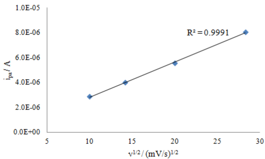
Figure 4.7. Plot of i_{pa} vs. v^{1/2} / (mV/s)^{1/2} for 20.
