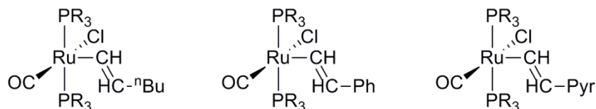
Figure 3.2. Five coordinate monometallic ruthenium vinyl complexes, where PR 3 = PPh 3 or P t Pr 3 .
