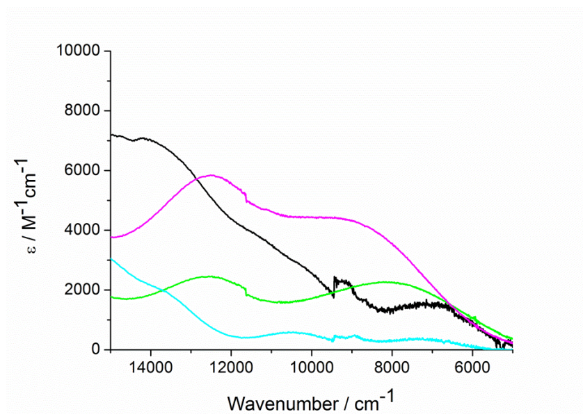
Figure 5.20. NIR transitions of the electrochemically generated [39a]^+ (black) and [42\text{-Me}]^+ (blue) in 0.1 M \text{NBu}_4\text{PF}_6 / \text{CH}_2\text{Cl}_2 and the chemically generated [40b]^+ (green) and [40b]^{2+} (purple) in \text{CH}_2\text{Cl}_2 at -40^\circ\text{C} .
