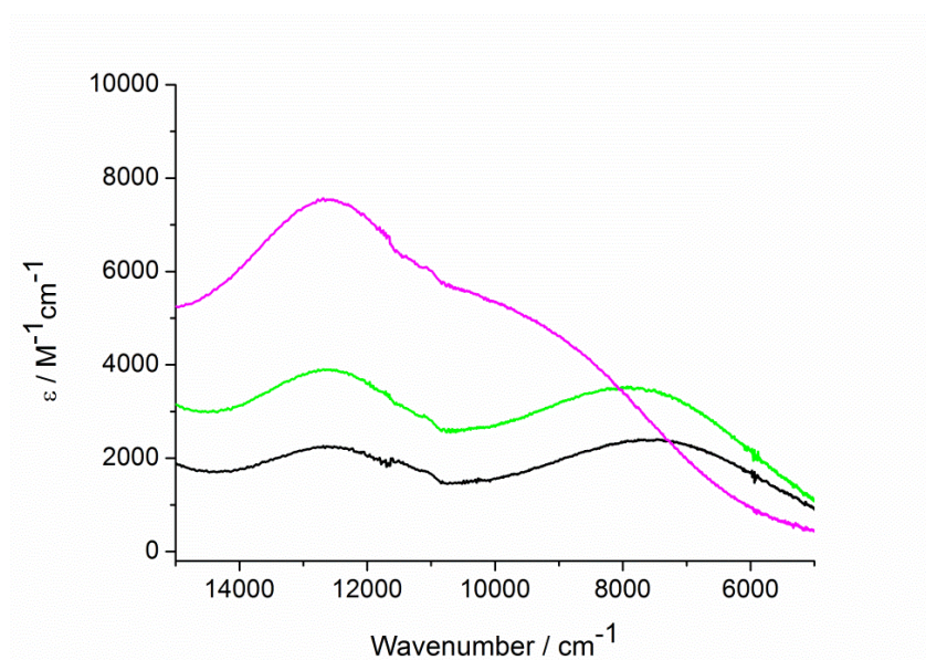
Figure 5.21. The NIR spectra of [41c]^+ (black), [41c]^{2+} (green), [41c]^{3+} (purple) obtained by stoichiometric oxidation with one, two and three equivalents of [\text{FcAc}]\text{PF}_6 in \text{CH}_2\text{Cl}_2 at -40^\circ\text{C} .
