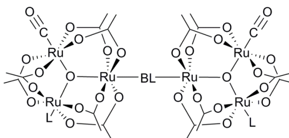
Figure 1.14. Ligand bridged bis(ruthenium) cluster complexes.
