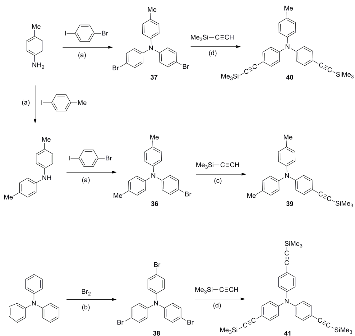
Scheme 5.1. Preparation of the ligands 39 , 40 and 41 . Conditions: (a) \text{Pd}_2(\text{dba})_3 / \text{dppf} / \text{NaO}^t\text{Bu} / toluene / reflux; (b) \text{Br}_2 , \text{CHCl}_3 , 0 °C; (c) \text{PdCl}_2(\text{PPh}_3)_2 / \text{CuI} / \text{NEt}_3 / reflux; (d) \text{Pd}(\text{PPh}_3)_4 / \text{CuI} / \text{NEt}_3 / reflux.
