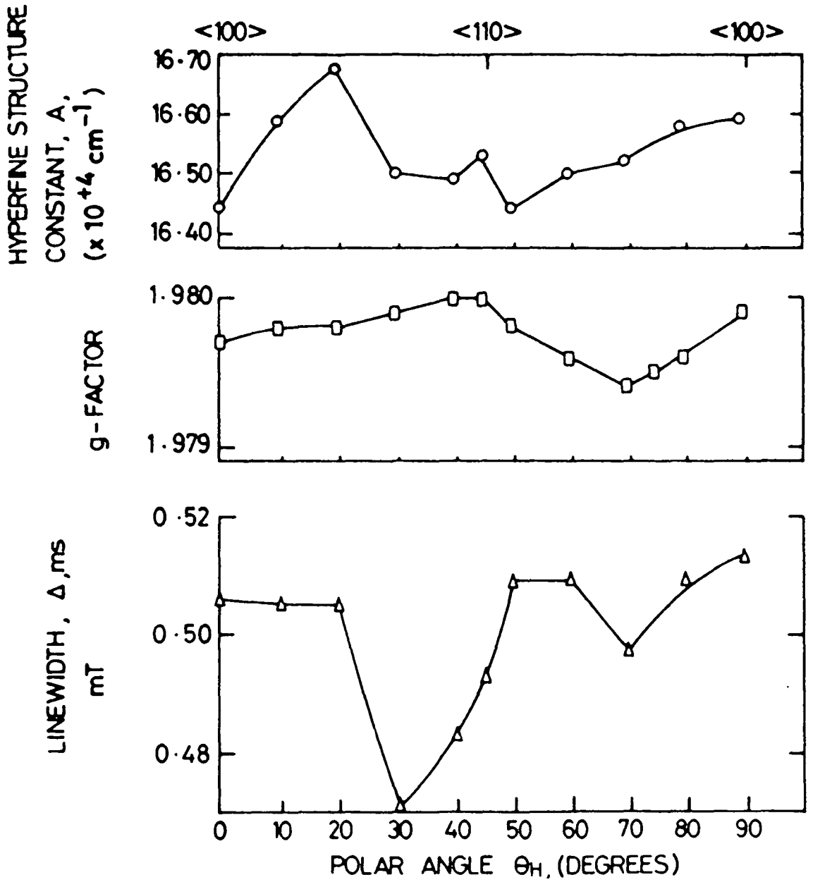
FIGURE 7.3 VARIATION OF A , g -FACTOR AND \Delta H_{ms} WITH POLAR ANGLE IN THE [100] PLANE; SINGLE CRYSTAL \text{Cr/MgO} , 800 p.p.m. \text{Cr} , 293K.
