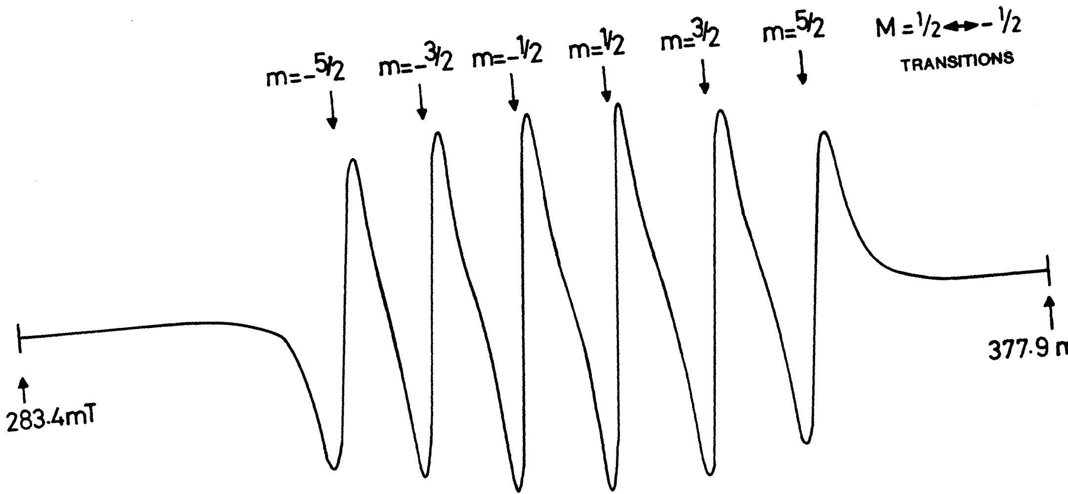
FIGURE 8.2(b) E.P.R. SPECTRUM OF SINGLE CRYSTAL Mn/MgO AT \theta = 32^\circ ; 2,900 p.p.m. Mn, 9.3815 GHz, 293K.
