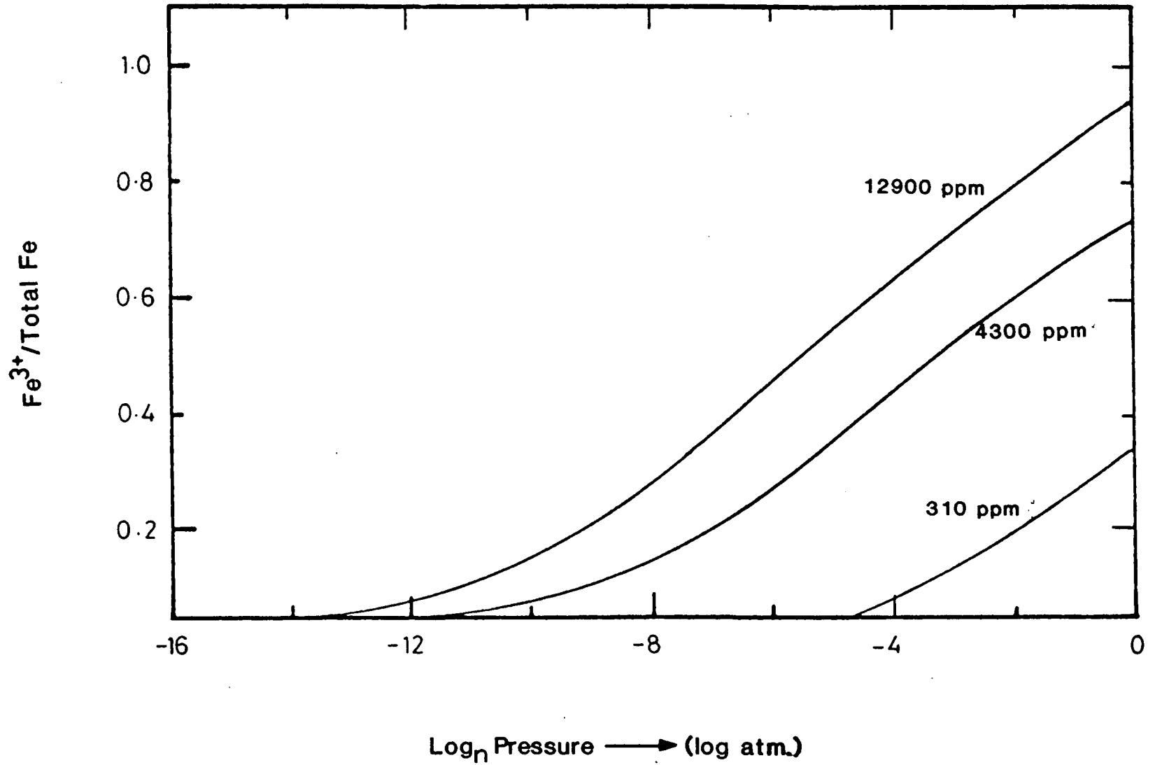
FIGURE 2.6(b) THE VARIATION OF THE FRACTIONAL CONCENTRATION OF Fe 3+ WITH TOTAL IRON CONTENT AND OXYGEN PRESSURE AT 1573K.
