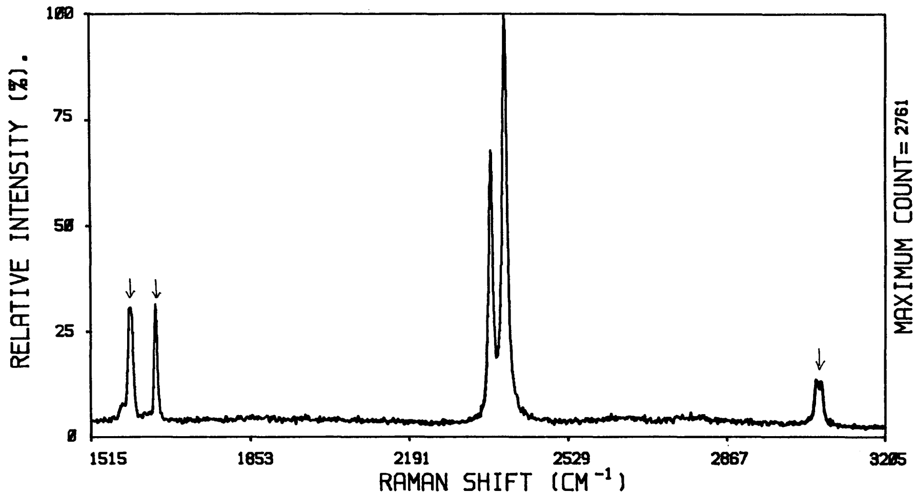
FIGURE 8.8 Gated spectrum of \text{Al}_2\text{O}_3 /benzophenone mixture (ca. 4 ns gate). The Raman bands ( \downarrow ) are clearly revealed, while the doublet and background features are greatly reduced in intensity.
