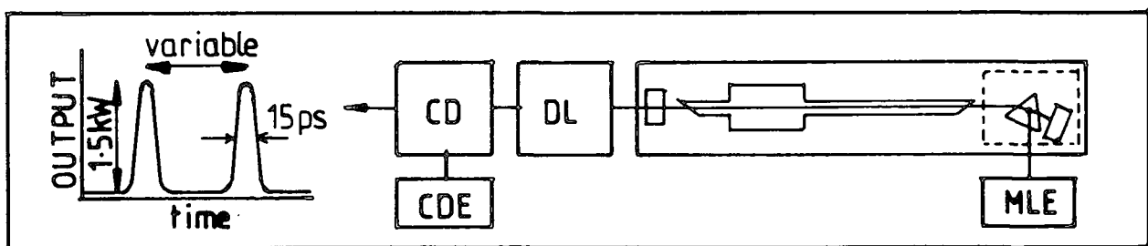
FIGURE 5.3 CW and pulsed dye laser configurations.
