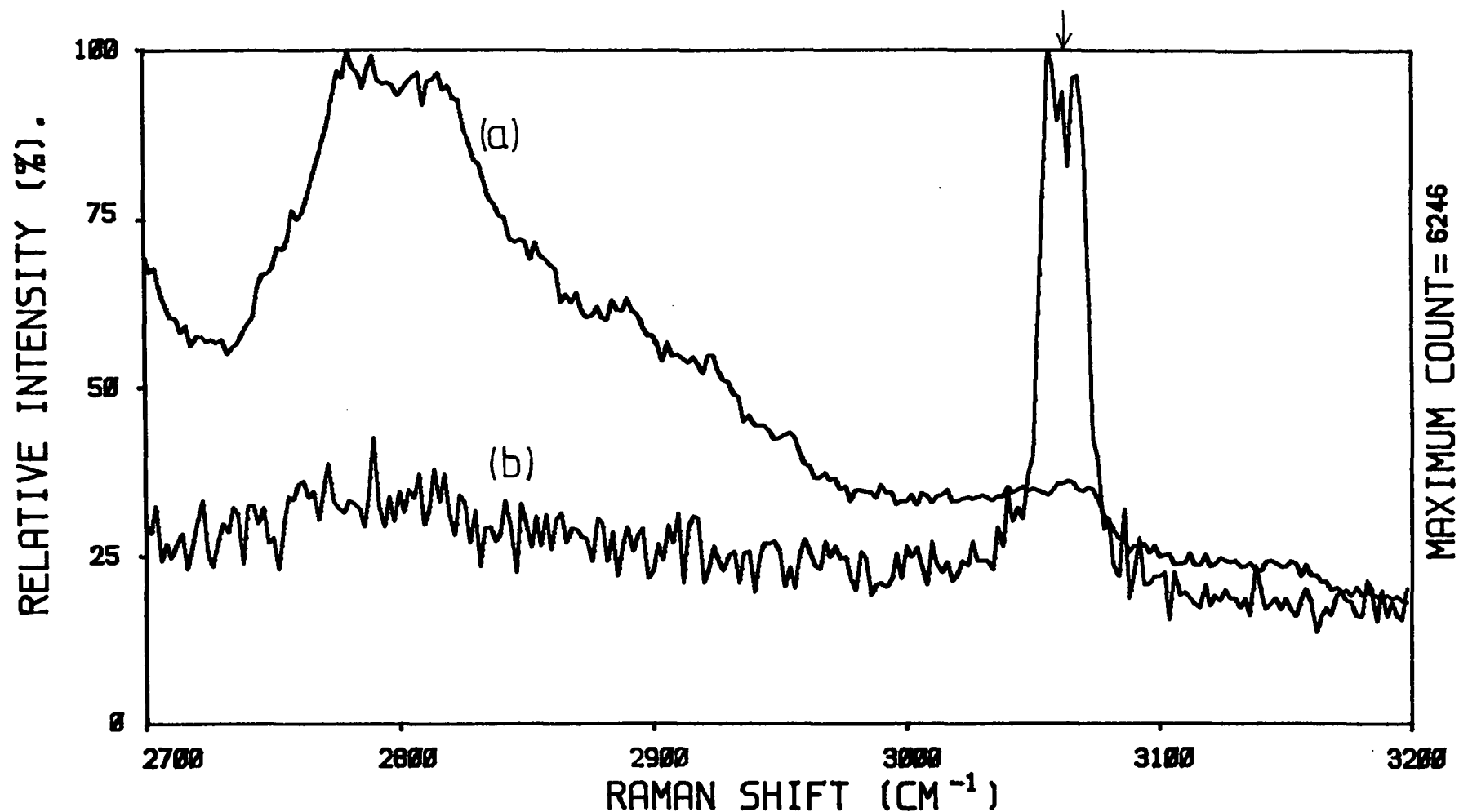
FIGURE 8.9 Expansion of \text{Al}_2\text{O}_3/\text{benzophenone} spectra. (a) = ungated, (b) = gated spectrum. Both spectra are normalised to same scale for ease of comparison. Raman band ( \dagger ) is greatly enhanced in gated spectrum.
