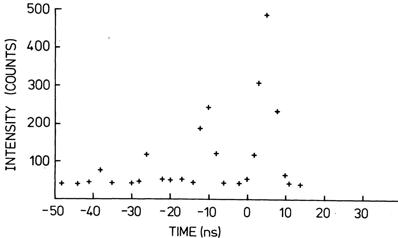
FIGURE 7.10 Intensity of 992 cm -1 band of benzene as a function of gate position. The multiple opening of the gate (see text) is clearly illustrated.
