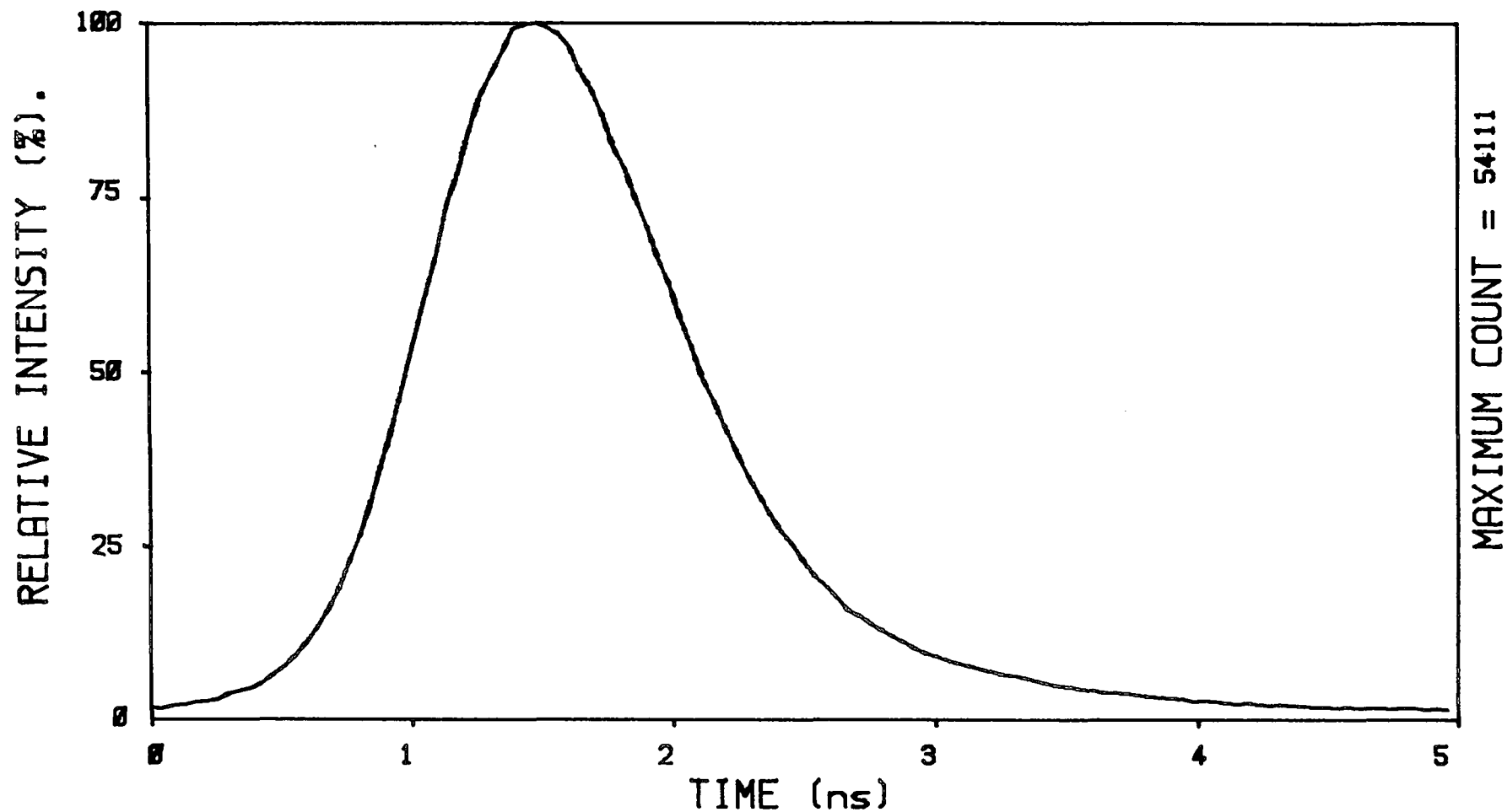
FIGURE 8.15 IRF of system with rewired PMT voltage divider. Anode pulses processed by amplifier/discriminator incorporated in IDA, i.e. a simple leading edge discriminator. FWHM = 1.1 ns.
