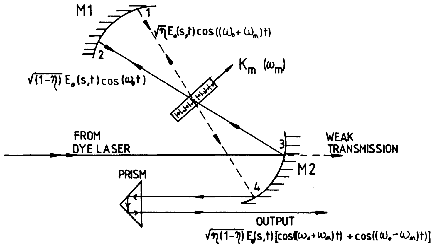
FIGURE 5.9 Schematic of Bragg cell operation. See text for details. Note the weak transmission of mode-locked pulses through mirror M2 (Section 5.3.3.1).
