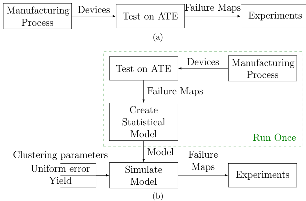
Figure 3.1: Experiments with Real and Modelled Failure Maps.
