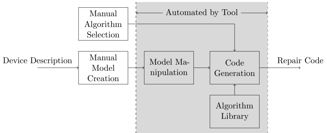
Figure 1.4: Proposed System Overview: The user must first describe the device using the graphical editor and select the repair algorithm required. The tool then manipulates the model and draws upon a library of repair algorithms to generate repair code.
