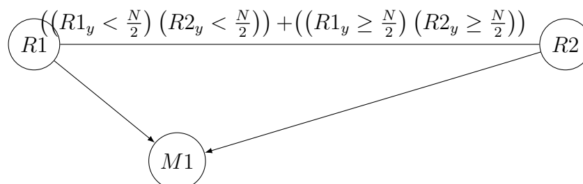
Figure 5.8: Redundant blocks R1 and R2 can both repair M1, but the use of either constrains the use of the other to the same half of M1 (this constraint is commonly caused by sharing the most significant fusebox bit).
