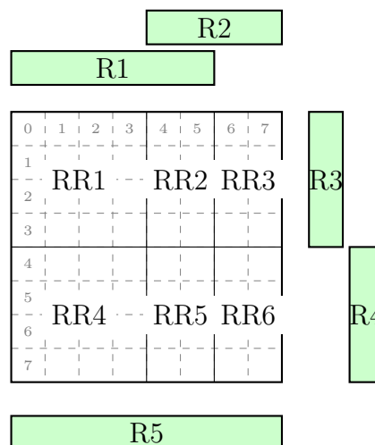
Figure 7.5: Repair regions in a simple device. Repair regions, marked RR_n , are derived from the redundant elements, marked R_n .
