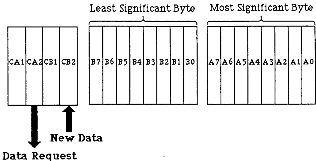
Fig 5.2.5 Data arrangement required from receiver hardware.
