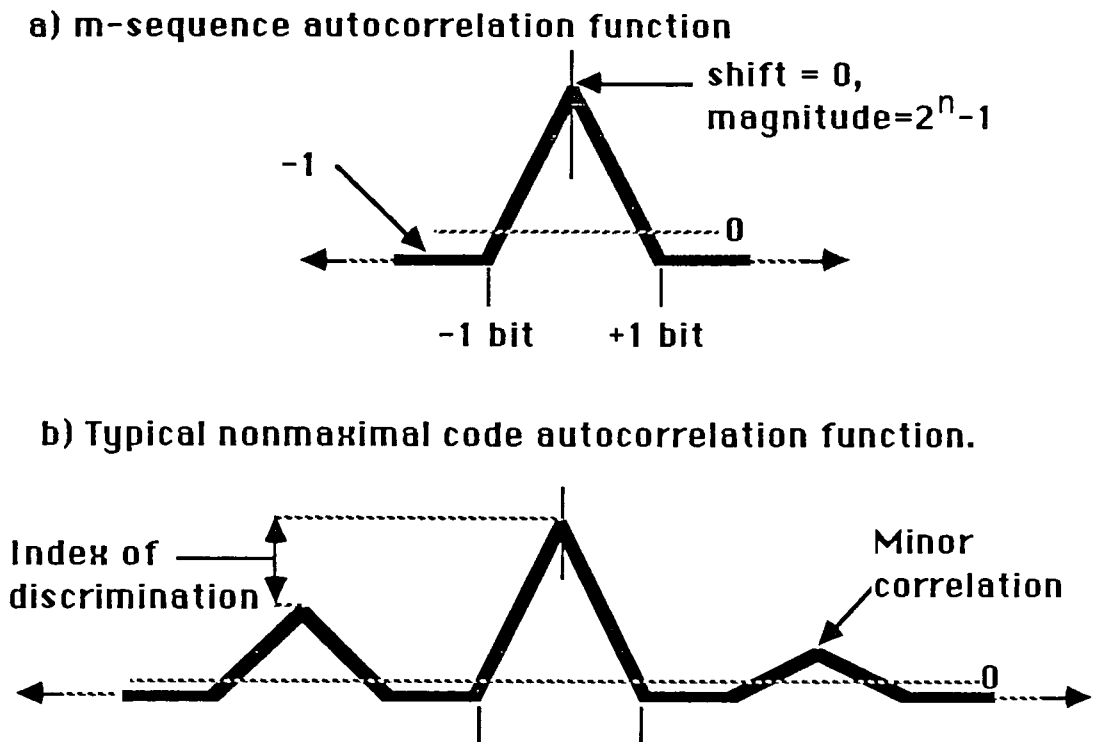
Fig 4.1.5 Autocorrelation of Maximal and Non-maximal sequences.
