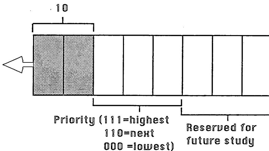
Fig b.3 Management data frame.
