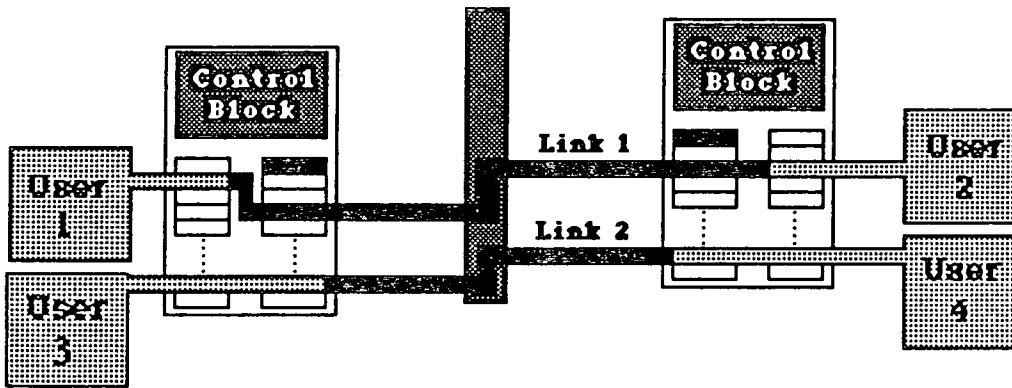
Fig 6.4.2 Possible Red-black separation points.
