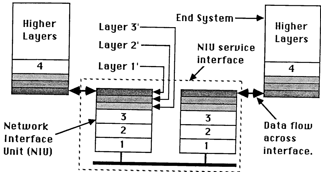
Fig 3.4.2 Interfacing to a Network via NIUs.
