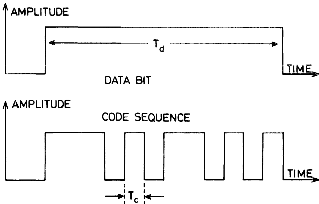
FIGURE (2.1a): Direct Sequence SS Modulation
