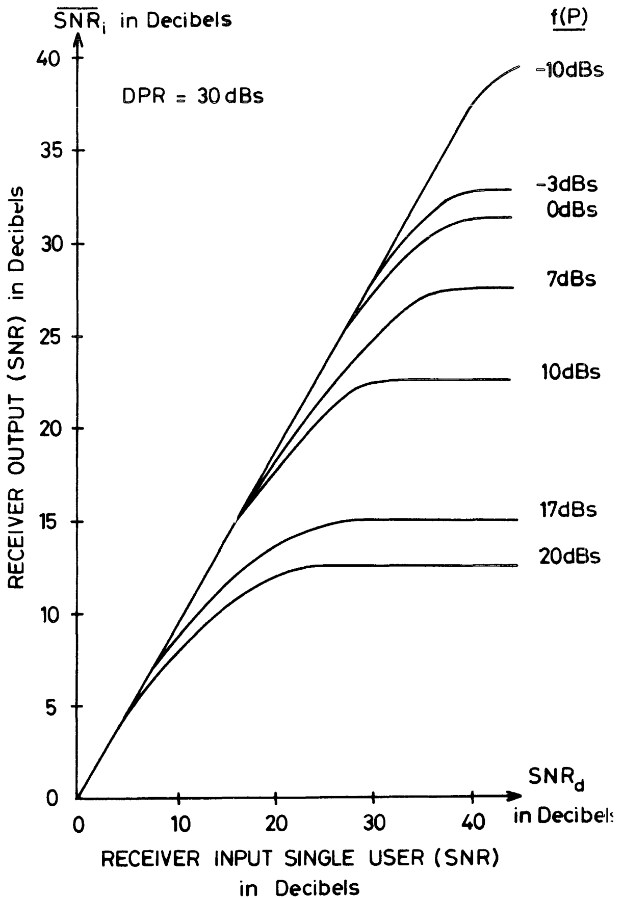
FIGURE (6.7): \overline{\text{SNR}}_i vs \text{SNR}_d for a DPR of 30 Decibels
