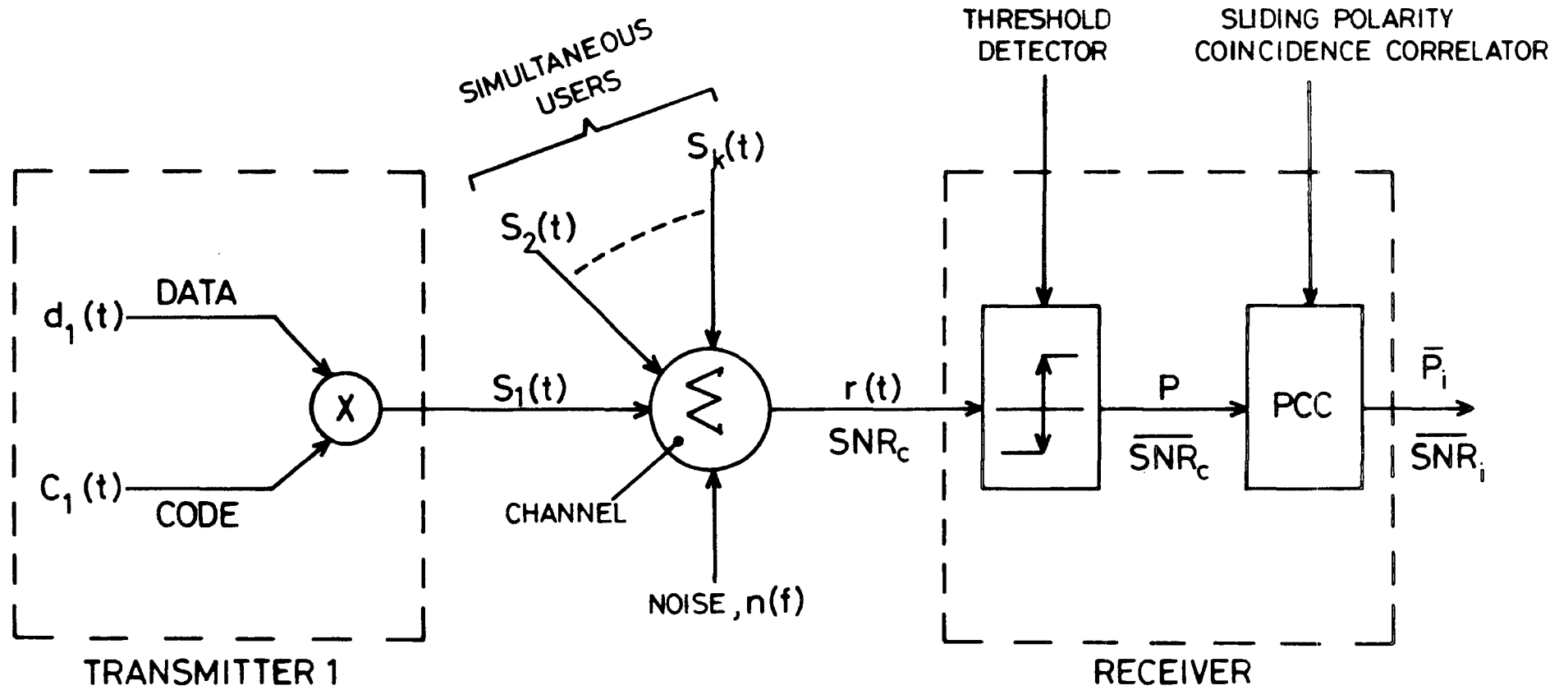
FIGURE (6.5): Schematic of an SS-LAN Communicating Pair
