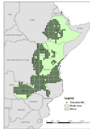
Figure 3.7: The geographical distribution of optimal and tolerable coffee growing locations, based on decadal mean annual temperatures and total annual precipitation between 1961 and 2002.
