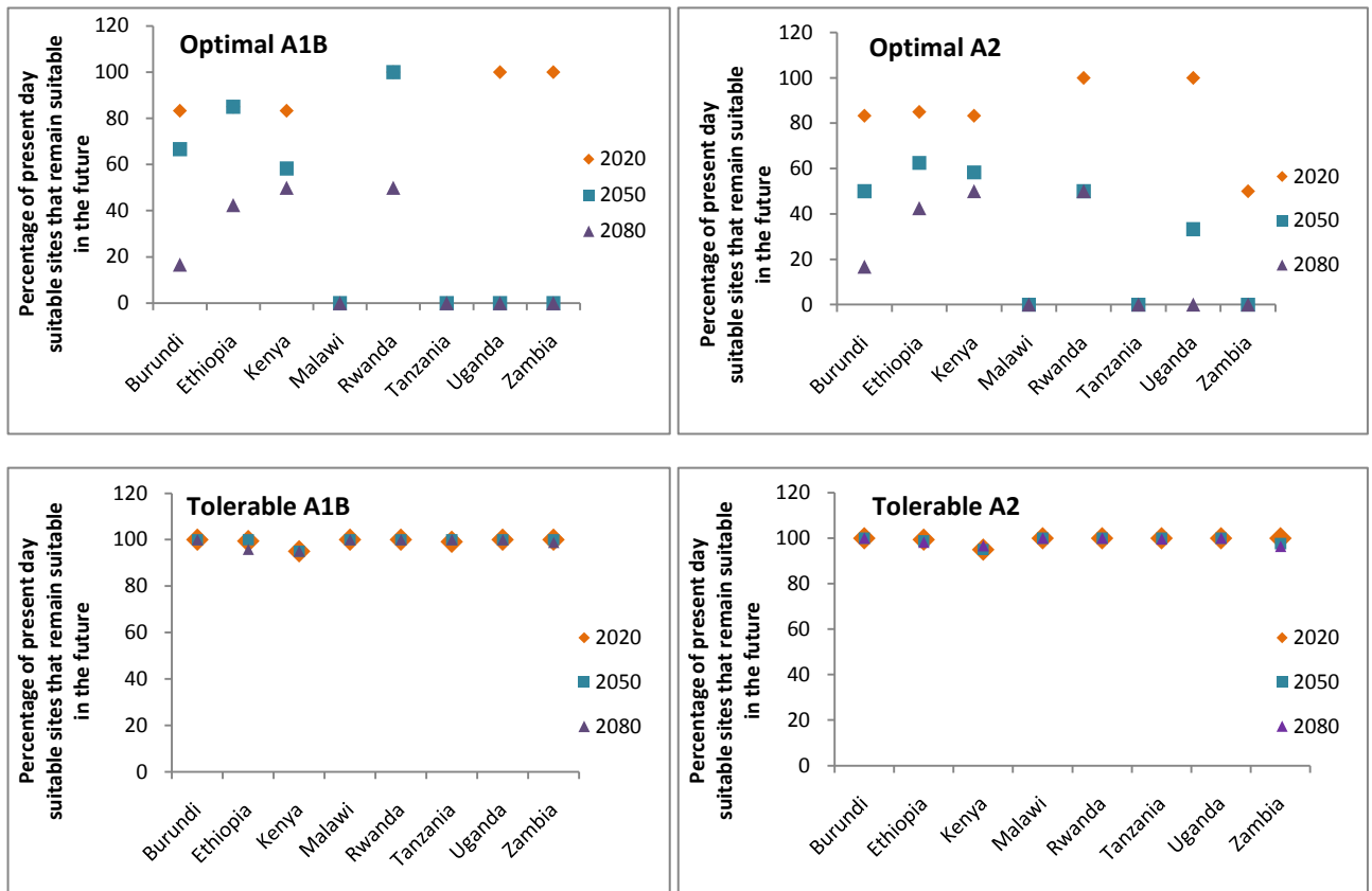
Figure 5.6: The percentage of current suitable C. arabica growing locations by country, which remain suitable in the future, calculated from the combined results of three GCMs.
