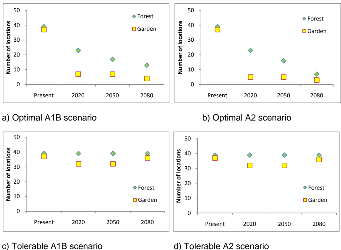
Figure 5.8: The number of forest and garden coffee growing locations in Ethiopia under optimal and tolerable climatic conditions through time. Climatic conditions are calculated as a mean of the output from three GCMs.
