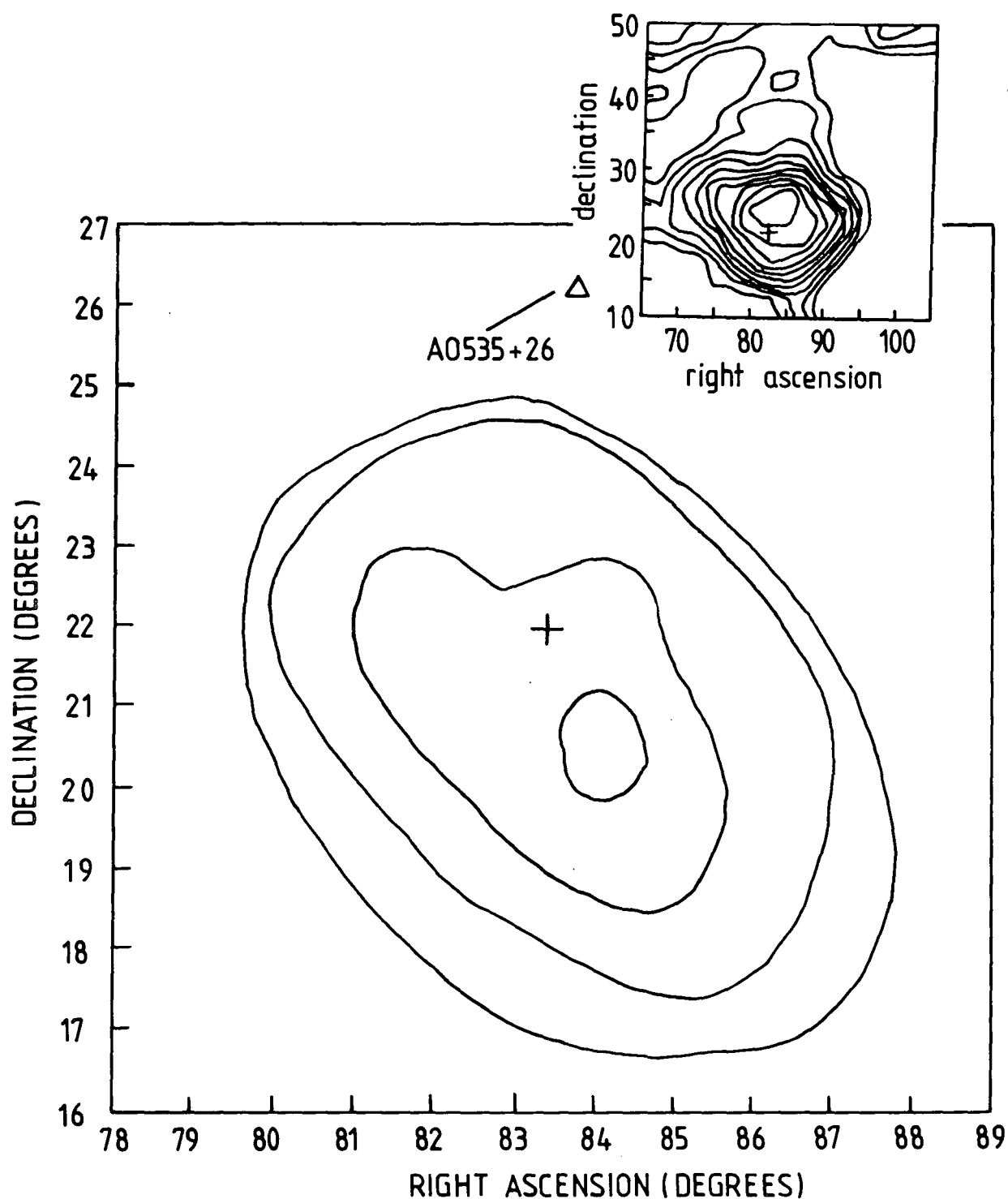
Figure 5.3 Results of a cross-correlation analysis for the field of view containing the Crab. The energy interval of accepted events is 50 to 350 keV. The contours represent positions where the correlation function has constant values at the \alpha level. The cross denotes the true position of the Crab in 1950 coordinates. From the graph the error in the orientation system is estimated to be 1.4^\circ rms. For comparison the inset shows the Crab imaged in 3-7 MeV gamma-rays (Schonfelder, 1979).
