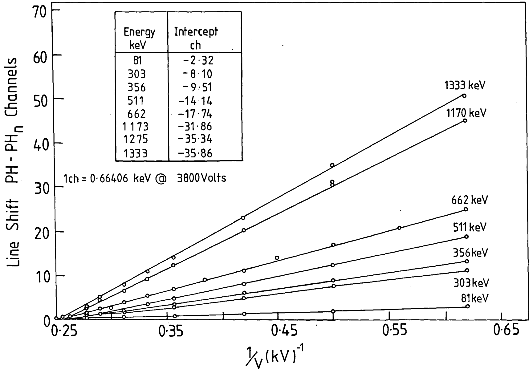
Figure B.1 Full energy peak shift as a function of detector bias.
