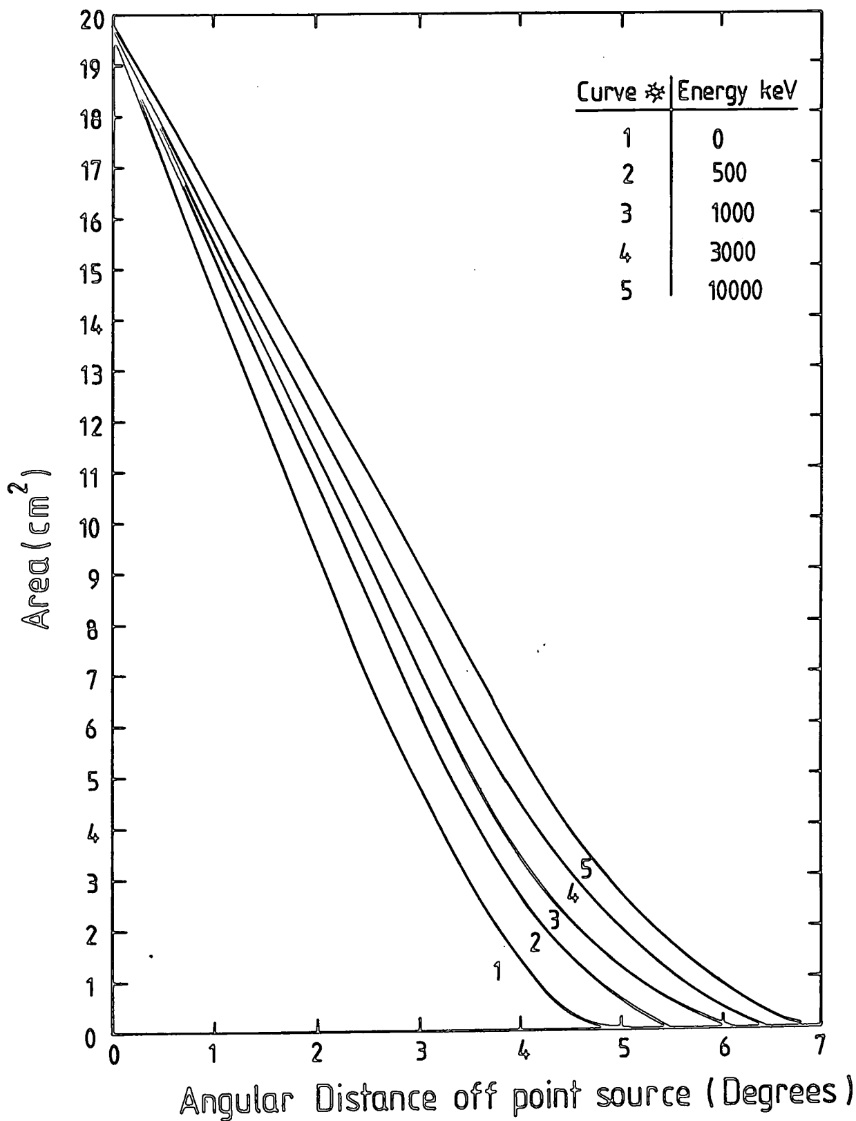
Figure 4.9 The angular response of the MK2 telescope to a distant point source.
