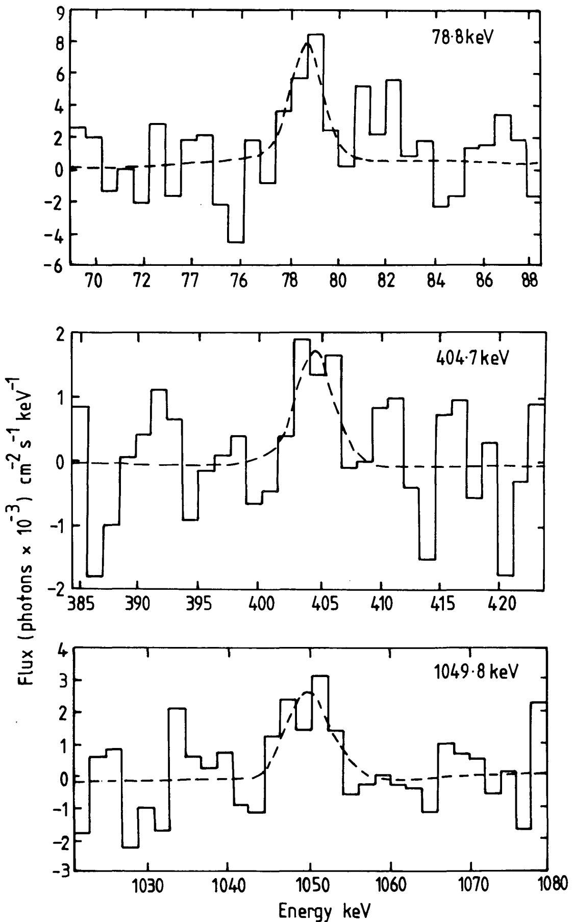
Figure 5.6 Line profiles of the three detected features after correcting to the top of the atmosphere. The dashed line on each profile is a best fit polynomial plus a Gaussian peak. The 78.8 keV line is discussed in section 5.4.4.
