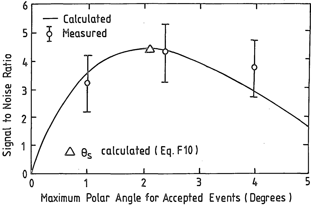
Figure F.1 The calculated and experimentally determined signal to noise ratio's as a function of the maximum polar angle for accepted events.
