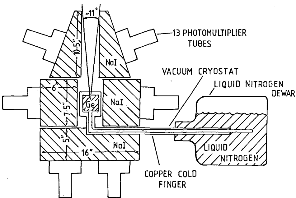
Figure 2.8 A cross sectional view of the Bell-Sandia instrument apparatus. (Leventhal et al., 1977)
