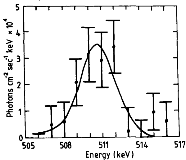
Figure 3-4 An expanded version of Fig. 3-3 in the vicinity of 511 keV. From Leventhal et al. (1978)
