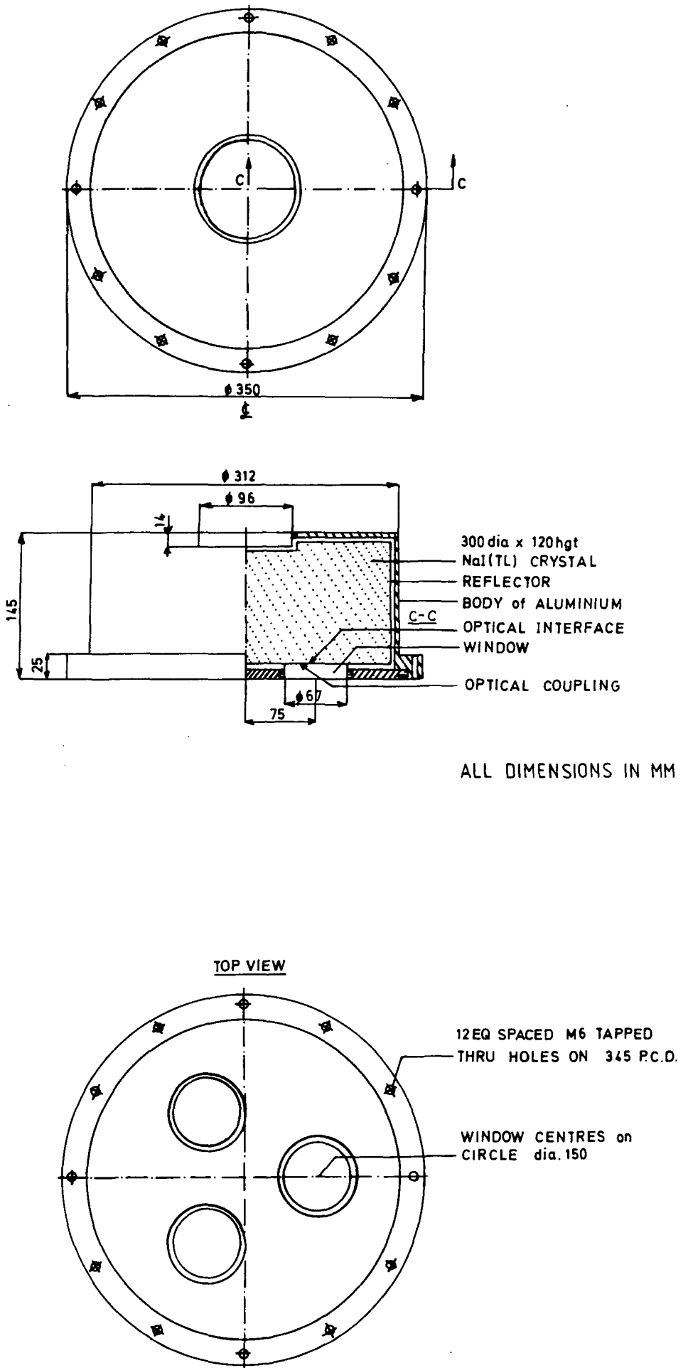
Figure 4.4 The A3 crystal assembly.
