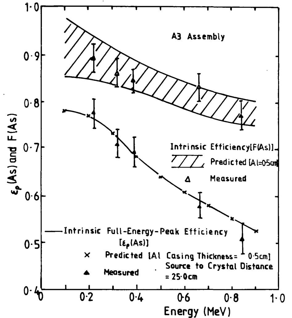
Predicted and measured values of intrinsic efficiency and intrinsic full-energy-peak efficiency for the A3 shield assembly as a function of source energy.
