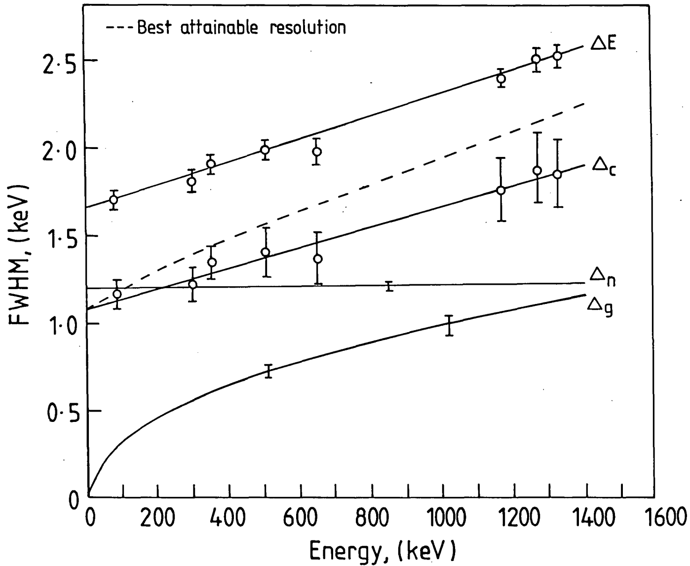
Figure B.2 The detector Energy Resolution FWHM as a function of energy at the nominal Bias. The various contributions to the FWHM are shown separately.
