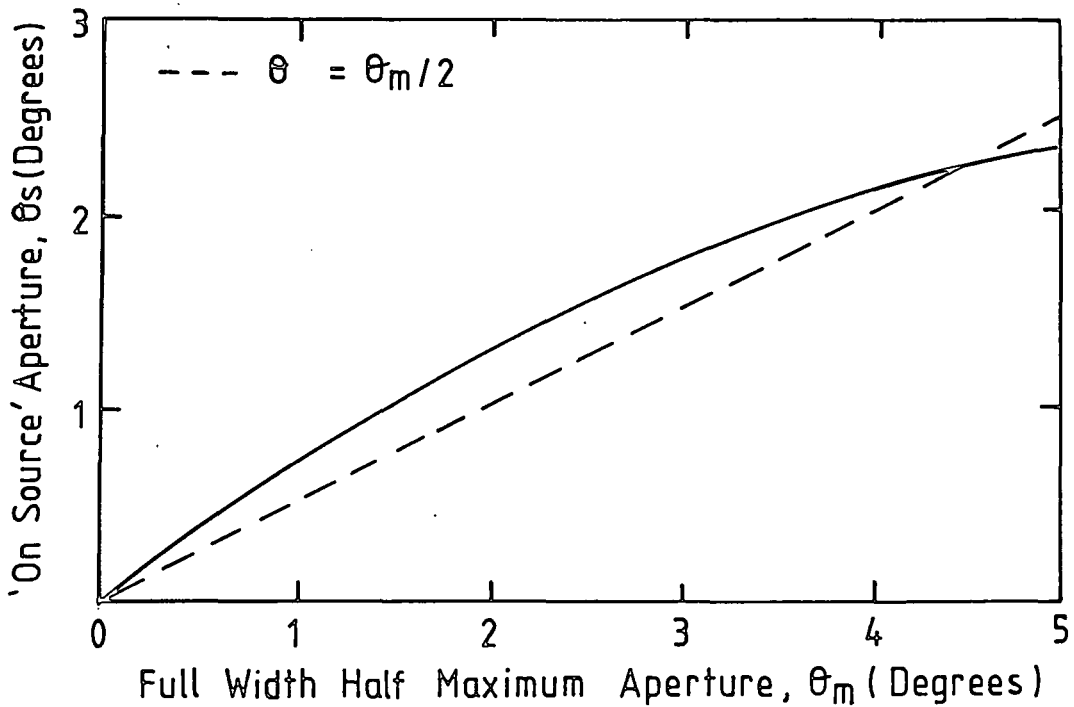
Figure F.2 The variation of the 'on source' polar angle, \theta_s , with FWHM aperture. Here \theta_s is the value of the maximum polar angle for accepted events for which the signal to noise ratio is a maximum.
