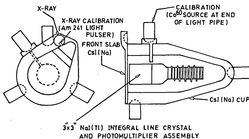
Figure 2.6 A schematic drawing of the \gamma -ray spectrometer onboard the OSO-7 satellite. (Chupp et al. 1973)
