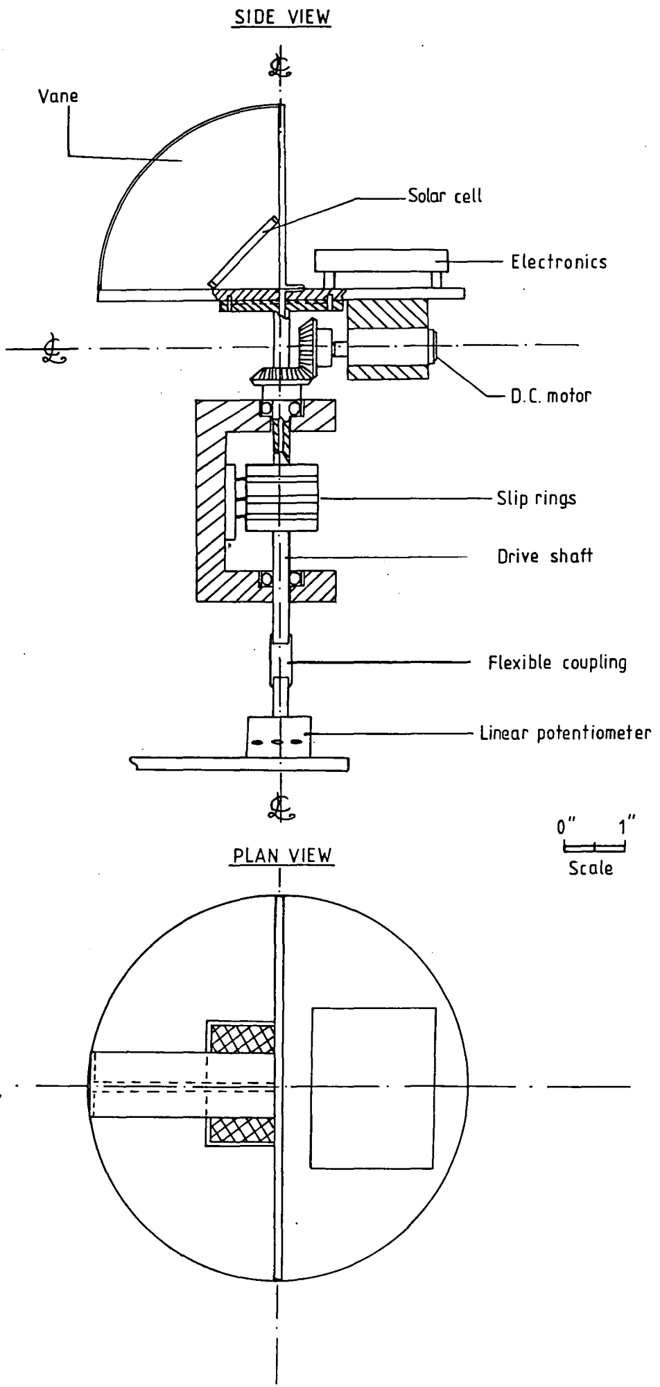
Figure A.5 The Solar Sensor
