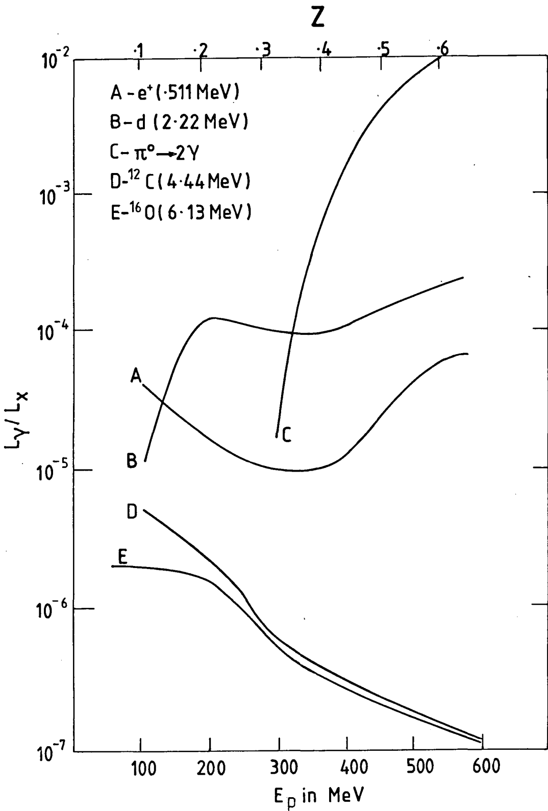
Figure 1.4 Expected gamma-ray line fluxes as a function of neutron star redshift z or accreted proton energy E_p . (from Brecher, 1978)
