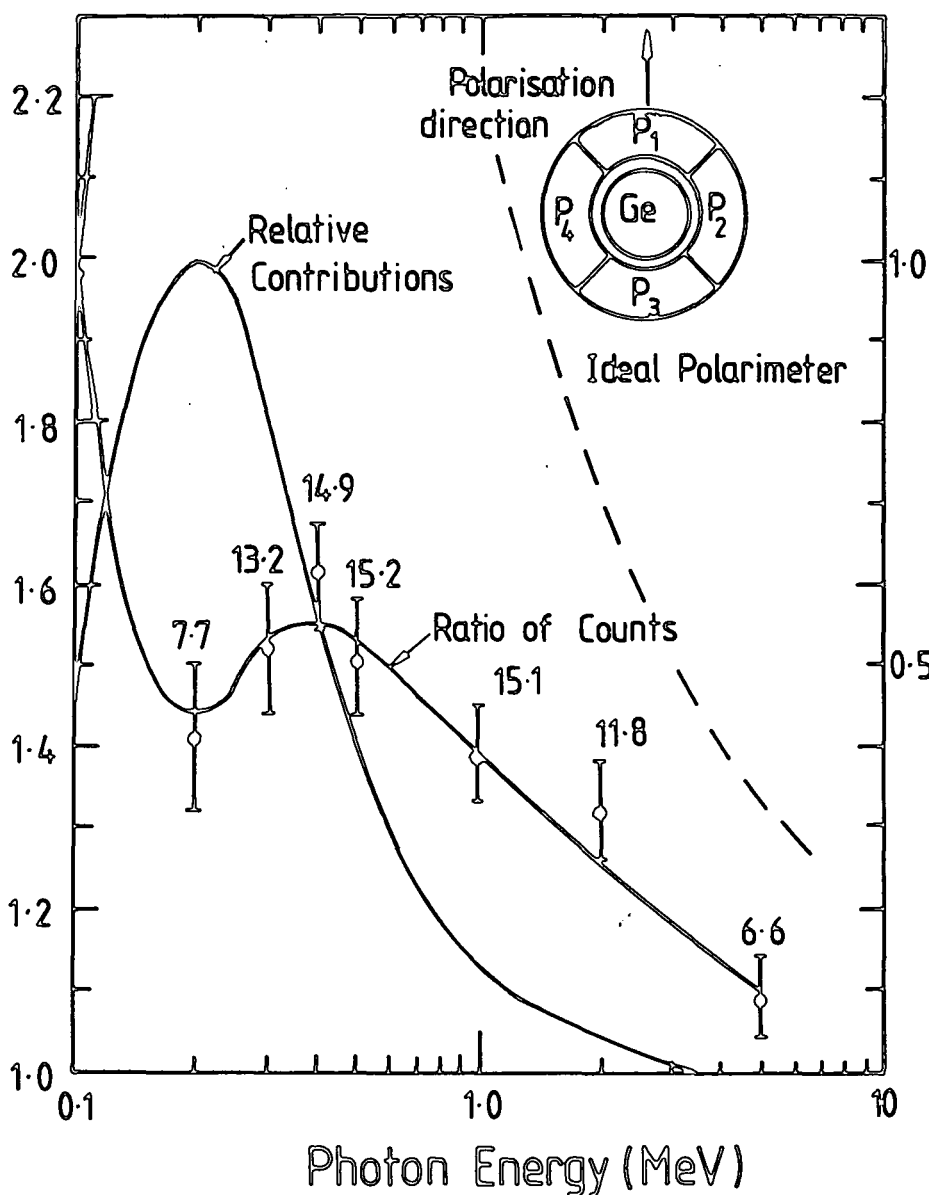
Figure 4.11 The ratio of the counting rates (P_2 + P_4)_{Ge} / (P_1 + P_3)_{Ge} as a function of energy for a 100% polarized incident beam. For comparison the response of an ideal polarimeter is also shown (assuming point scattering and absorption). The parameter for each point is the percentage of the incident \gamma -rays which contribute to the polarisation measurement. For a typical source spectrum N_\gamma(>E) \propto E_\gamma^{-2} , the relative contributions of photons to polarisation measurements are shown as a function of energy.
