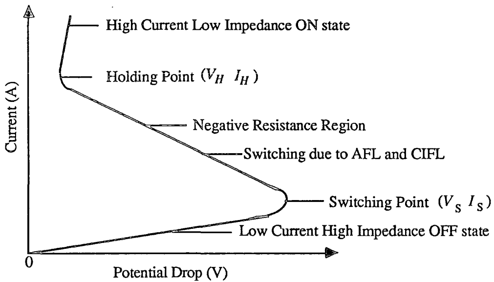
Fig 2.3: Ideal Two State Current Voltage Curve
