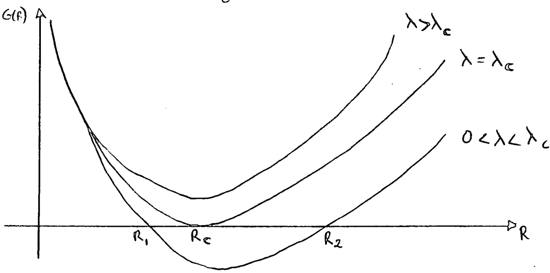
fig. 2 G(R) for \lambda > 0 , K=+1 Models.
