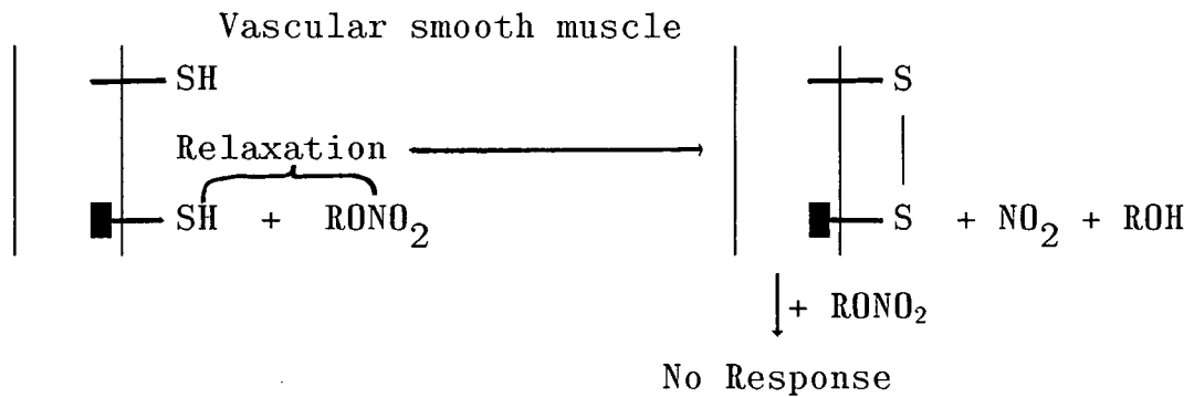
Figure 1.1 Organic nitrate receptor
