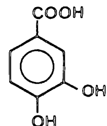
3,4 dihydroxy-benzoic acid
