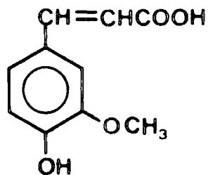
Ferulic acid
