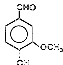
Vanillin
