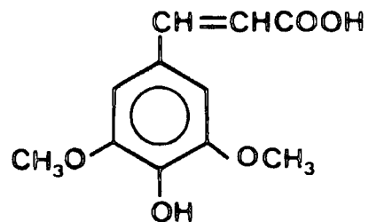
Sinapinic acid
