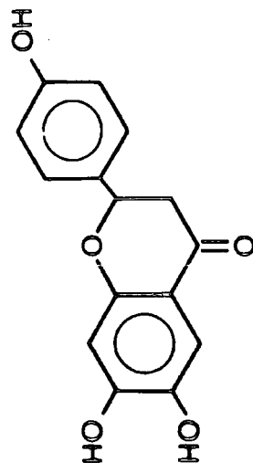
Apigenin
