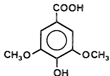
Syringic acid
