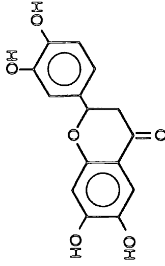
Luteolin
