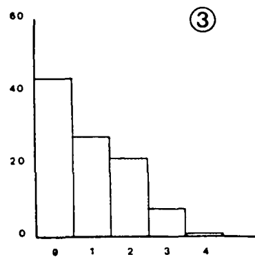
Fig. 4: A graphical representation of the frequencies of the individual areas.
