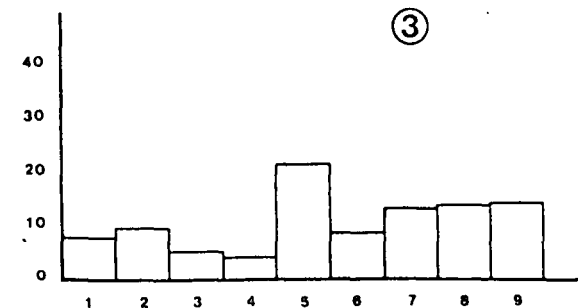
Fig. 2: A graphical representation of the frequencies of the individual areas
