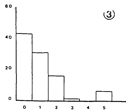
Fig. 4: A graphical representation of the frequencies of the individual areas.
