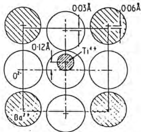
Figure 4 : The Atomic Positions in Tetragonal BaTiO 3
