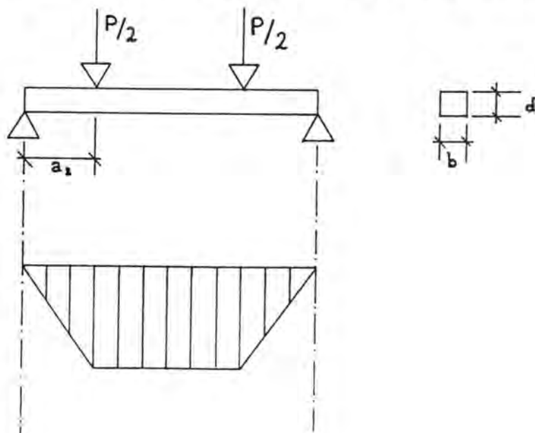
Figure 7b: Bending Moment Diagram for Four-Point Bending
