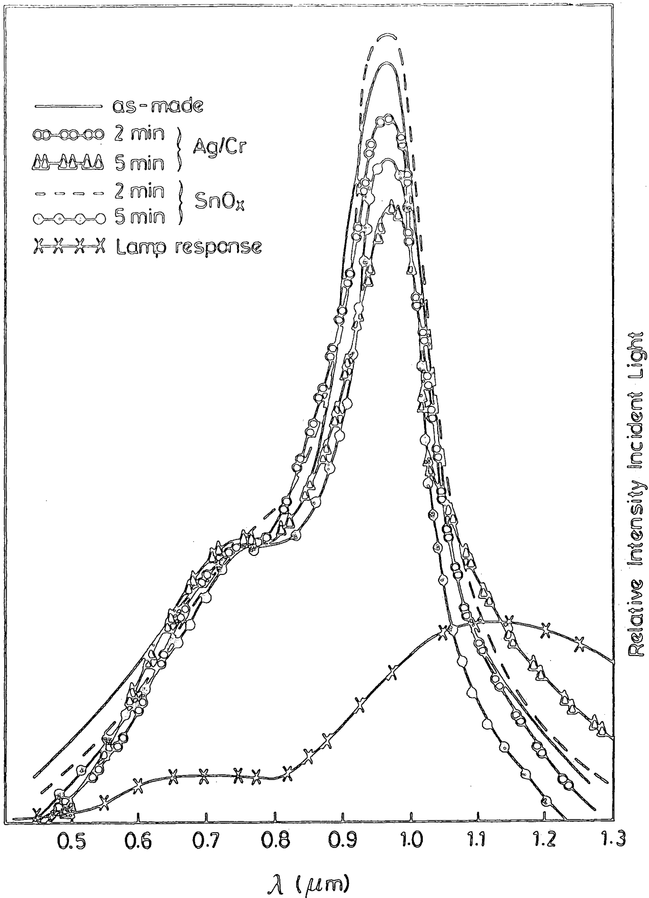
Fig 6.15 : V_{oc} spectral response (at 295 K) of two heterojunction devices fabricated on Ag/Cr and SnO x with 0.1 V electroplating bias after annealing in Argon for different periods.
