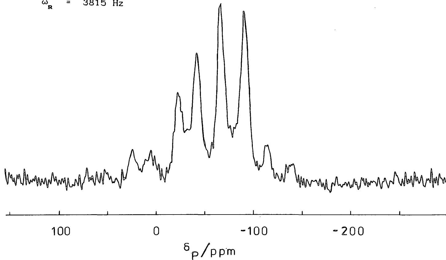
Fig (4-18) ^{31}\text{P} CP/MAS/HPPD Spectrum of complex (II).
