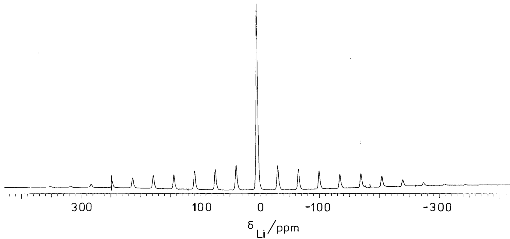
Fig (4-4c) {}^7\text{Li} SP/MAS/HPPD Spectrum of [\text{LiBH}_4\cdot\text{TMEDA}]_2 with the sample inside the new insert at 7.0463 T.
