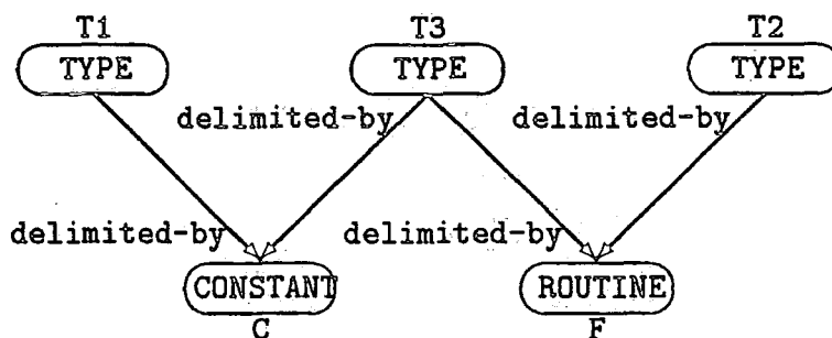
Figure 8.2: The Entity-To-Entity Interconnection Graph for Figure 8.1
