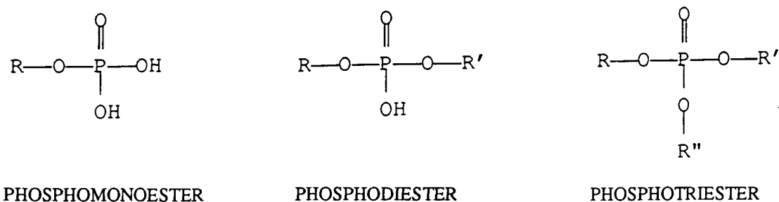
Fig. 1.1 Formulae for phosphate esters
