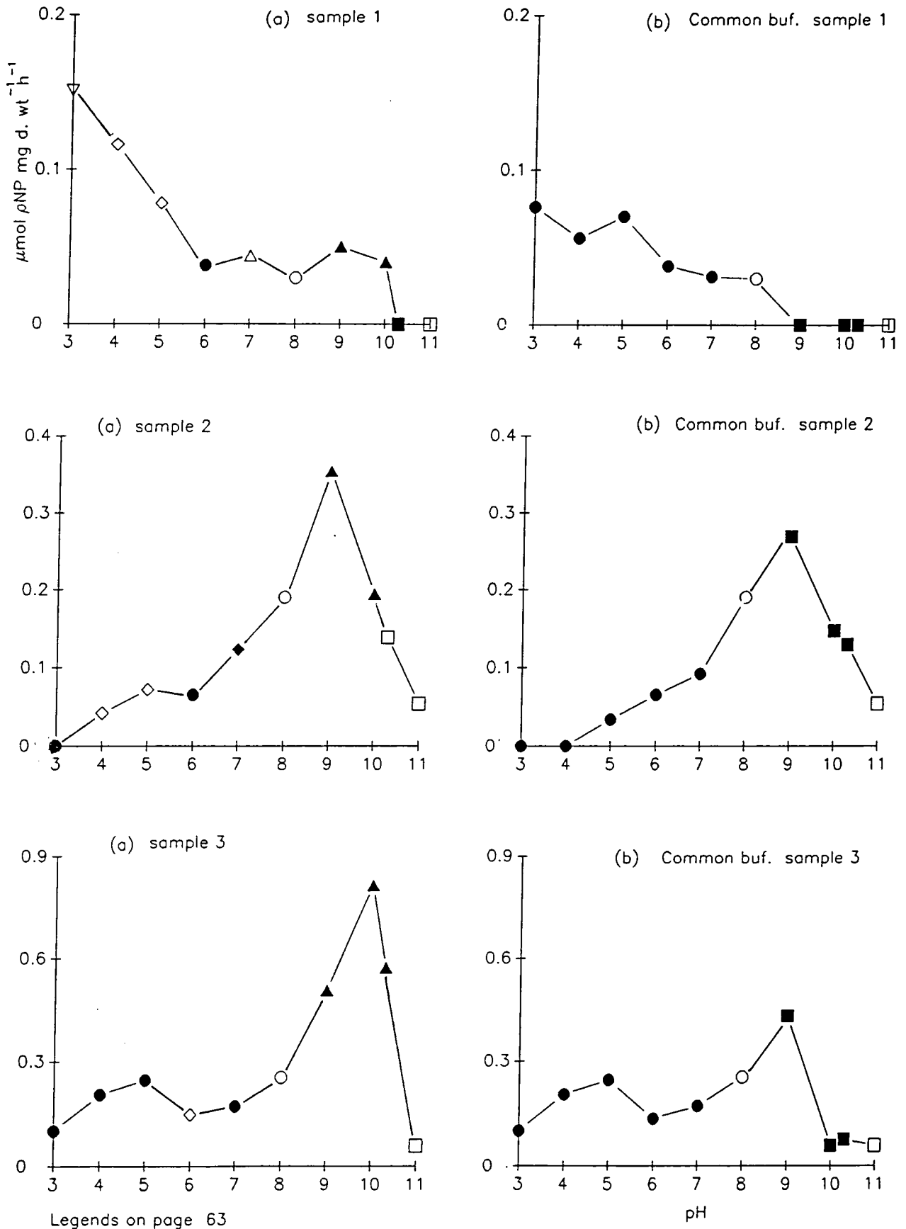
Fig. 5.5 Effect of pH on phosphatase activity of algal samples collected from 14 sites in survey B (Table 5.2). Each sample is presented twice in two ways: a, b (5.21)
