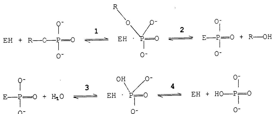
Fig. 1.2 Reaction scheme for the enzyme catalyzed hydrolysis of phosphate esters as described by McComb et al. , (1979).
