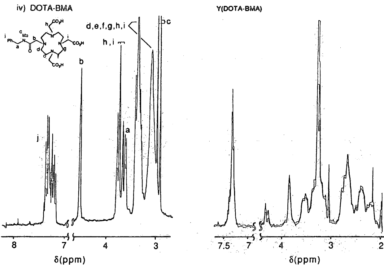
Figure 2.9: a iii) TETA and TETA in the presence of \text{Y}^{3+} ; (cont'd) iv) DOTA-BMA and \text{Y}(\text{DOTA-BMA}) .
