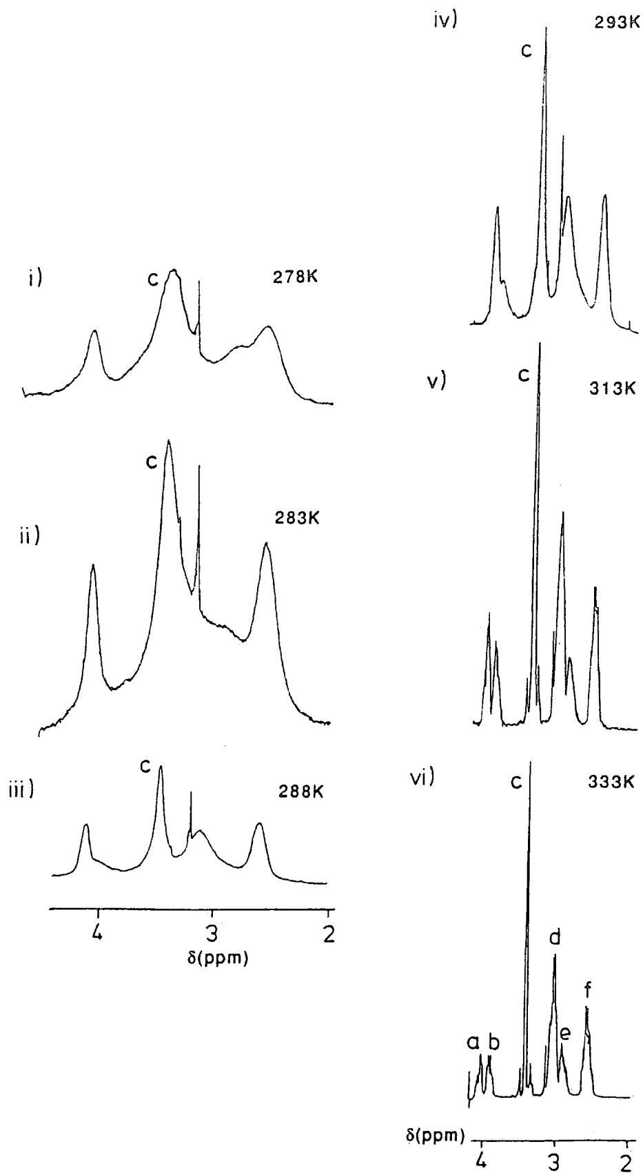
Figure 2.13: ^1\text{H} NMR spectra (250 MHz) of Y(ODOTRA) at various temperatures in \text{D}_2\text{O} (pD 5.0).
