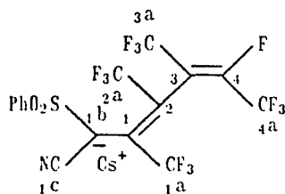
Spectra #57b
