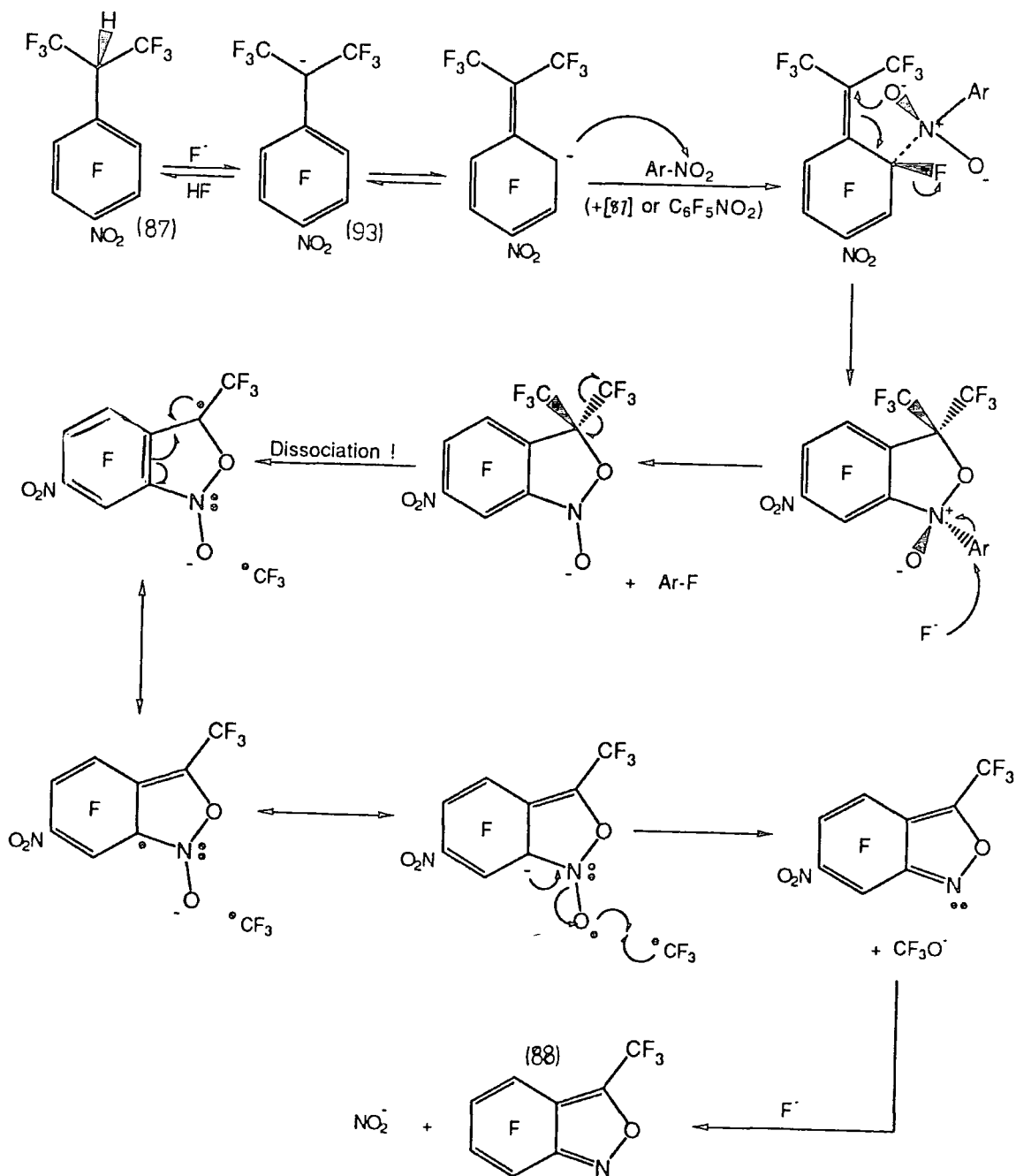
(Scheme 2.35)
