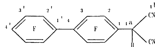
Spectra #42
