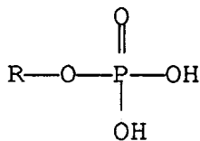
Fig. 1.1 Formulae for phosphate esters.
