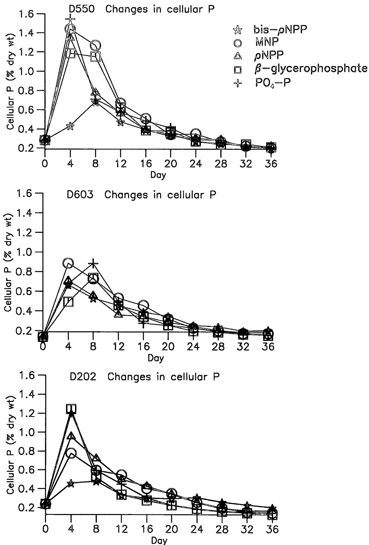
Fig. 4.1 Utilization of P-PO_4 , \beta -glycerophosphate, \rho NPP, MNP, bis- \rho NPP by Calothrix 202, 550 and 603. Cultures were grown at 32^\circ\text{C} and 100 \mu\text{mol photon m}^{-2} \text{s}^{-1} .
