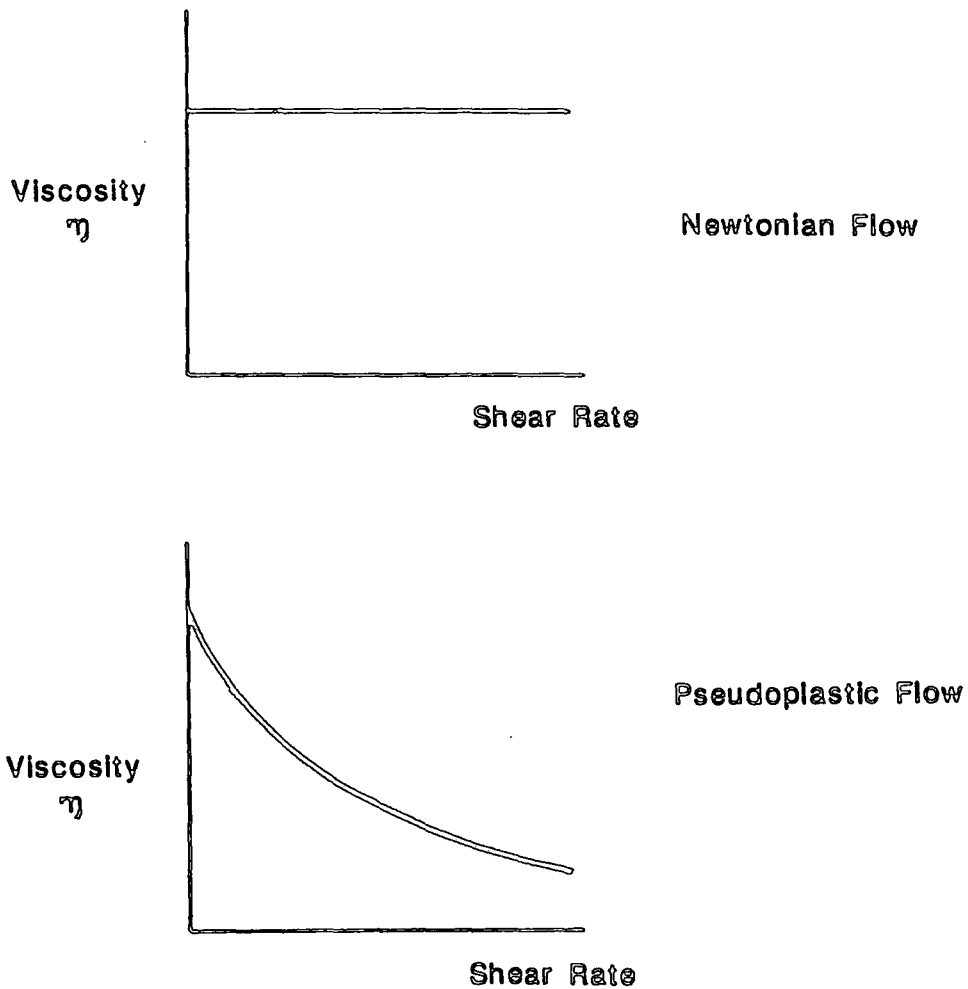
FIGURE 3.9 A comparison of Newtonian and non-Newtonian flow characteristics
