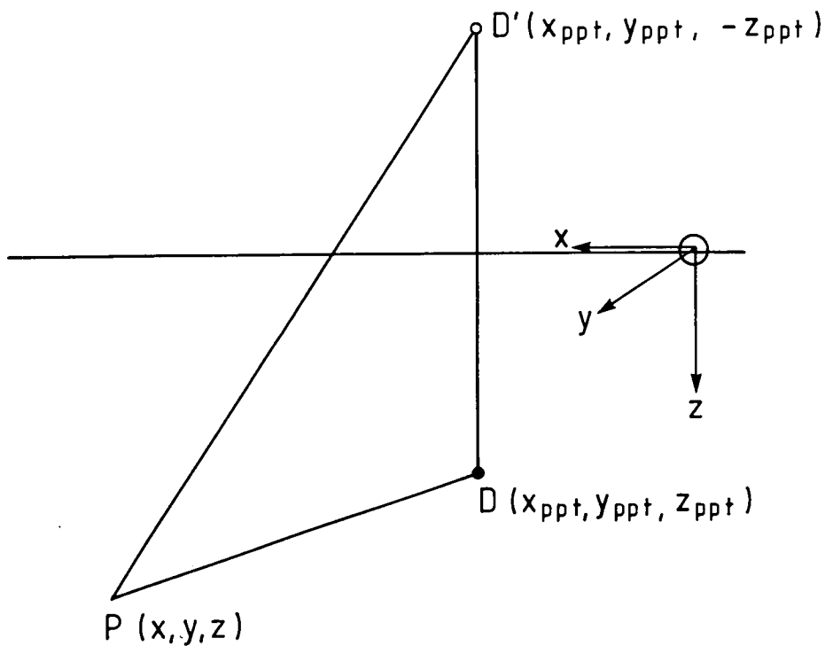
Fig. 4.15: Positions of precipitate and image precipitate.
