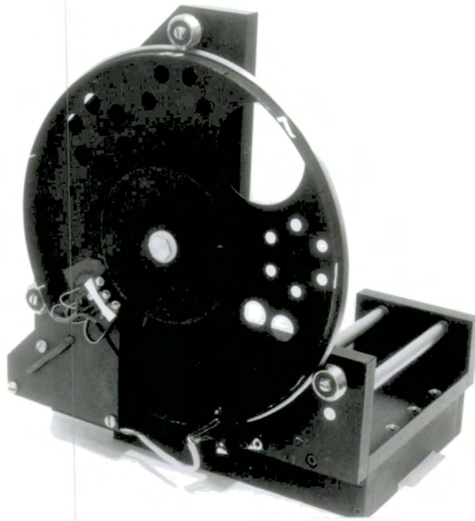
Figure 4.3: Aperture wheel assembly.
