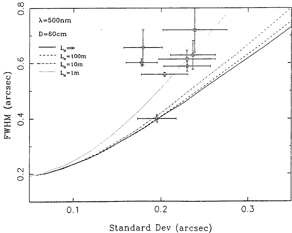
Figure 5.5: Plot of the full width half maximum of the long exposure images versus the standard deviation of image centroid motion. Also shown is the theoretical relationship expected for various values of the outer scale of turbulence L_0 .
