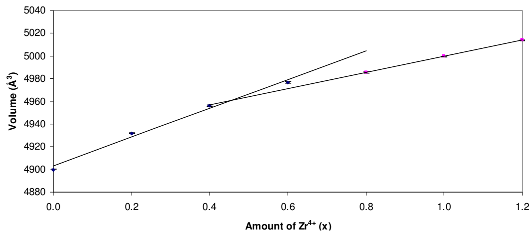
Figure 4.16: Variation of cell volume of \text{Bi}_2\text{Sn}_{2-x}\text{Zr}_x\text{O}_7 (synthesised via the conventional solid state route) with increasing zirconium content.
