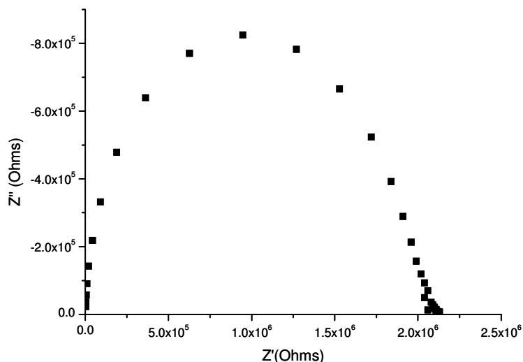
Figure 4.20: Complex impedance plot of \text{Bi}_2\text{Sn}_2\text{O}_7 at 470 \text{ }^\circ\text{C} .
