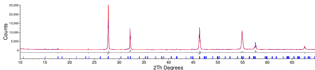
Figure 7.11: d9_04599: Rietveld fit of \text{Bi}_{18.9}\text{Sr}_{0.1}\text{V}_2\text{O}_{33.45} . R_{\text{wp}} = 7.914\% .
