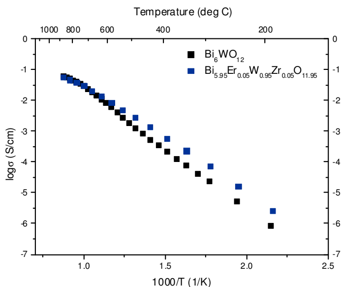
Figure 6.34: Arrhenius plot for members of the \text{Bi}_{6-x}\text{Er}_x\text{W}_{1-y}\text{Zr}_y\text{O}_{12-y} series.
