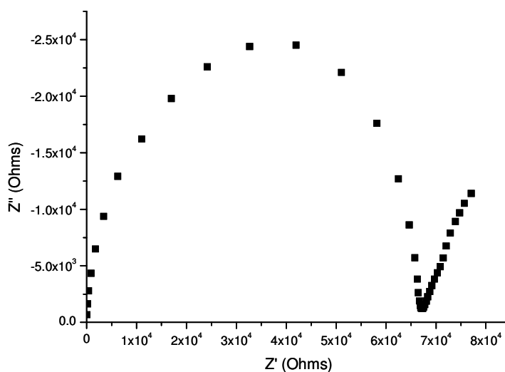
Figure 6.22: Impedance plot for \text{Bi}_6\text{W}_{0.95}\text{Nb}_{0.05}\text{O}_{11.975} at 290\text{ }^\circ\text{C} .
