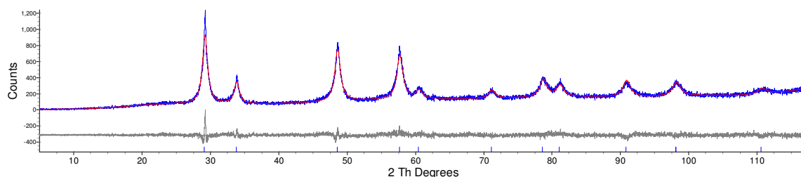
Figure 5.4: d5_07882: Fluorite type \text{Nd}_2\text{Zr}_2\text{O}_7 after annealing for 309 hours at 800 °C. Rietveld refinement for a fluorite structure. R_{wp} = 9.389\% , a = 5.3014(4) Å.
