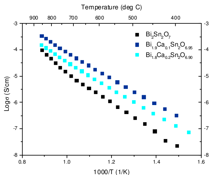
Figure 4.27: Variation of conductivity with temperature for the \text{Bi}_{2-x}\text{Ca}_x\text{Sn}_2\text{O}_{7-x/2} system.
