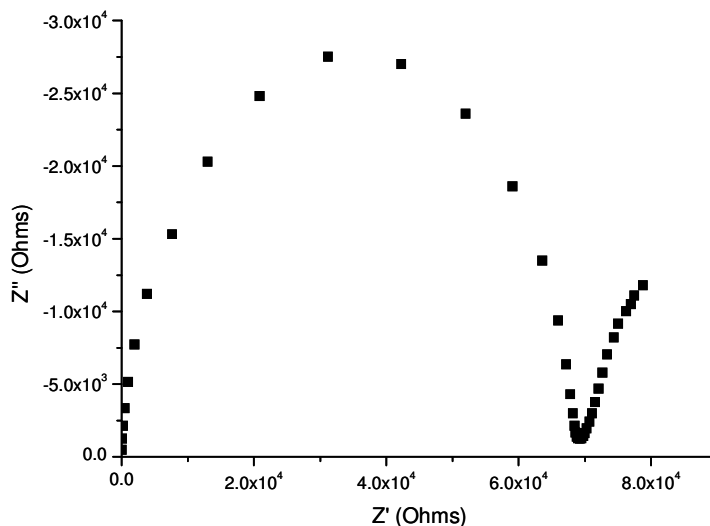
Figure 6.26: Complex impedance plot for \text{Bi}_6\text{W}_{0.95}\text{Zr}_{0.05}\text{O}_{11.95} at 192 °C.
