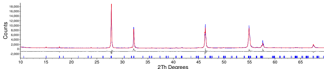
Figure 7.6: d9_04445: Rietveld fit for \text{Bi}_{18.9}\text{Ca}_{0.1}\text{V}_2\text{O}_{33.45} , R_{\text{wp}} = 8.387\% .
