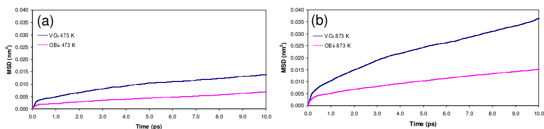
Figure 7.3: MSDs for all oxygens in either VO_4 units or OBi_4 units at (a) 473 K and (b) 873 K.
