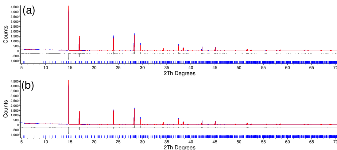
Figure 6.1: Fit to \text{Bi}_6\text{WO}_{12} synchrotron PXRD data using (a) Ling's 2010 model. R_{\text{wp}} = 6.944\% . (b) Nespolo's model. R_{\text{wp}} = 6.855\% .
