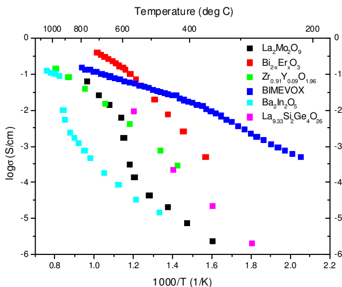
Figure 1.4: Oxide ion conductivity of some selected compounds. \text{Ba}_2\text{In}_2\text{O}_5 is a brownmillerite phase, BIMEVOX is the \text{Bi}_2\text{V}_{0.9}\text{Cu}_{0.1}\text{O}_{5.35} Aurivillius phase, \text{Y}_{0.09}\text{Zr}_{0.91}\text{O}_{1.96} has the fluorite structure, as does \text{Bi}_{2-x}\text{Er}_x\text{O}_3 , whilst \text{La}_2\text{Mo}_2\text{O}_9 is the parent member of the LAMOXY family. \text{La}_{9.33}\text{Si}_2\text{Ge}_4\text{O}_{26} is an example of an apatite oxide ion conductor. 20-23
