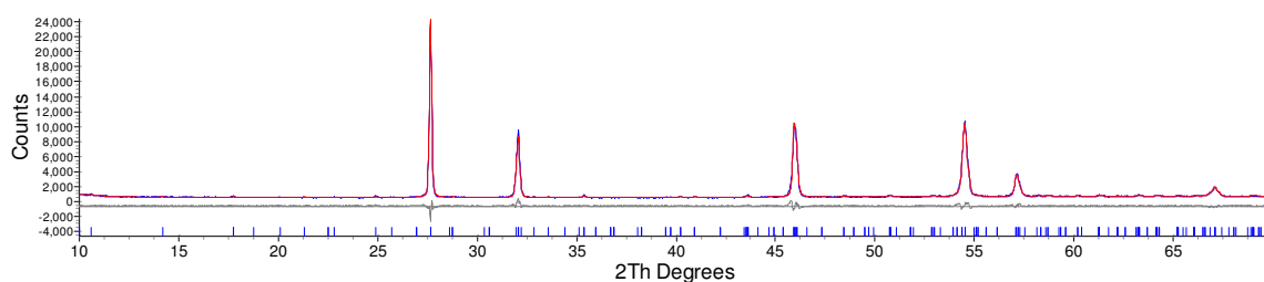
Figure 6.28: d9_03885: Rietveld refinement for \text{Bi}_{5.6}\text{Er}_{0.4}\text{WO}_{12} . R_{\text{wp}} = 6.006\%
