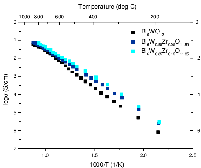
Figure 6.27: Arrhenius plots for the \text{Bi}_6\text{W}_{1-x}\text{Zr}_x\text{O}_{12-x} system.
