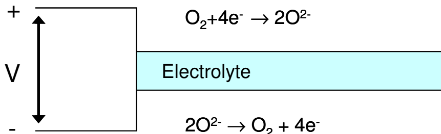
Figure 1.7: Diagram of an oxygen pump. 20
