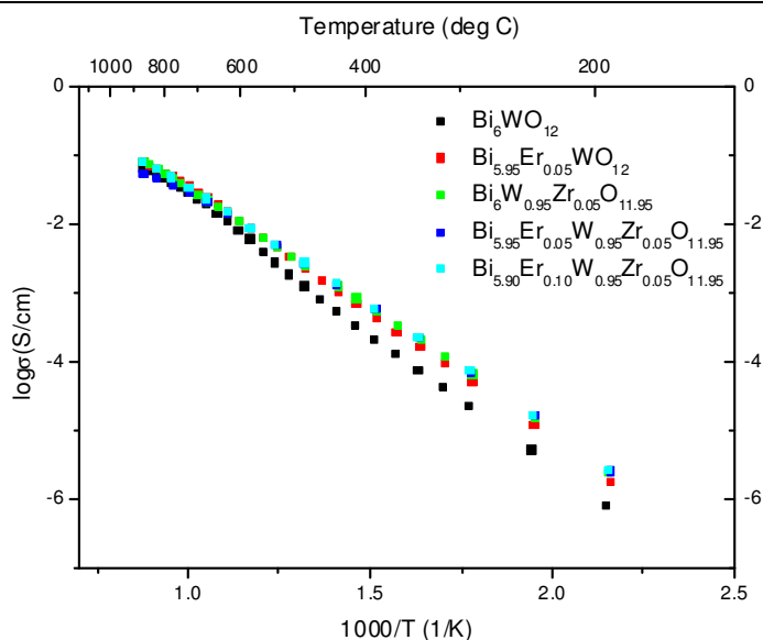
Figure 6.38: Comparison of conductivities achieved with different dopants in \text{Bi}_6\text{WO}_{12} related phases.
