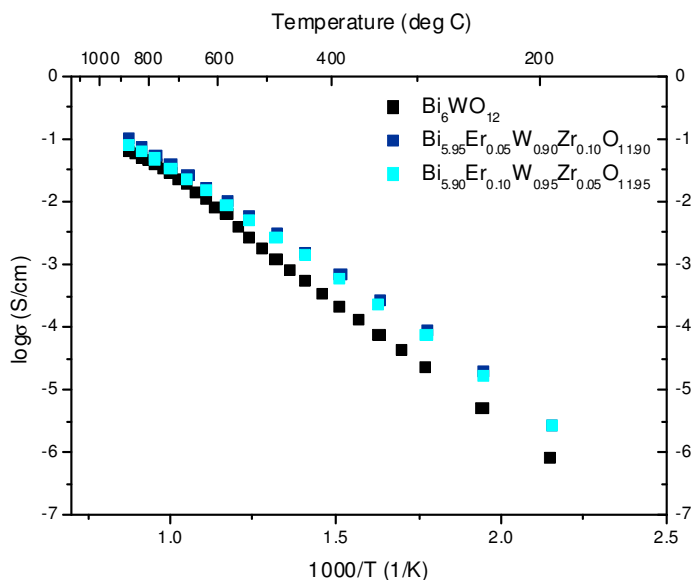
Figure 6.37: Arrhenius plots of conductivity for \text{Bi}_{6-x}\text{Er}_x\text{W}_{1-y}\text{Zr}_y\text{O}_{12-y} where x \neq y
