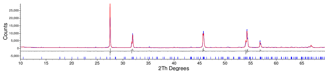
Figure 6.18: d9_03821: Rietveld fit for \text{Bi}_{5.8}\text{Ca}_{0.2}\text{WO}_{11.9} . R_{\text{wp}} = 9.740\% .
