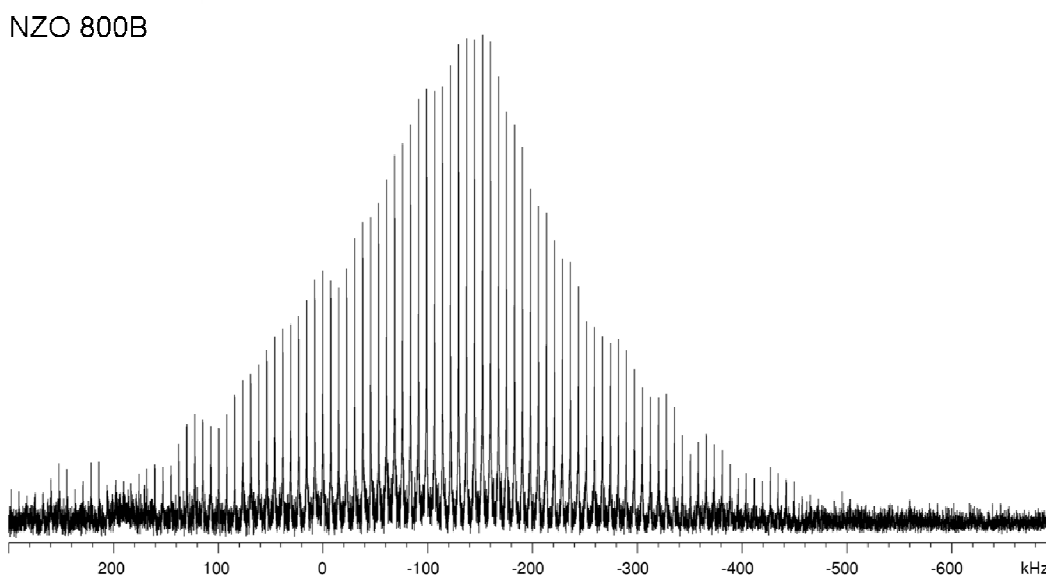
Figure 5.10: ^{91}\text{Zr} solid state NMR spectrum of NZO 800B.
