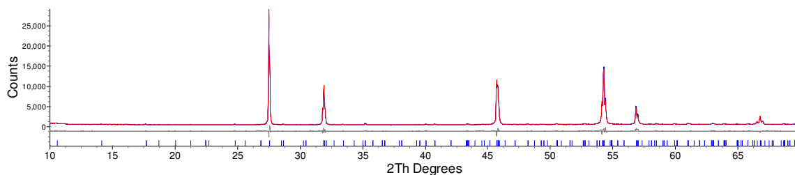
Figure 6.32: d9_04106: Rietveld fit for \text{Bi}_{5.95}\text{Er}_{0.05}\text{W}_{0.95}\text{Zr}_{0.05}\text{O}_{11.95} . R_{\text{wp}} 5.869%.
