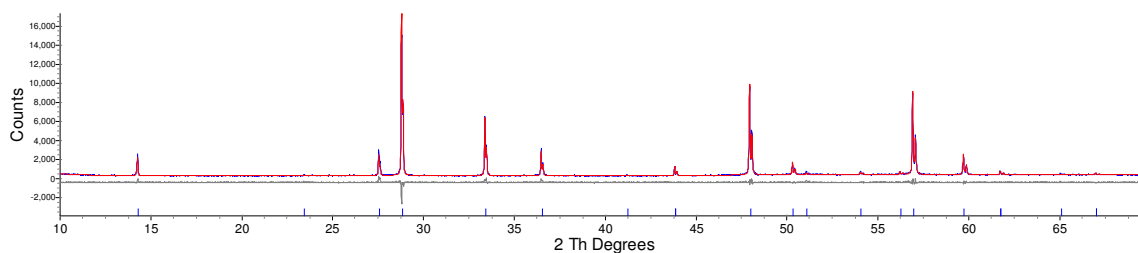
Figure 4.31: d9_03284: Rietveld refinement for \text{Bi}_2\text{Sc}_{1.05}\text{Nb}_{0.95}\text{O}_{6.95} , R_{\text{wp}} = 6.447\% .
