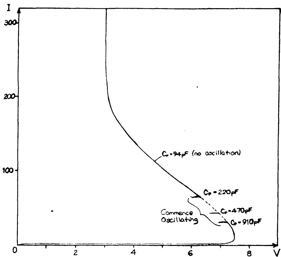
Figure 7.6; The stable NDR characteristic of a MISS device of area 1.24 \text{ mm}^2 indicating the points of onset of instability arising from the addition of a range of values of parallel capacitance, C_p
