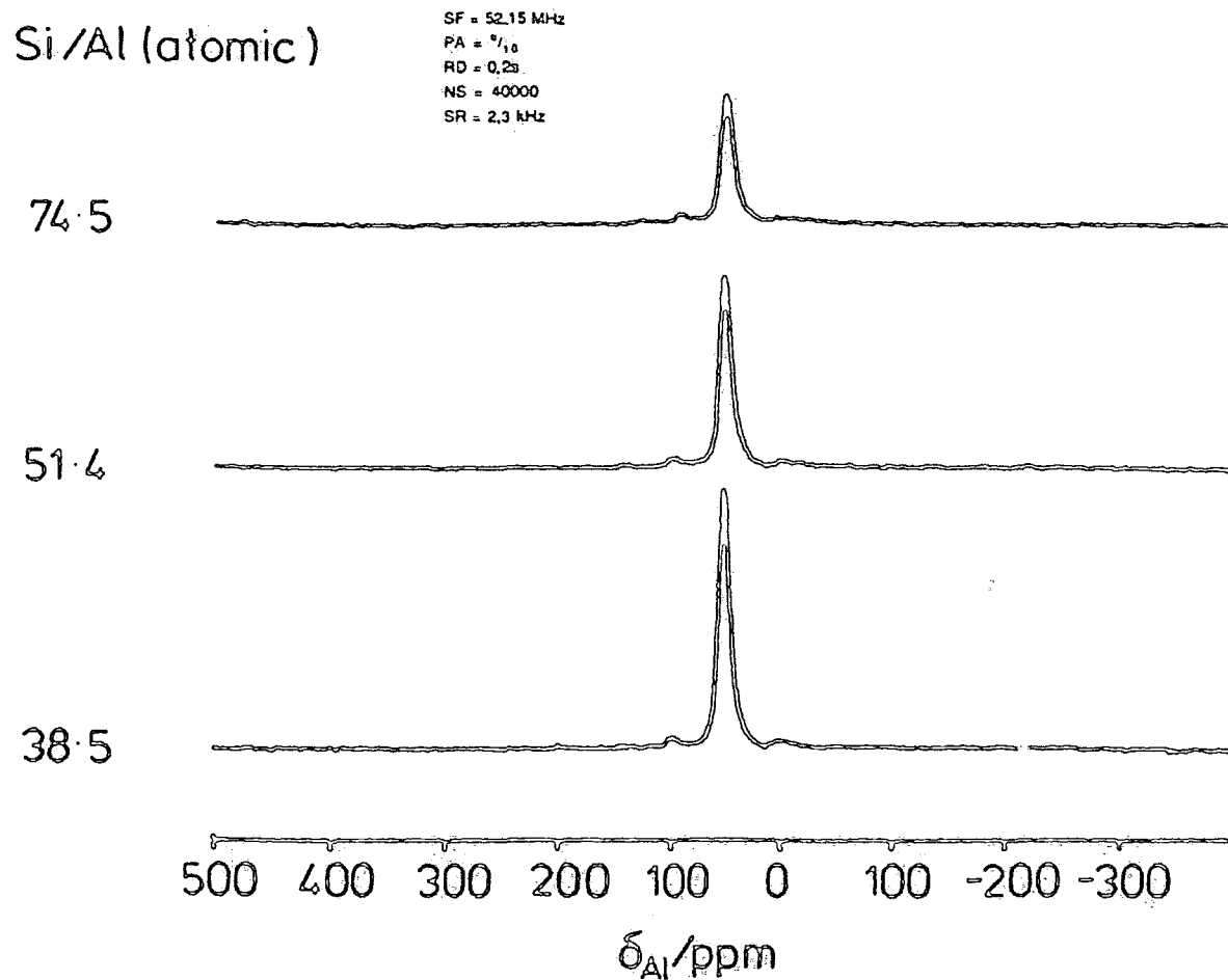
Figure 7.20: Intensity of framework four-coordinate aluminium resonance as a function of dealumination.
