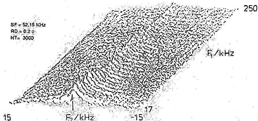
Figure 5.13(c): ^{27}\text{Al} nutation spectrum of \text{NH}_4^+\text{-ZSM-5} after heating at 503K for 3 days.
