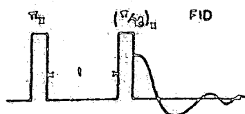
Figure S.22: Application of the conventional inversion recovery pulse sequence to NaY zeolite.
