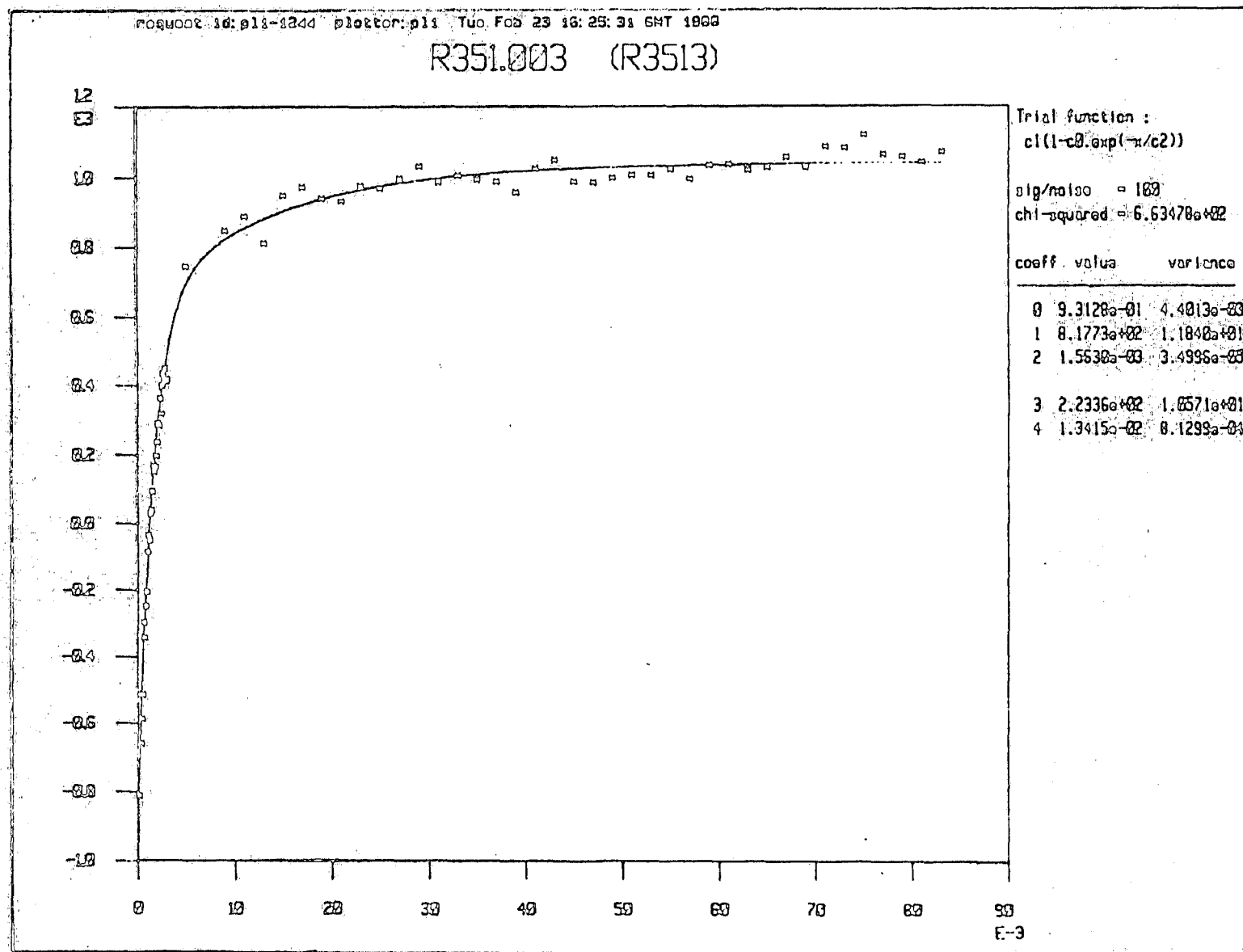
Figure 6.12: ^1\text{H} T_1 determination for partially hydrated calcined high-silica theta-1.
