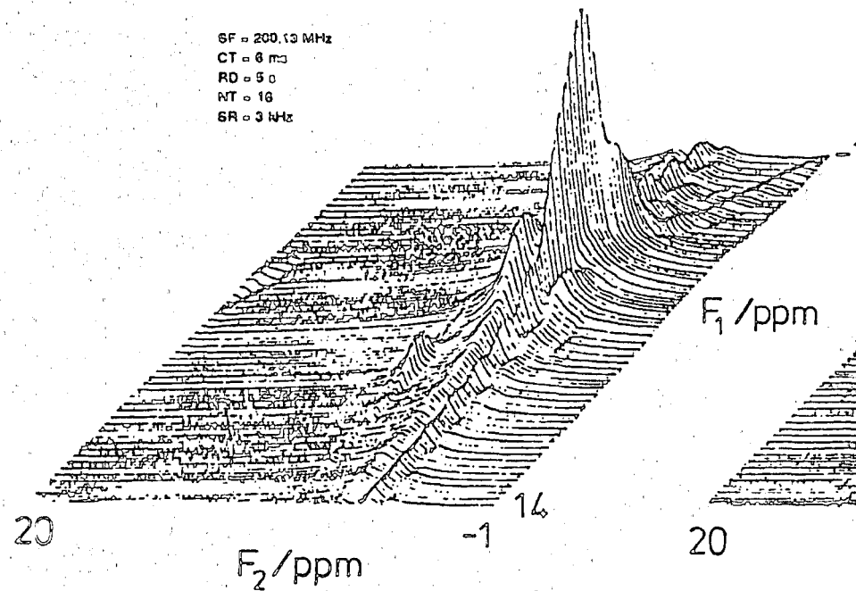
Figure 7.6(b): As-synthesised theta-1 with \tau_m = 6\text{ms} .
