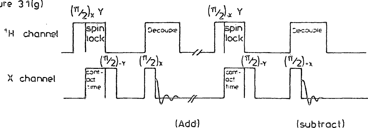
T_1 measurement by cross-polarization (Torchia method).
