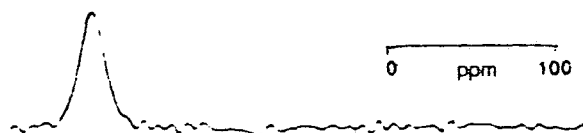
Figure 7.28(a): Application of the MREV-8 pulse sequence to aluminum bromide hexahydrate.
