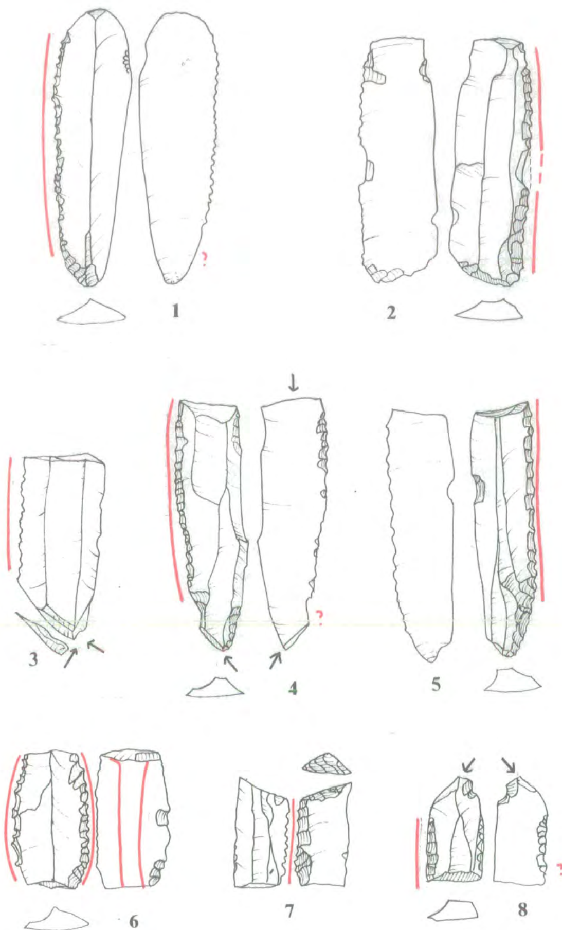
Fig.VI:15 Lusted Flint Blades: Period 3 Ghorraifé (after M.-C. Cauvin). Scale 1:1
