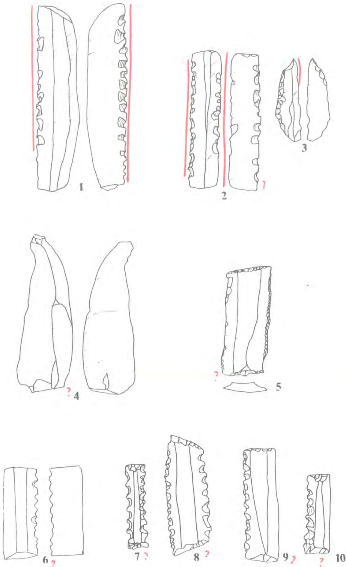
Fig.VI:35 Lustrated Flint Blades: Ubaid, Uruk and Early Dynastic Period nos. 1-3 Tello (after Cauvin), no.4 Abu Khamis (after Masry), no.5 Uruk (after Eichmann), no. 6 Kish and nos. 7-10 Abu Salabikh (after Crowfoot Payne). Scale 1:1
