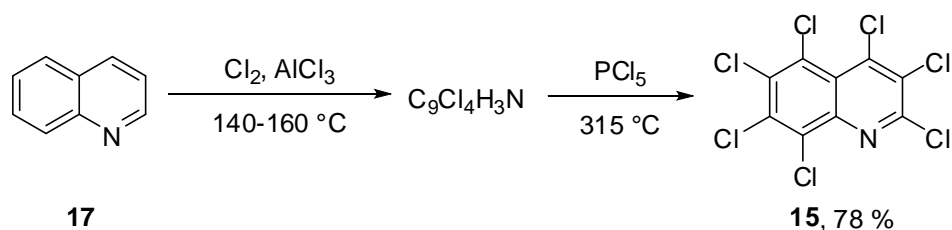
Scheme 4. Synthesis of heptachloroquinoline ( 15 ) from quinoline ( 17 ) 27
