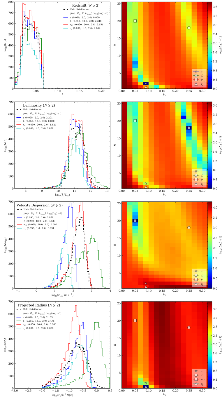
Figure 5.28: Results minimizing the property the \chi^2 statistic using each of the individual halo and group properties. Here we consider only halos and groups for which greater than 50 per cent of the light from the system is visible prior to applying the correction factor. The symbols, lines and colour bar have the same meanings as in Figure 5.4.
