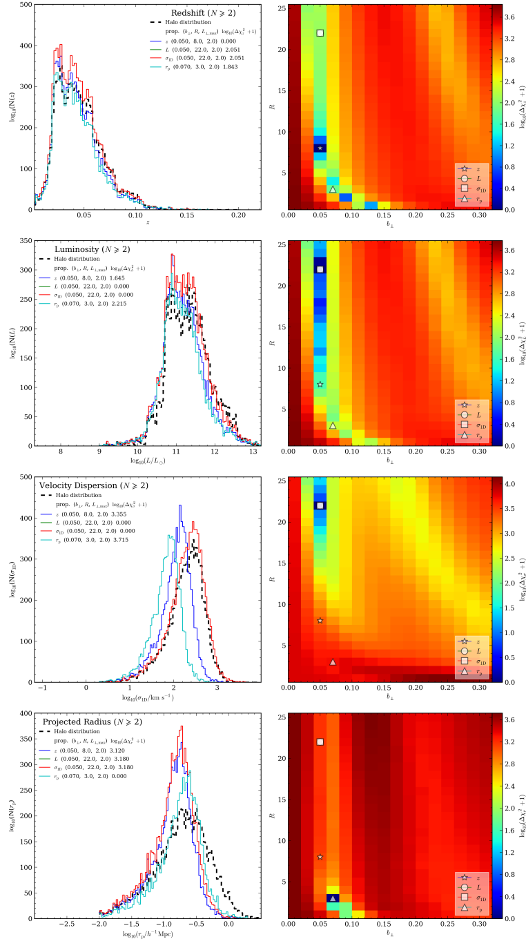
Figure 5.10: Results minimizing the property the \chi^2 statistic using each of the individual halo and group properties. Here we have constructed the property distributions using 100 bins. The symbols, lines and colour bar have the same meanings as in Figure 5.4. Note that the square and the circle symbols are lying on top of one another and the red line and the green line are lying on top of one another.
