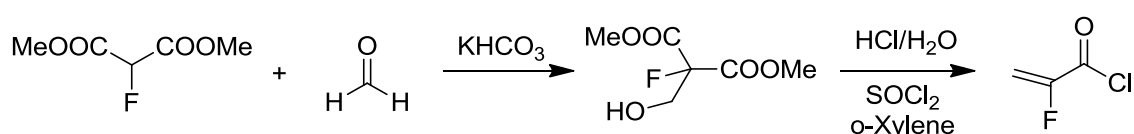
Figure 28: Synthesis of 2-fluoroacrylic chloride from dimethyl fluoromalonate. 97
