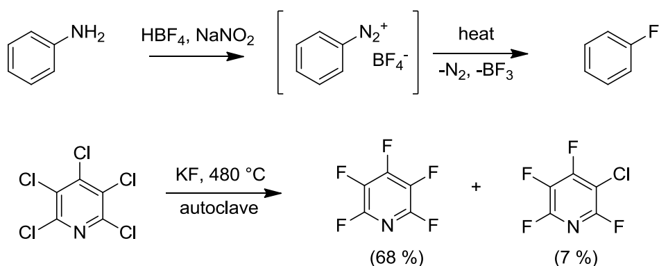
Figure 3: Aromatic fluorination methods: the Balz-Schieman reaction (top) and halogen exchange reaction (bottom).
