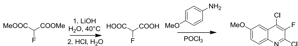
Figure 22: Synthesis of 3-fluoro-6-methoxyquinoline using dimethyl fluoromalonate. 59
