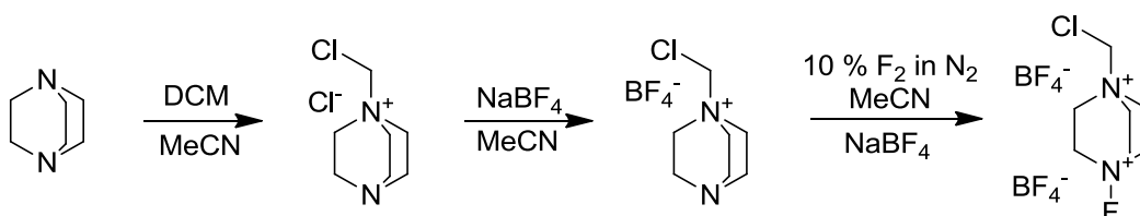
Figure 18: Synthesis of Selectfluor TM .
