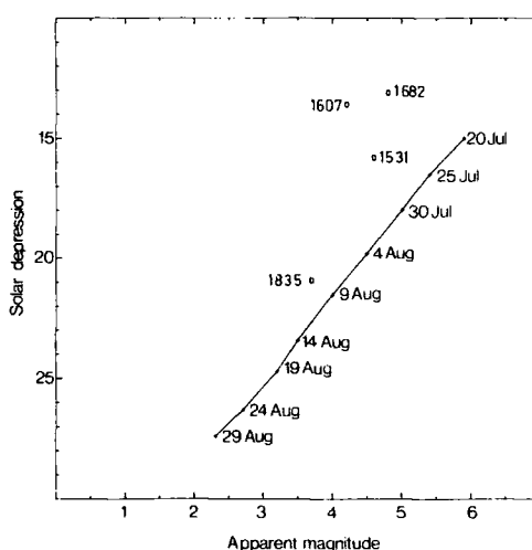
Fig. 6 Plot of the solar depression as a function of the calculated apparent magnitude of P/Halley on the evening of 24 Aug in 87 BC for dates of perihelion between 20 Jul and 29 Aug with, for comparison, the circumstances at the last recorded visibility (in Korea) in AD 1531, 1607, 1682, 1835.
