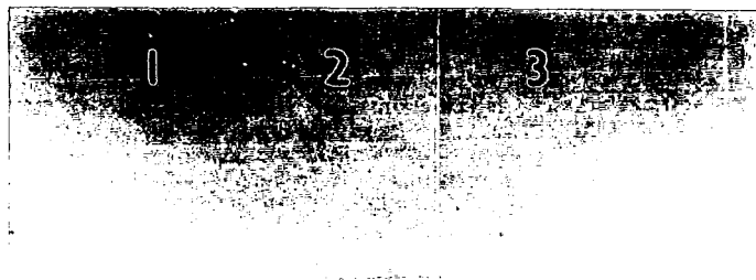
Macroscopic localisation of pPR 179 in Pisum root.
