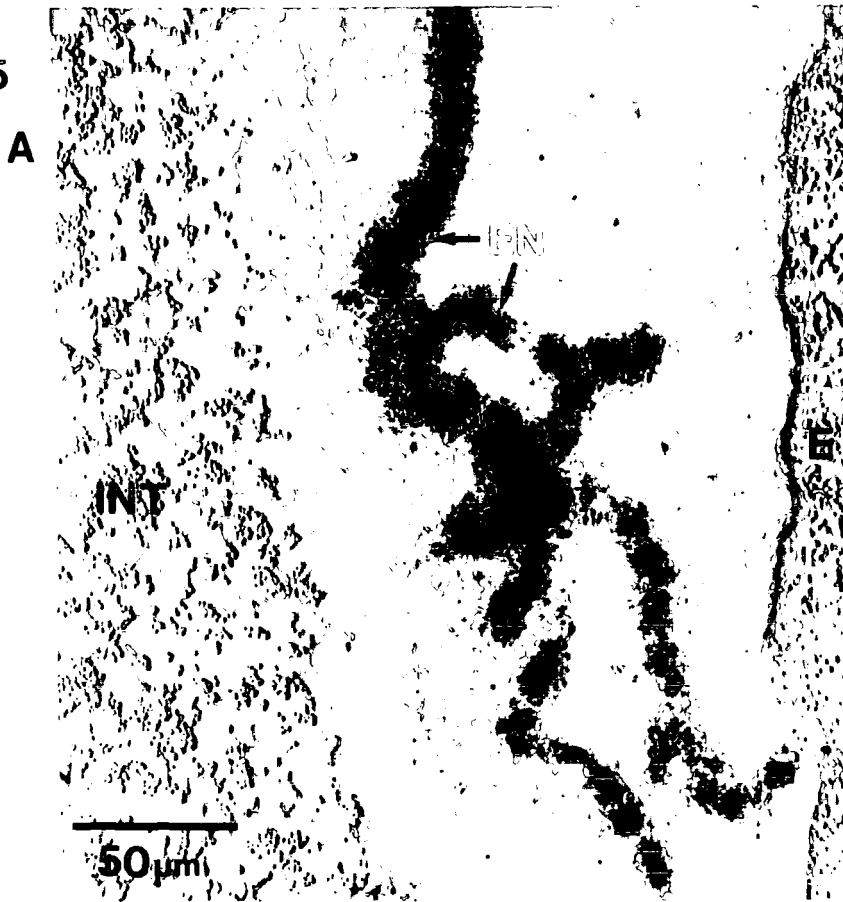
Distribution of legA mRNA in Stage (2) ovule. The section was hybridised with the ^{35}\text{S} labelled probe to legA and hybrids were detected via autoradiography.
