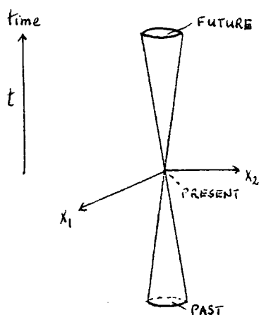
Figure 2 Spacetime cone
