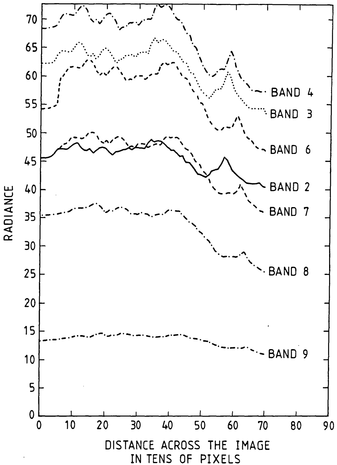
Fig. 4.5 Effect of across-track shading on calibrated ATM 3000m data from Mahd Adh Dhahab area.
