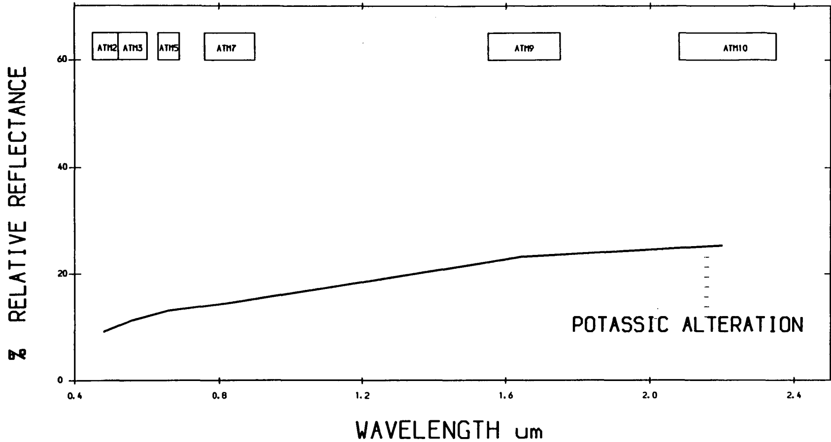
ATM 1000 M BAND EQUIVALENT TO TM CALIBRATED TO RELATIVE REFLECTANCE USING CALIBRATION CURVE MAHD ADH OHAHAB- SAUDI ARABIA
