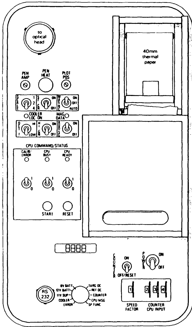
Figure 3. The IRIS Mk IV Control Unit. a) External details.
