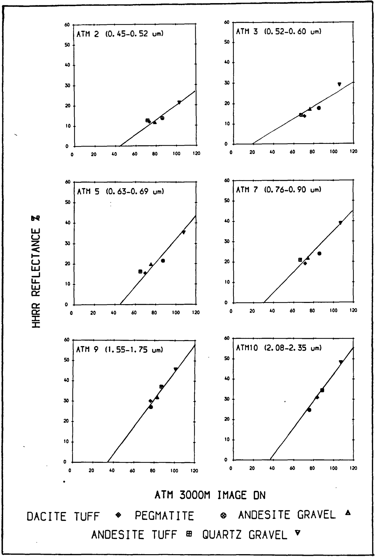
Fig. 4.13 Calibration curve for ATM 3000m data (resolution 7.5m) based on HHRR field measurement, Jabal Said.
