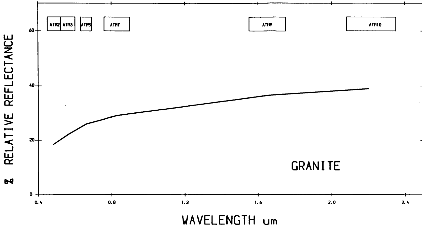
ATM 2000 M BAND EQUIVALENT TO TM CALIBRATED TO RELATIVE REFLECTANCE USING CALIBRATION CURVE JABAL SAID AREA - SAUDI ARABIA
