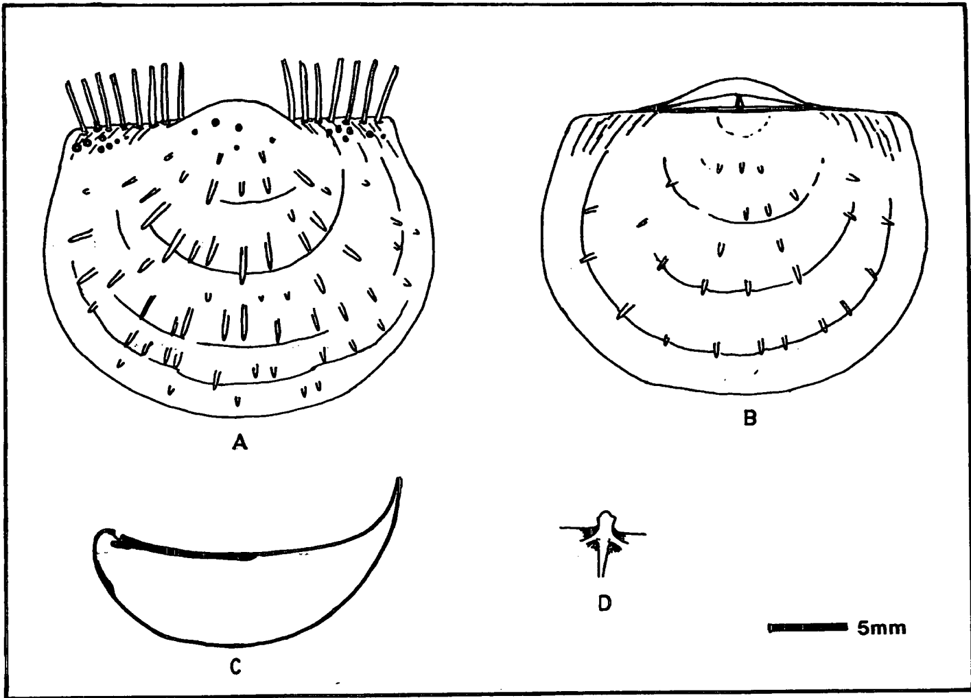
Text-figure 3.4. Reconstruction of Eostrophalosia permiana new species A - ventral view (exterior). B - dorsal view (exterior). C - lateral profile. D - cardinal process.
