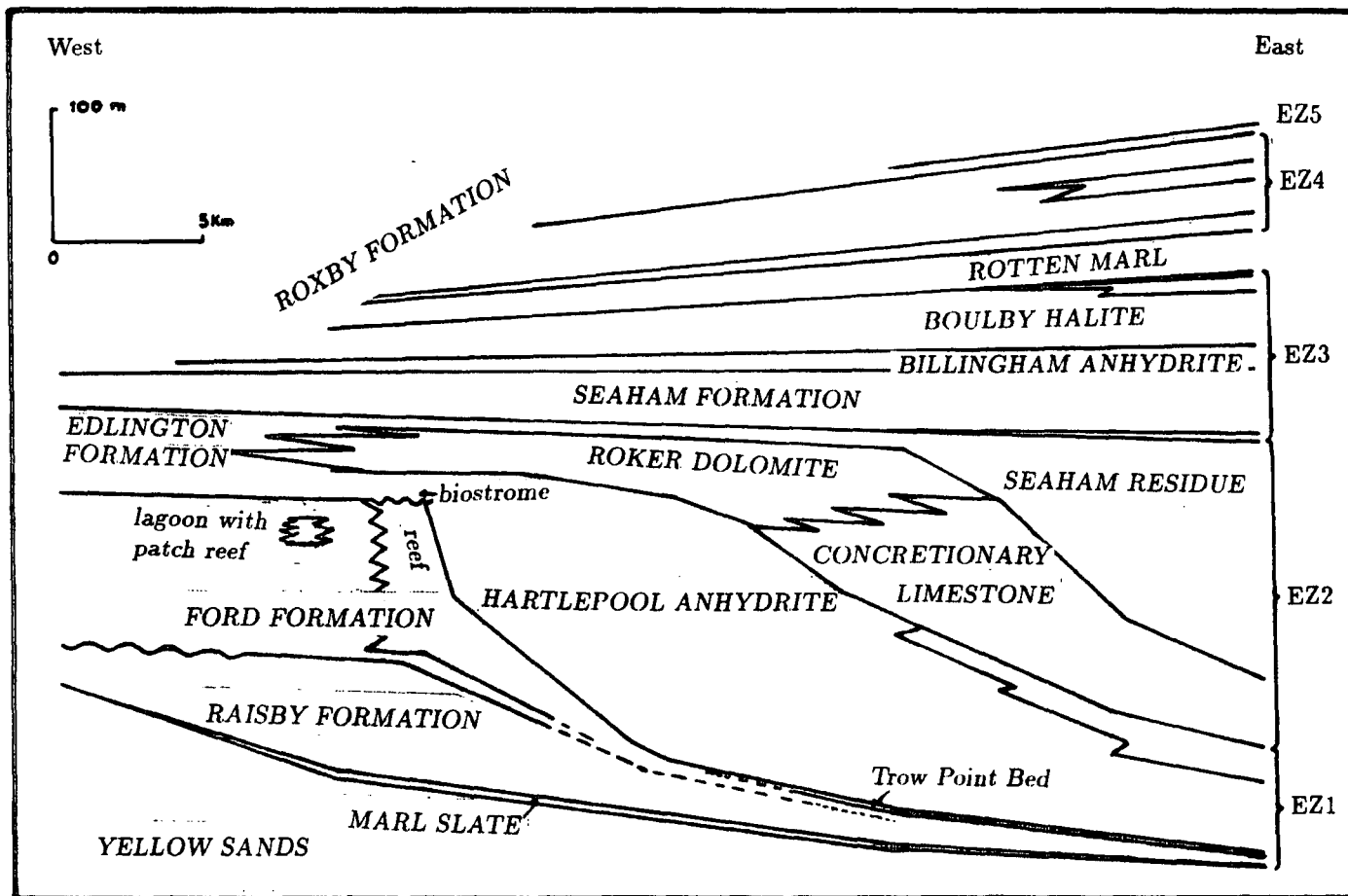
Text-figure 2.3. Lithostratigraphic correlation in the Zechstein of Durham Province [Modified from Smith (1989)]
