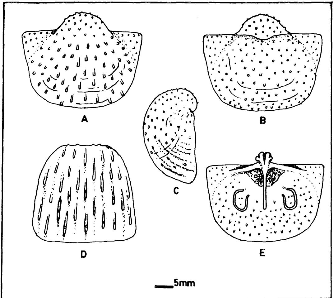
Text-figure 3.19. Reconstruction of Spinohorridonia geinitziana (de Koninck). A,C,D - Exterior of ventral valve: ventral, lateral and anteroventral views. B,E - Exterior and interior of dorsal valve.
