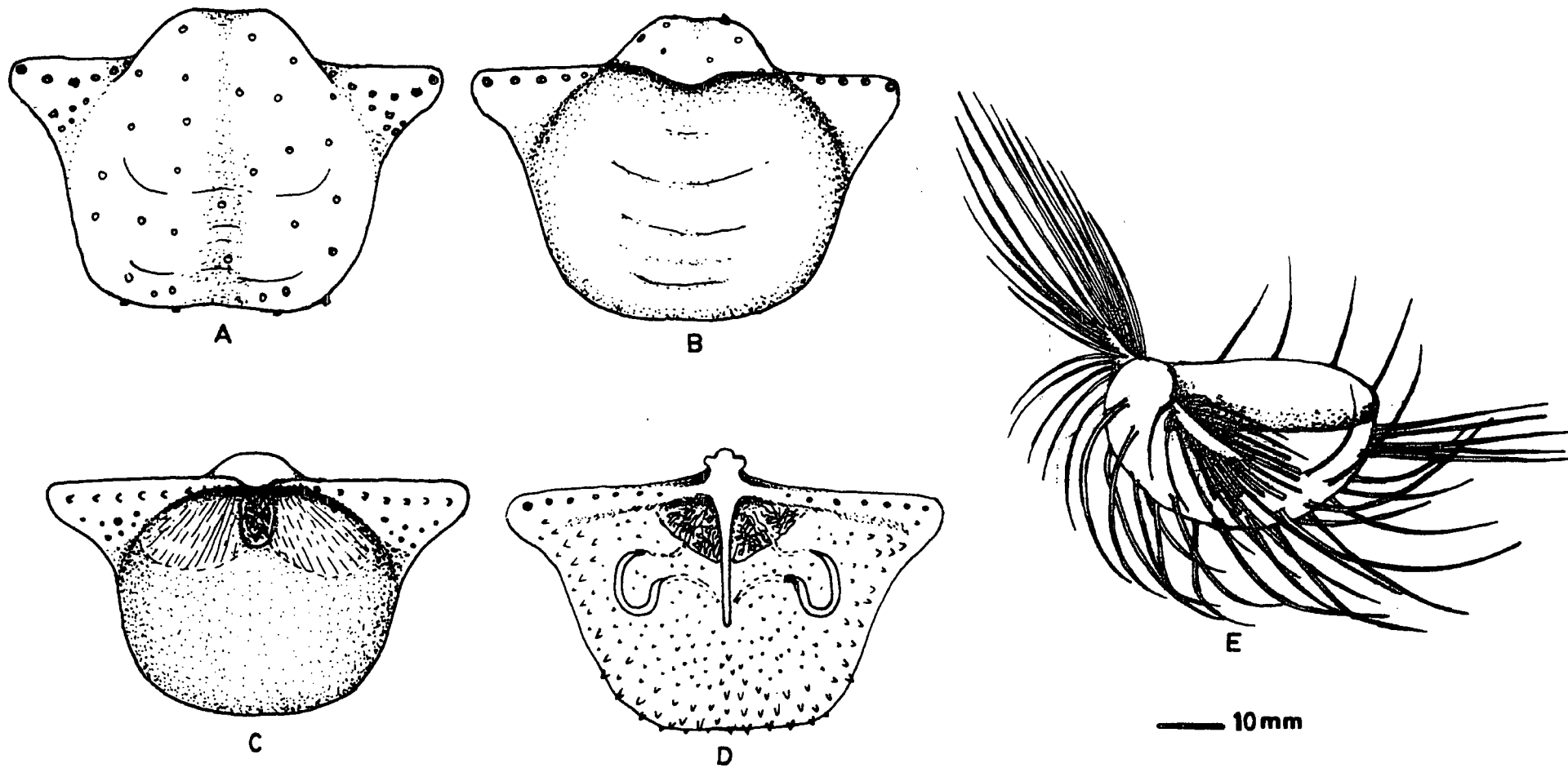
Text-figure 3.18. Reconstruction of Horridonia dunelmensis new species. A,B - Exterior of ventral and dorsal valves. C,D - Interior of ventral and dorsal valves. E - Common life position of Horridonia dunelmensis .
