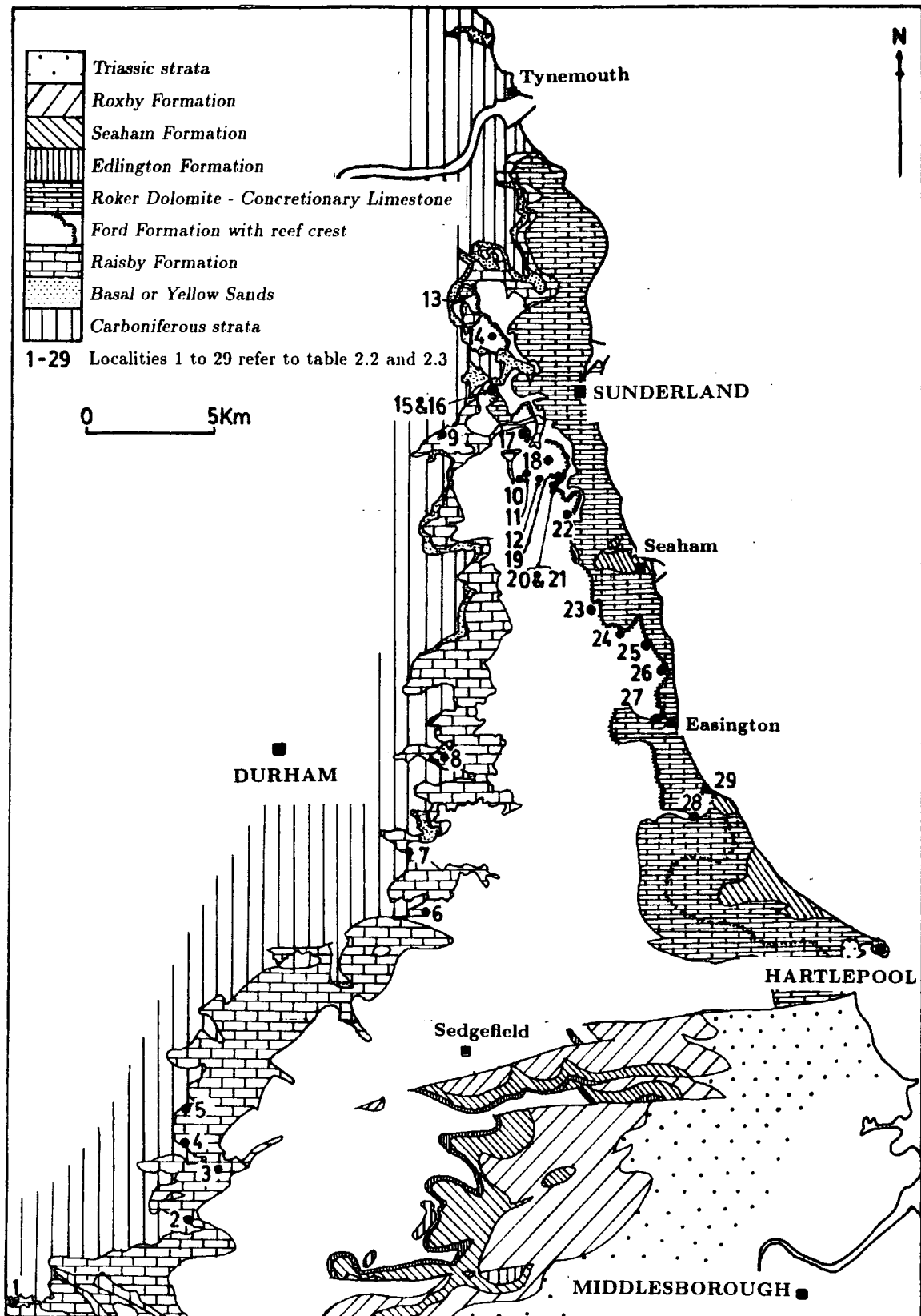
Text-figure 2.2. Zechstein rock formations in Durham Province [After Smith (1980) and Smith et al. (1986)]
