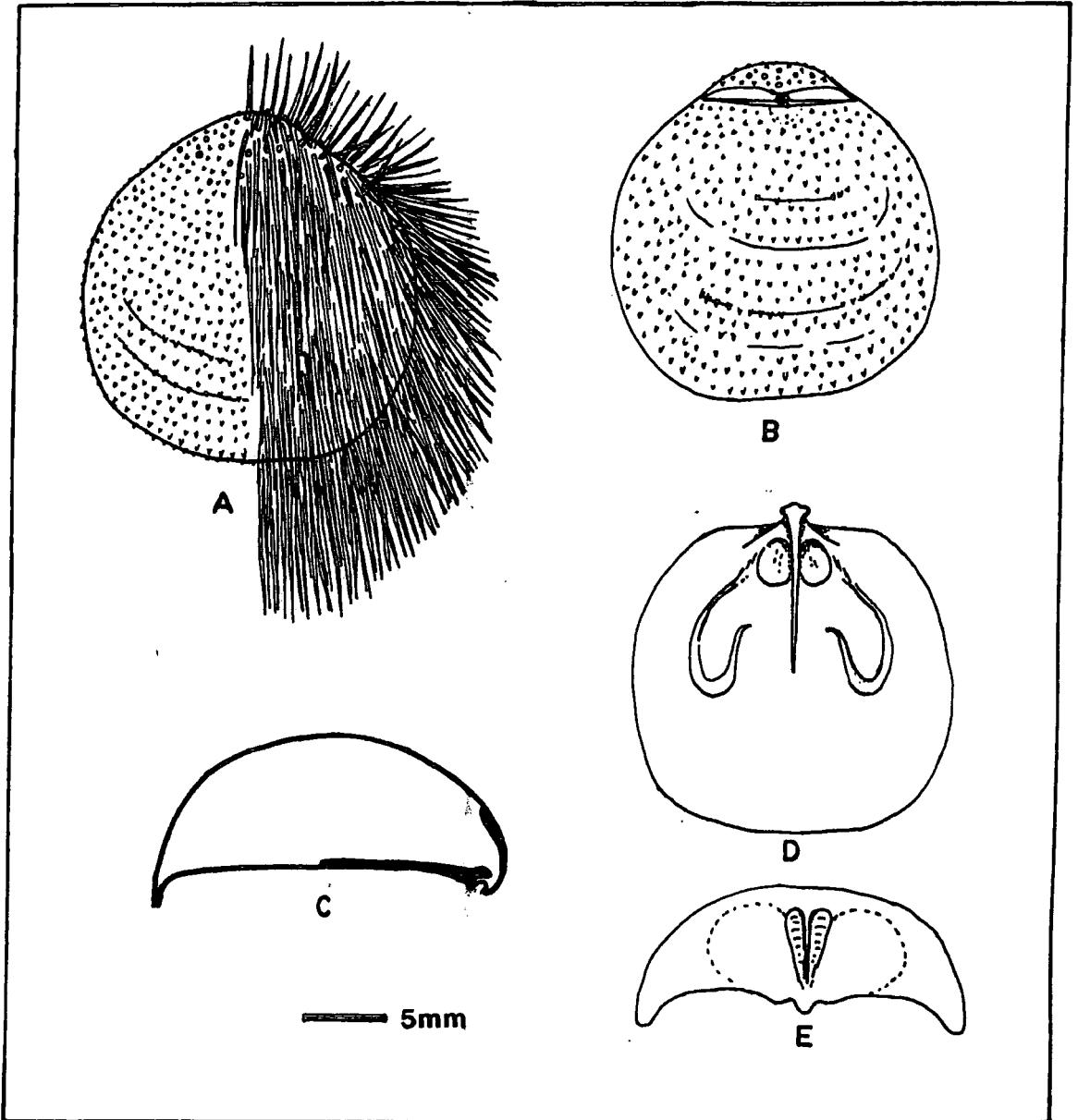
Text-figure 3.1. Reconstruction of Strophalosia lewisiana (de Koninck)
