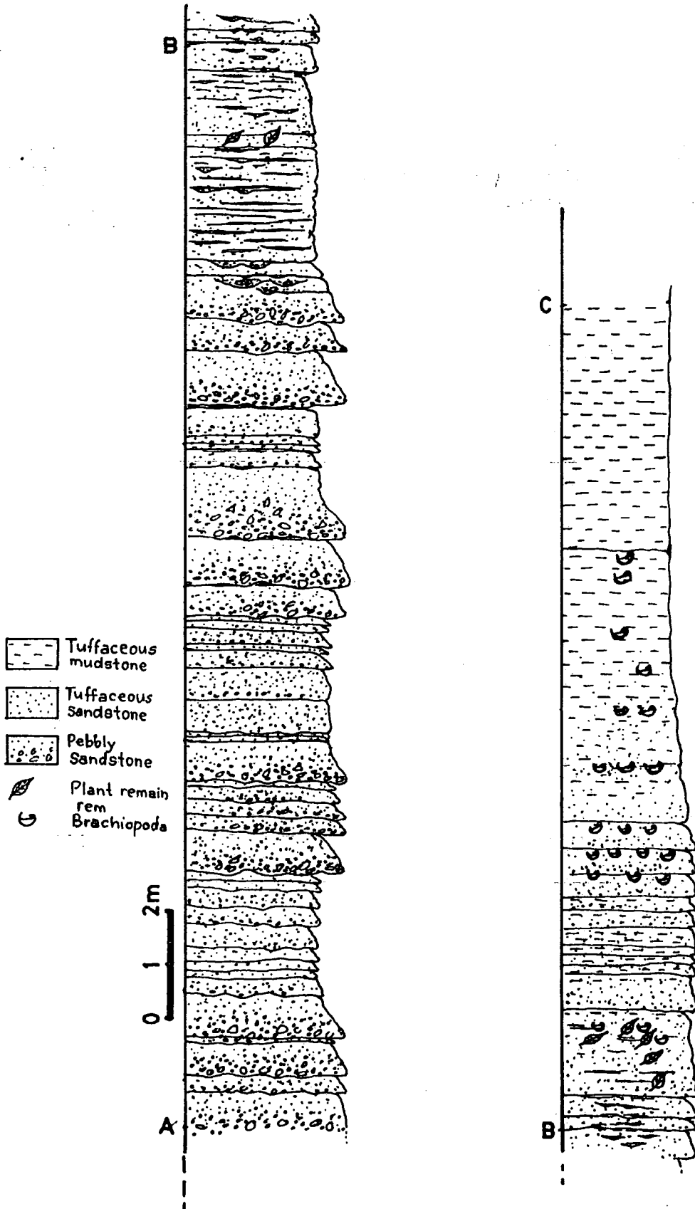
Text-figure 4.4. Stratigraphic column at locality 16, north of Sungai Toh, Merapoh, Pahang.
