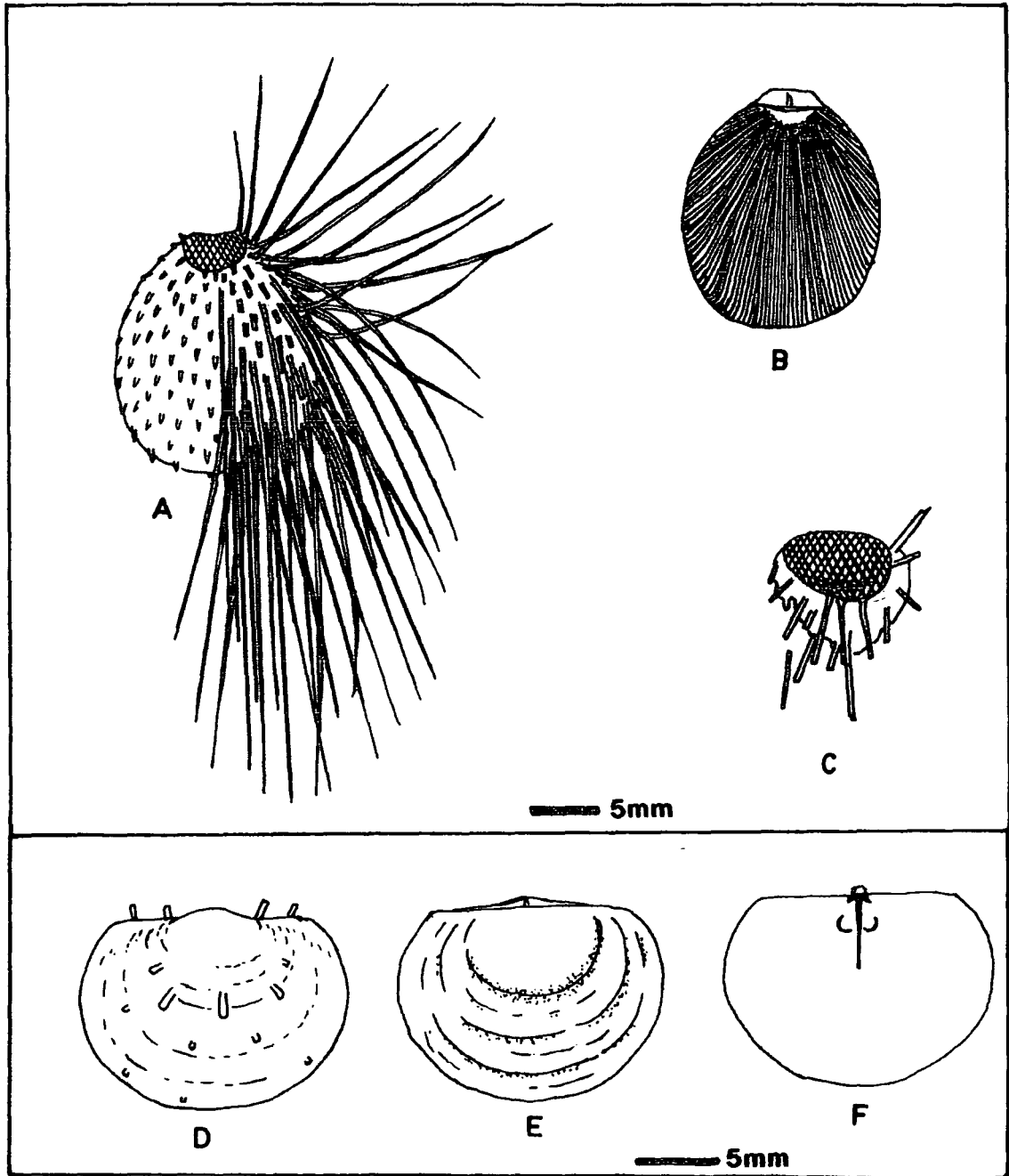
Text-figure 3.9. Reconstruction of Heteralosia aclyffensis new species (figure A to C) and Heteralosia? quarringtonensis new species (figure D to F).
