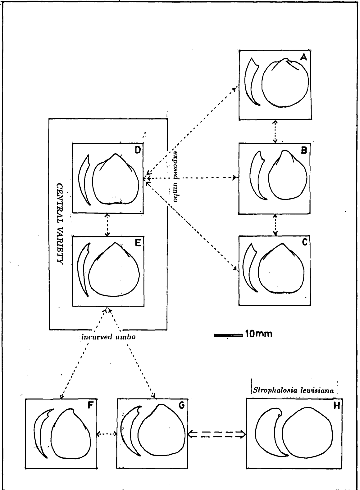
Text-figure 3.2. Variation in Strophalosia excavata (Gelnitz) from Beacon Hill railway cut
