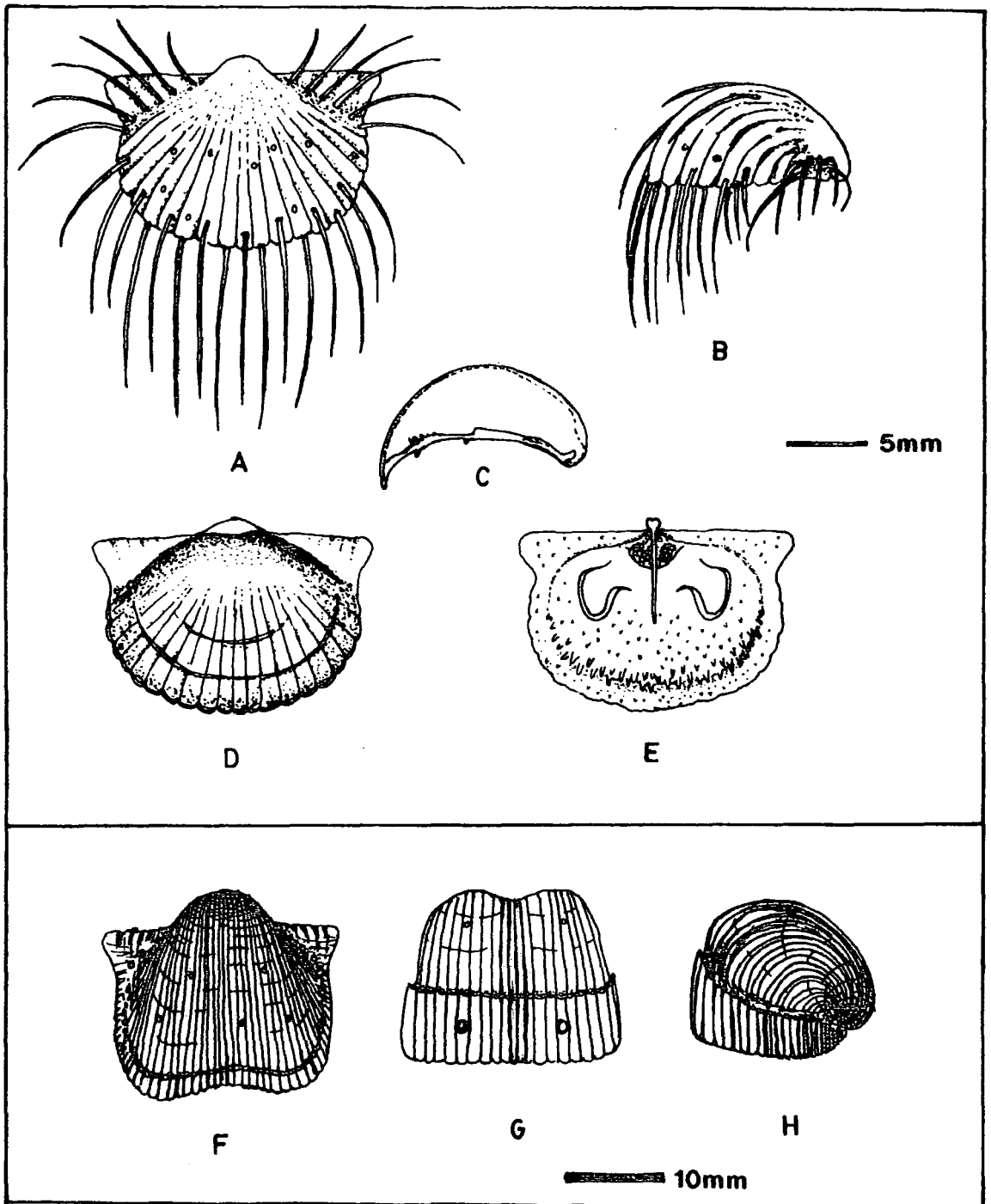
Text-figure 5.2. Reconstructions of Liosotella nakamurai new species (figure A-E) and Marginifera? sp. A (figure F-H)
