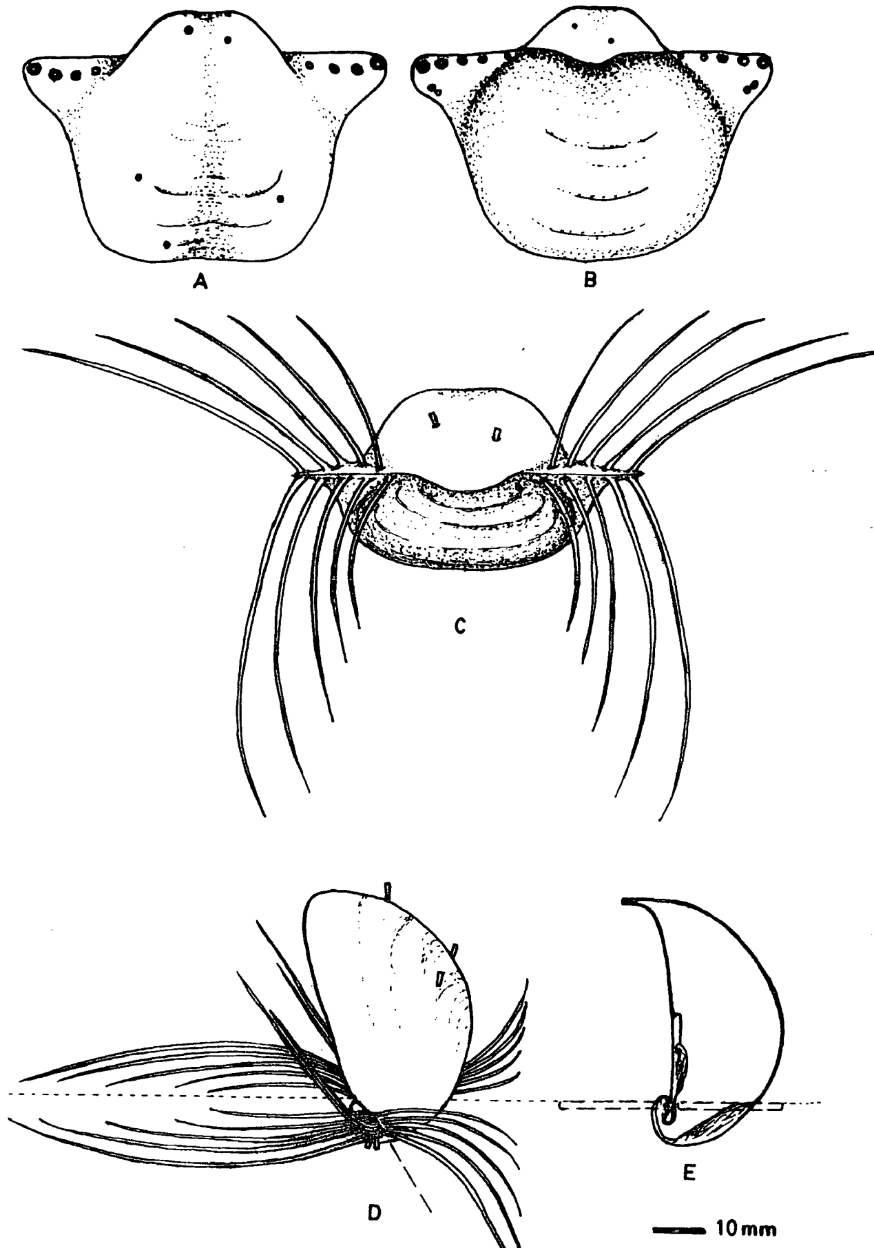
Text-figure 3.16. Reconstruction of Horridonia horrida (Sowerby).
