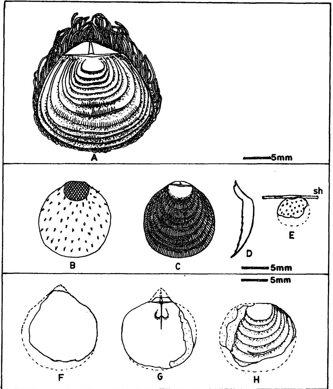
Text-figure 3.10. Reconstruction of British species of Craspedalosis .
