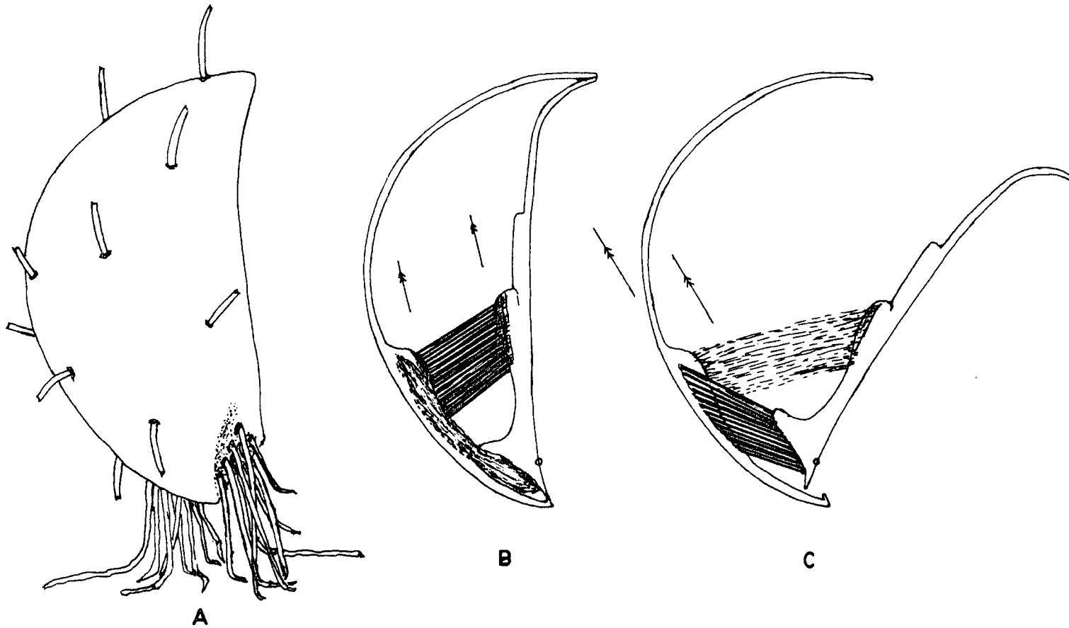
Text-figure 3.12. Howseia latirostrata ; A - Attachment by auricular spines; B - C - articulation mechanism.
