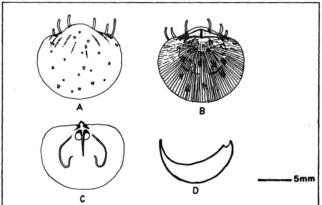
Text-figure 3.8. Reconstruction of Heteralosia seahamensis new species.
