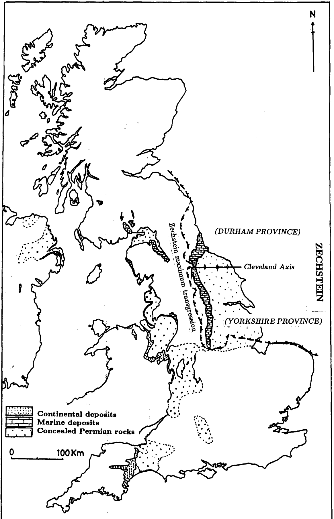
Text-figure 2.1. Distribution of Permian strata in Britain [After Smith et al. (1974) and Smith (1989)]
