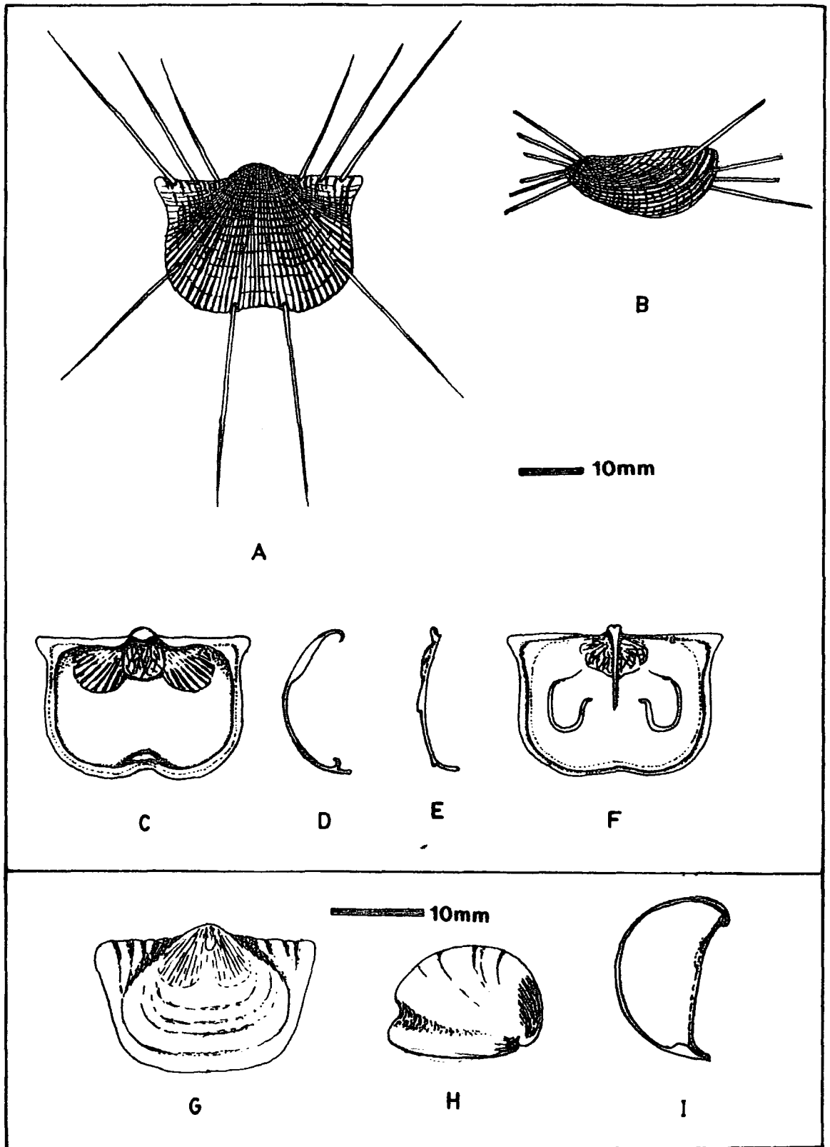
Text-figure 5.3. Reconstructions of Retimarginifera lipisensis new species (figure A-F) and Echinauris? sp. A (figure G-I)
