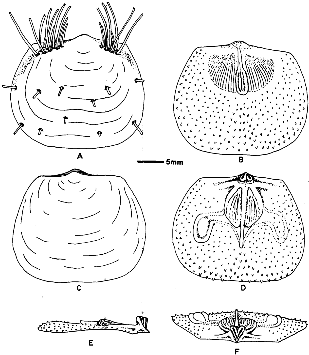
Text-figure 3.11. Reconstruction of Houseia latirostrata (Howse). A,B - Exterior and interior of ventral valve. C - Exterior of dorsal valve. D,E,F - Interior of dorsal valve; plan, lateral and posterior views.
