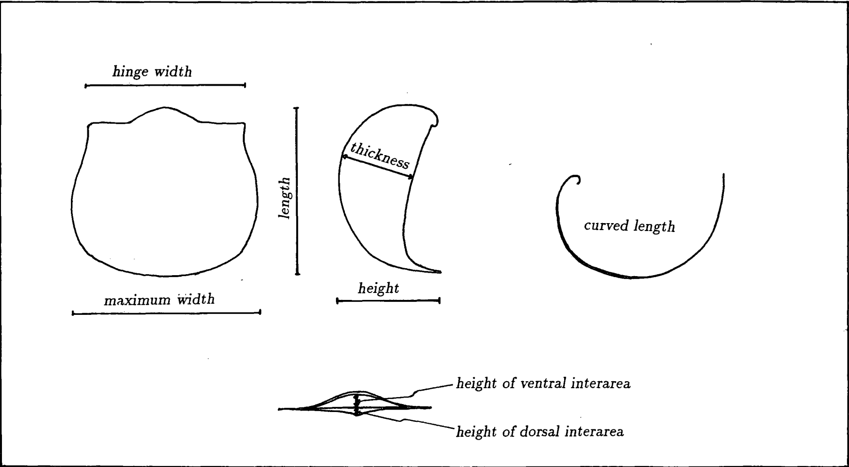
Text-figure 1.1. Measured dimensions
