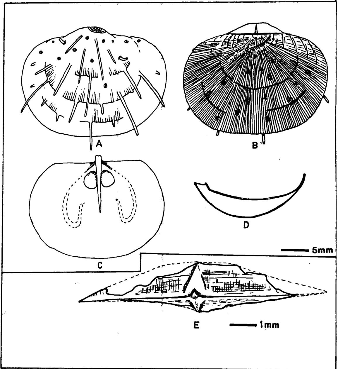
Text-figure 3.5. Reconstruction of Heteralosia morrisiana (King)
