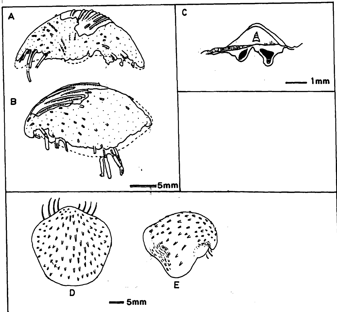
Text-figure 3.6. Camera lucida reproduction of Heteralosia humbletonensis (King). A,B - Posterior and lateral views of syntype no D318B (UCG collection). C - Interior of ventral interarea of syntype no D318C (UCG collection) showing a pair of deep sockets (darken). D,E - ventral and lateral view of specimen no G88.56a (HM collection).
