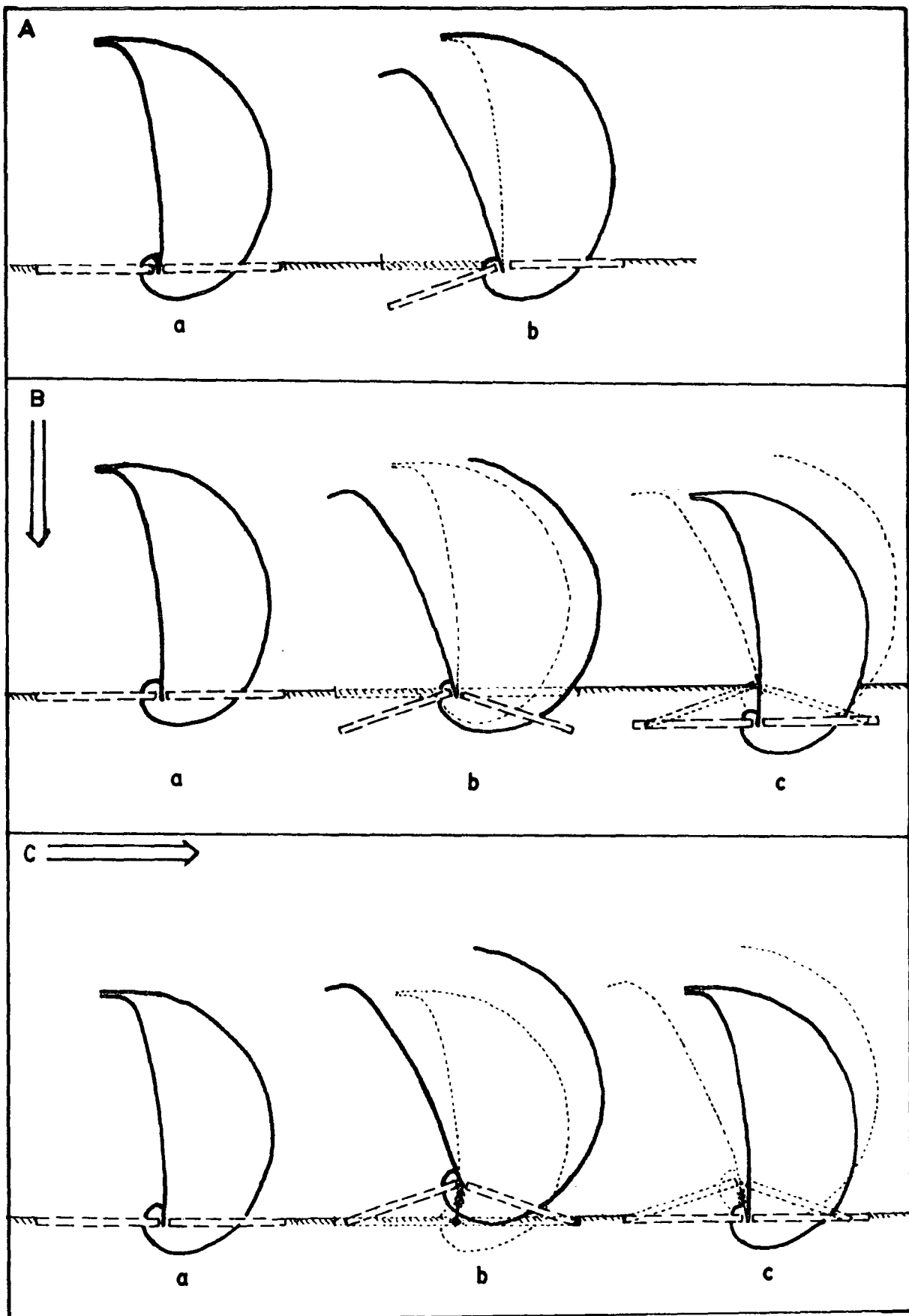
Text-figure 3.17. Postulation of various moving mechanisms in Horridonia horrida .
