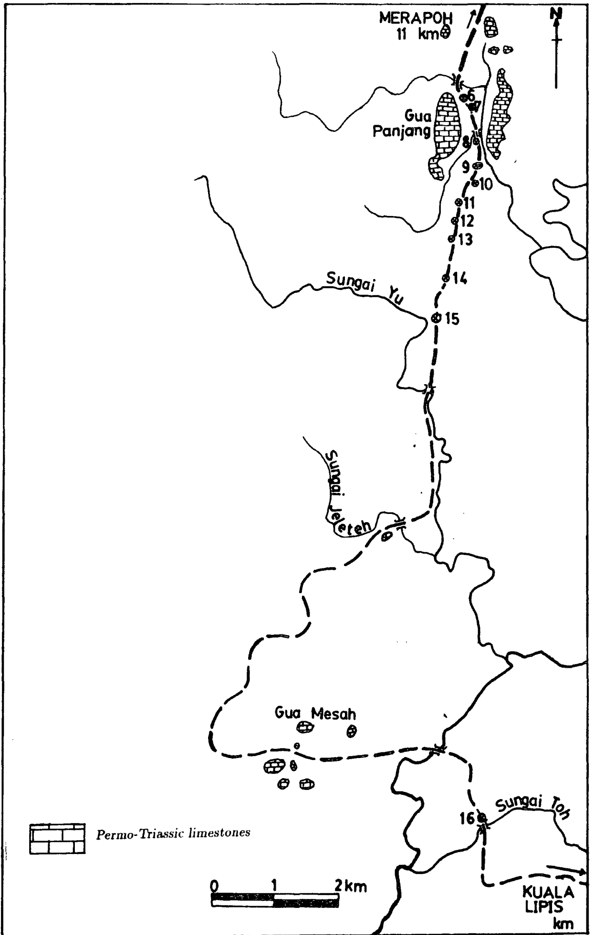
Text-figure 4.3. Distribution of localities 6 to 16 along the Dada Kering - Gua Musang Highway, Northwest of Pahang.
