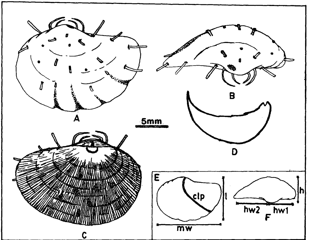
Text-figure 3.7. Reconstruction of Heteralosia hyltonensis new species.
