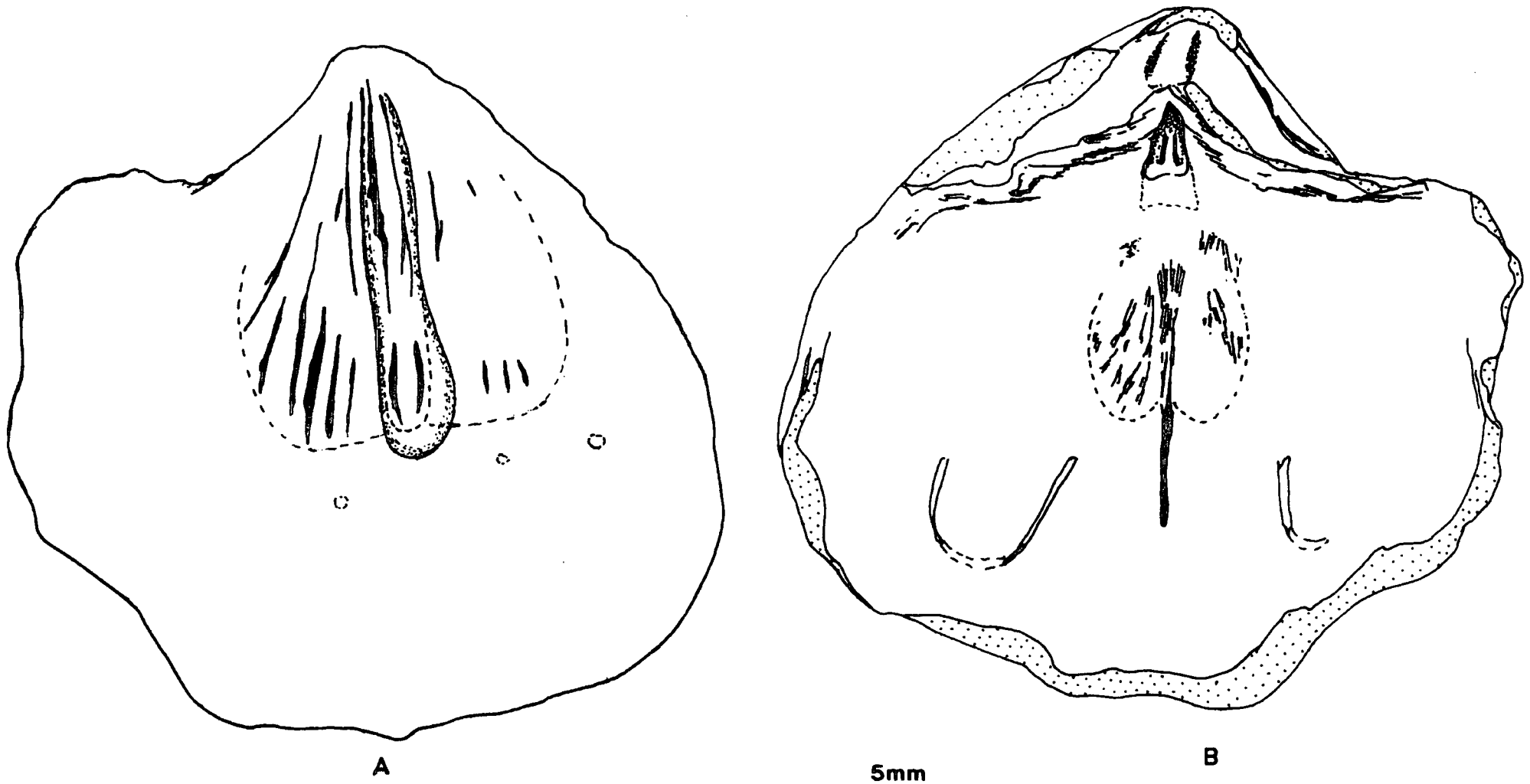
Text-figure 3.14 Camera lucida reproduction of the holotype of Howseia umbonilata (King); specimen no D184B (UCG collection). A - ventral view. B - dorsal view [rock matrix is dotted; - - - - reconstructed outline of various internal morphology].
