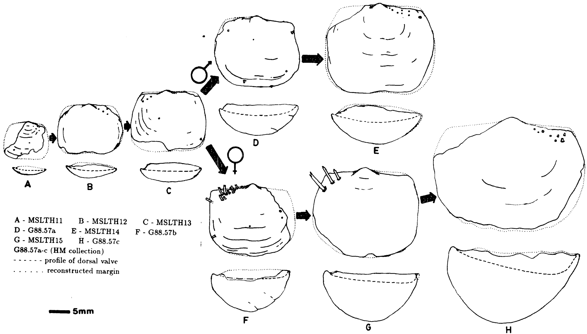
Text-figure 3.13. Ontogenic development of Howsea latirostrata from Tunstall Hill rock cottage.
