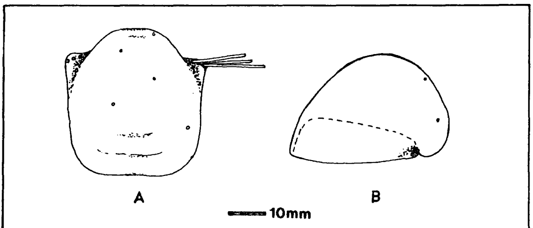
Text-figure 3.20. Reconstruction of Horridonia hoppeiana (Eisel) A,B — Ventral exterior (ventral and lateral views).
