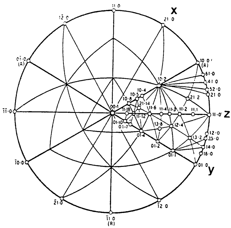
Figure 5.01 shows the stereographic projection of LiNbO_3 in terms of the hexagonal parameters hkil , ignoring the rhombohedral requirements -h+k+l=3N . After Nassau et al (1966).
