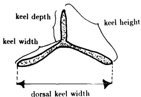
Figure 2.8 — Keel Cross-Section
