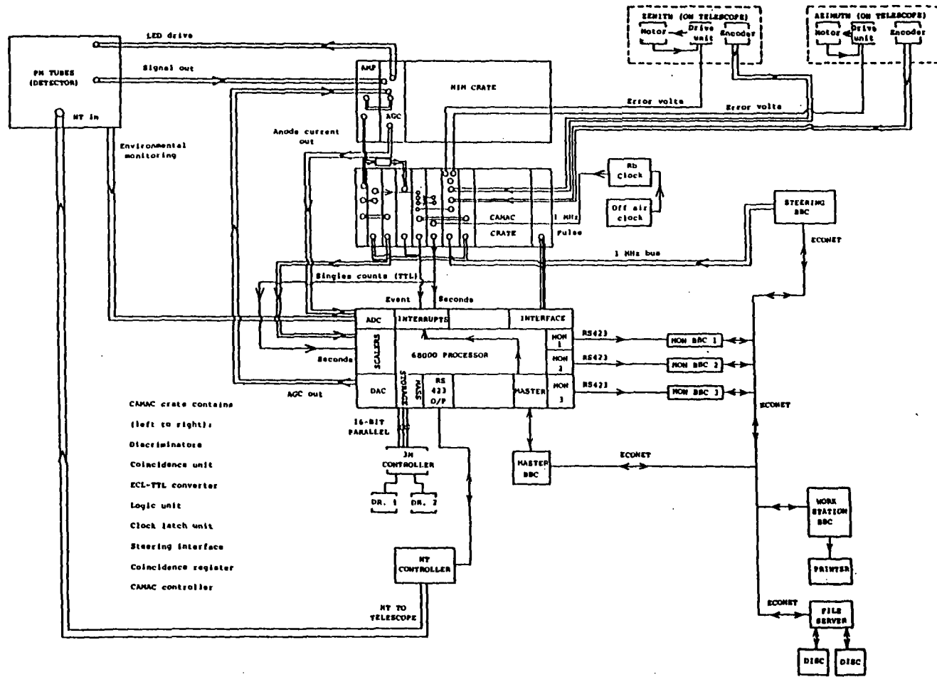
Figure 2.3 Data logging system of the Mark III telescope (from Brazier et. al., 1989a)
