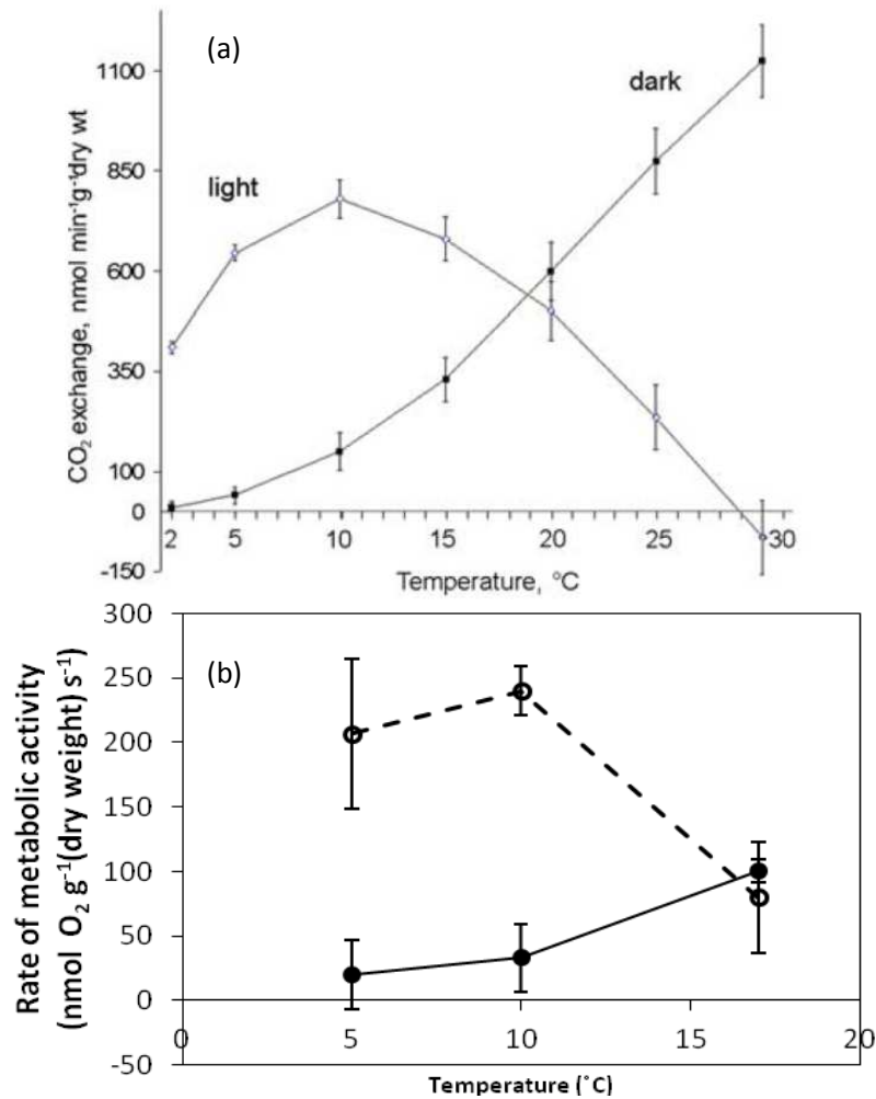
Figure 4.4.1: (a) Figure 1 from Aubert et al. (2007) illustrating the rate of CO 2 exchange of X. elegans thalli, at 500 \mu\text{mol m}^{-2} \text{s}^{-1} light intensity, at a range of temperatures. (b) Data for C. stellaris taken, in the present study, at 510 \mu\text{mol m}^{-2} \text{s}^{-1} , from the results in Section 4.3, rate of NP is depicted by open circles and DR by closed circles. Aubert et al. (2007) compared directly results from IRGA and oxygen electrode measurements, so the comparison here is justified.
