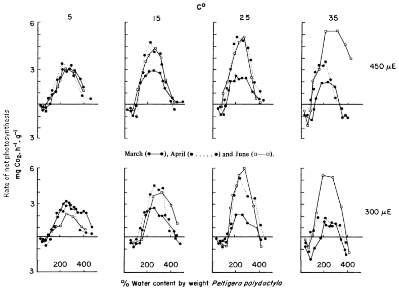
Figure 1.5.1: Net photosynthetic rate of Peltigera polydactyla , at 300 and 450 \mu\text{E m}^{-2} \text{s}^{-1} light intensities, and 5°, 15°, 25° and 35°C. Water content is expressed as a percentage of oven dry weight. Mean rates are given from thalli collected at different seasons through the year. From Kershaw (1977) - Figure 4.
