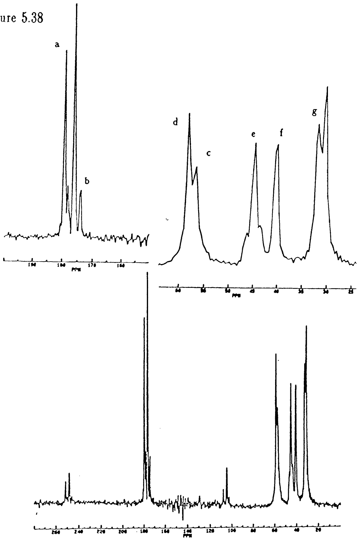
b). The ^{13}\text{C} CP NMR spectrum of the isolated salt.
