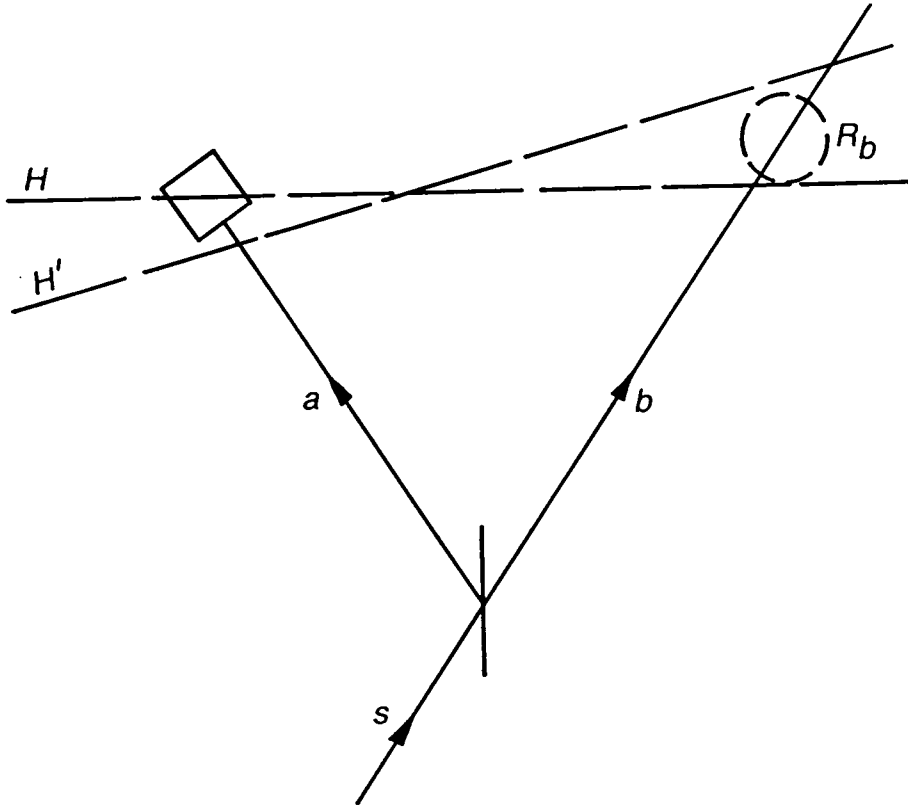
Fig. 9.1. Space-time diagram of a single particle impinging on a beam splitter.
