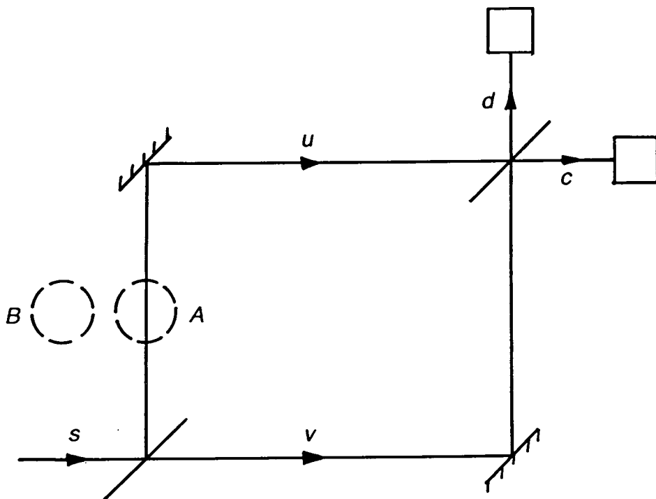
Fig. 9.2. The apparatus discussed by Elitzur and Vaidman. The path difference is set such that when there are no obstacles in the paths there is destructive interference in the d output.
