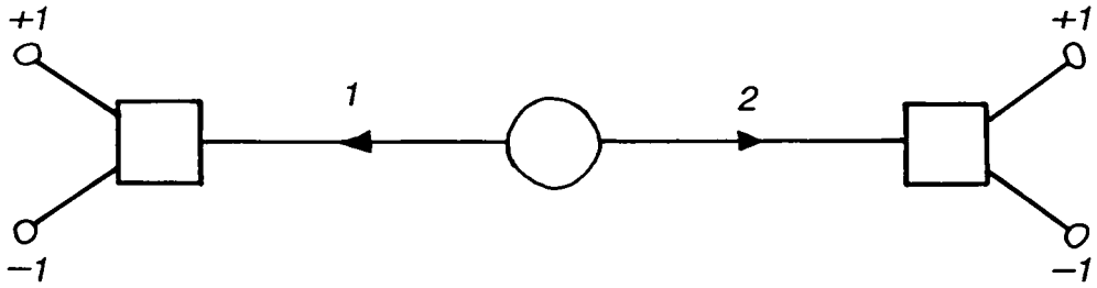
Fig. 4.1. Apparatus used to run Bell's demonstration of nonlocality.
