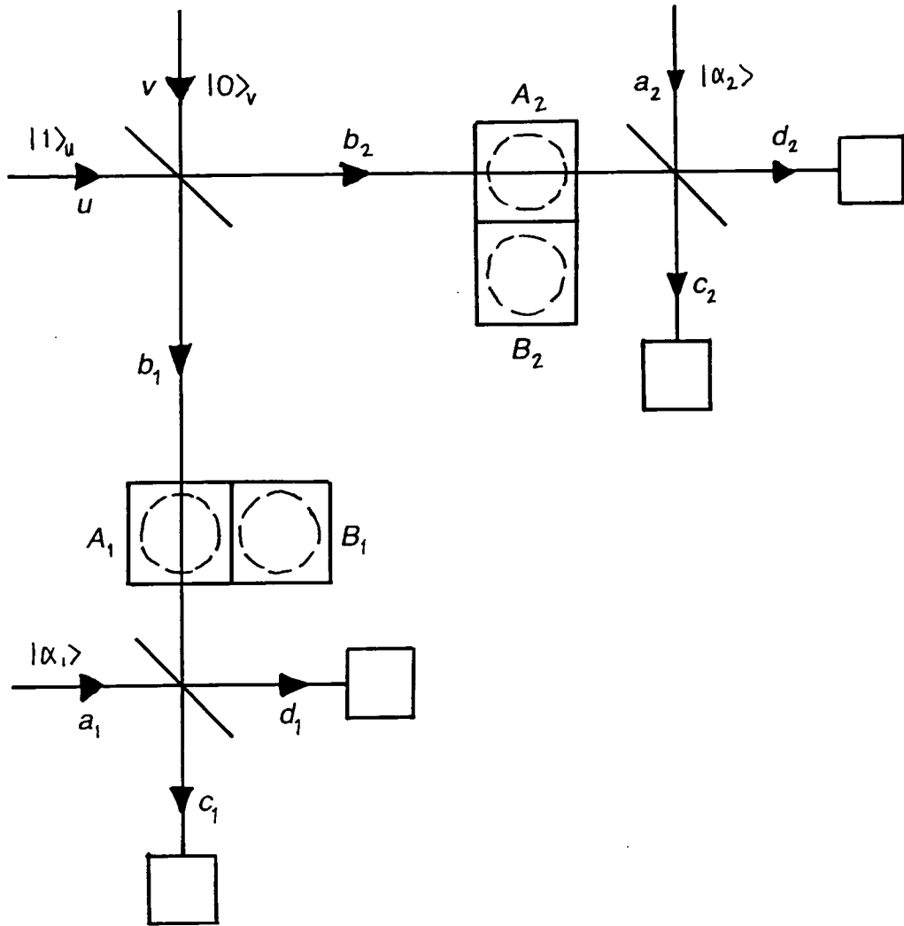
Fig. 6.3. The apparatus of Tan, Walls and Collett with an 'atom plus boxes system' placed in each internal path.
