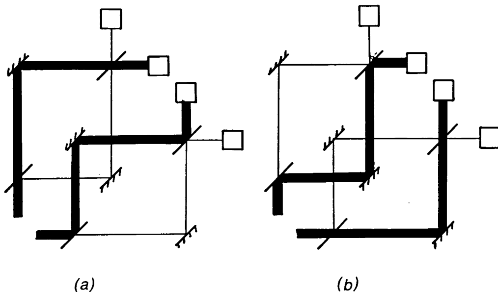
Fig. 9.5. Trajectories calculated (a) in the F_1 frame of reference and (b) in the F_2 frame of reference.
