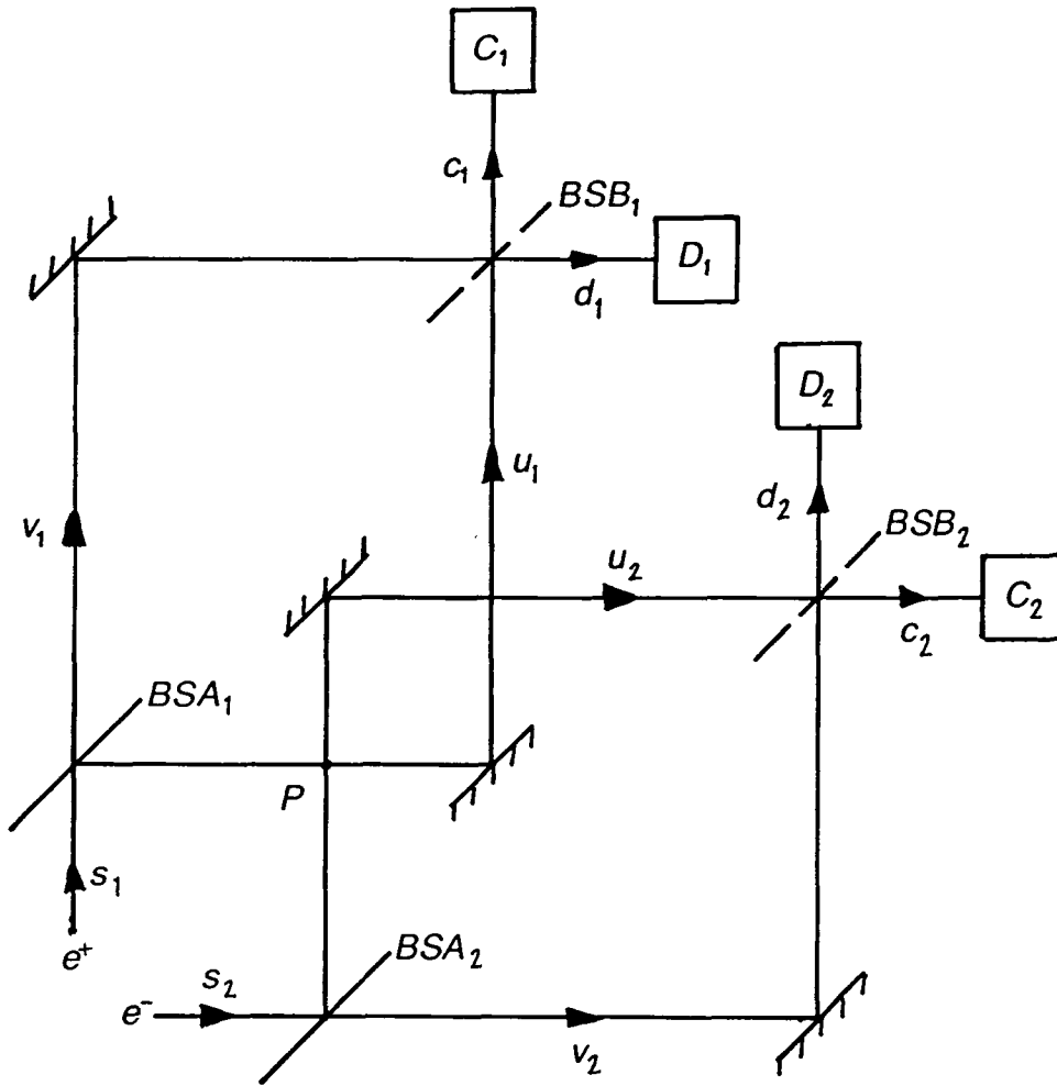
Fig. 8.1. Two Mach-Zehnder-type interferometers, one for positrons and one for electrons, arranged such that if a positron takes path u_1 and an electron takes path u_2 then they will meet at point P and annihilate one another.
