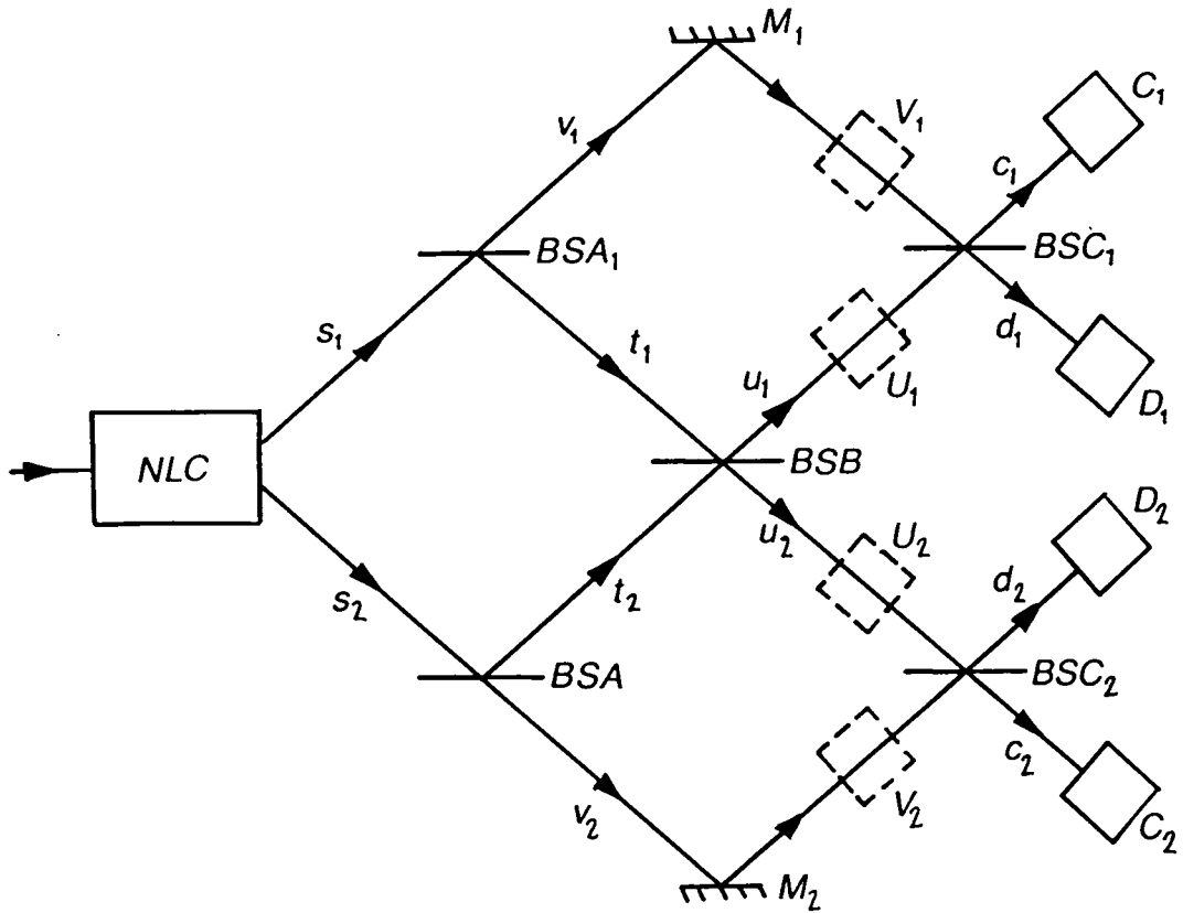
Fig. 8.4. Photon pairs are created by degenerate parametric down conversion. Each photon of the pair is fed into an interferometer system. The two interferometer systems meet at the beam splitter BSB .
