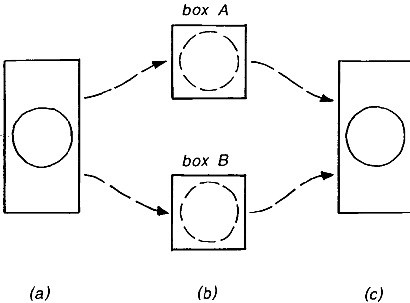
Fig. 3.3. (a) The atom, with spin +\frac{1}{2} along the x axis is placed in a box and a non-uniform magnetic field is placed along the z axis. (b) Dividing walls are placed so as to create two boxes A and B . (c) The boxes are brought back together and the dividing walls are removed.
