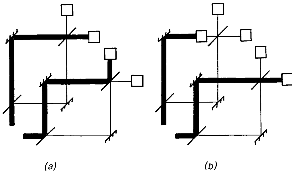
Fig. 8.2. Illustration of nonlocality with trajectories.
