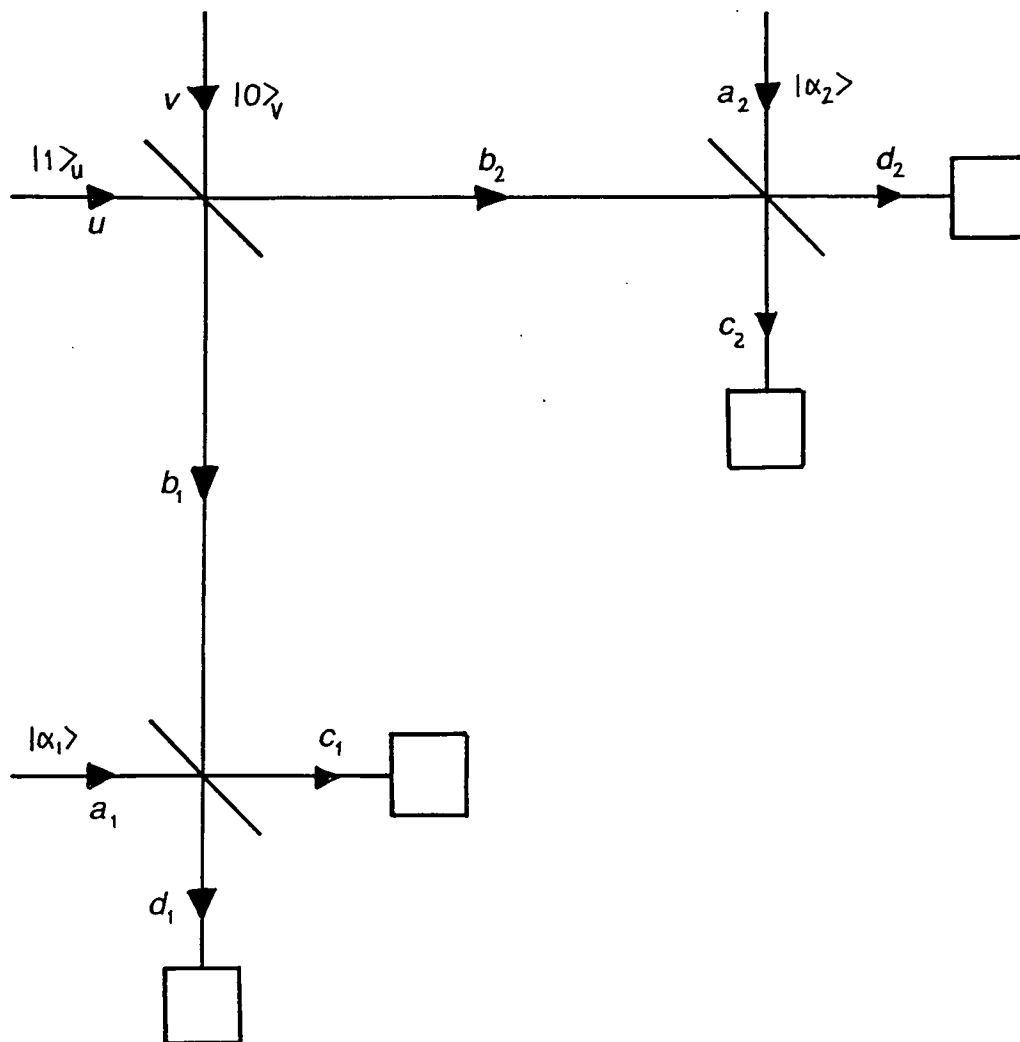
Fig. 6.1. A single photon impinges on a beam splitter and homodyne detection is performed on each output.
