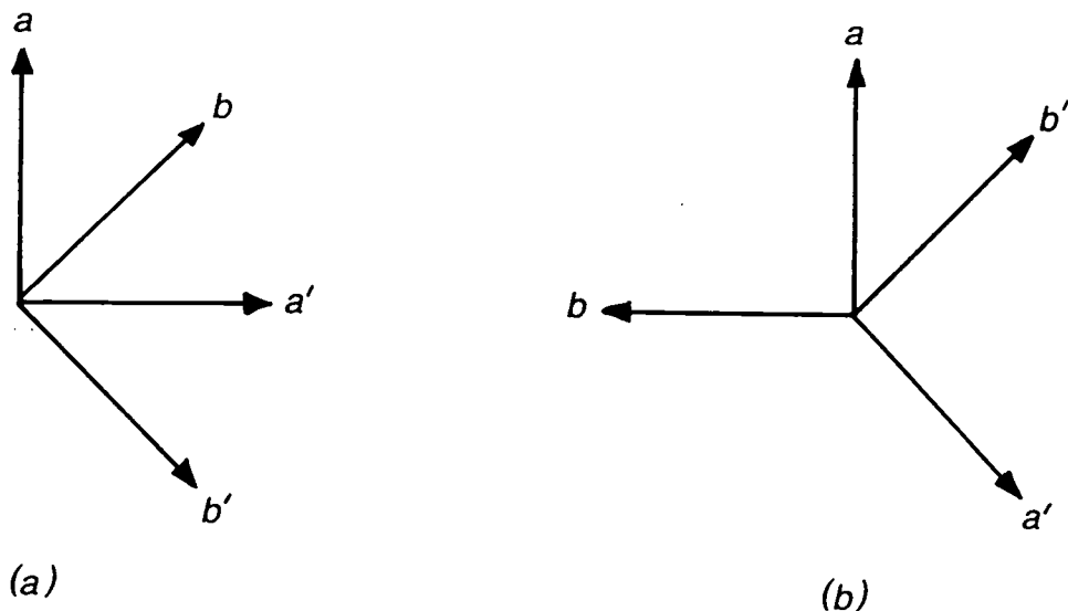
Fig. 4.2. Settings for maximum violation of (a) the upper limit and of (b) the lower limit of the CHSH inequalities for the singlet state.
