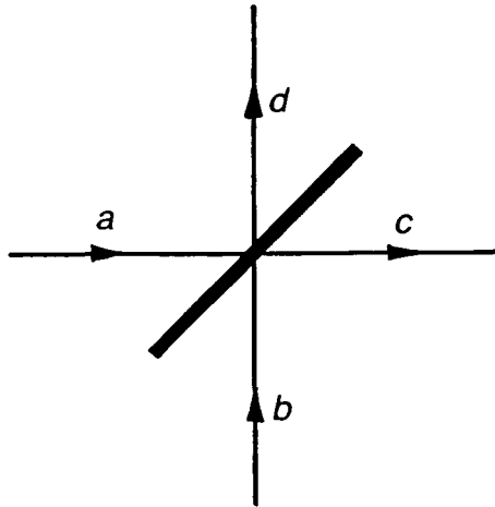
Fig. 8.5. A beam splitter with inputs a and b and outputs c and d .
