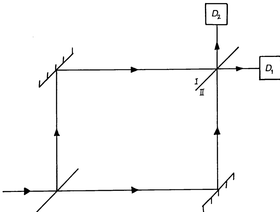
Fig. 2.2. Interference experiment performed by Grangier et. al.
