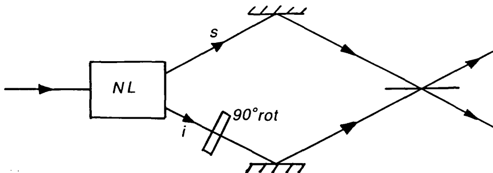
Fig. 5.1. Photon pairs are created by parametric down conversion. The polarisation of one photon is rotated by 90^\circ and then the two modes are mixed at a beam splitter.
