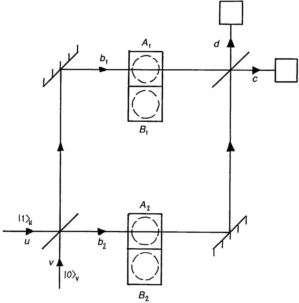
Fig. 6.2. A Mach-Zehnder interferometer with an ‘atom plus boxes system’ placed in each internal path.
