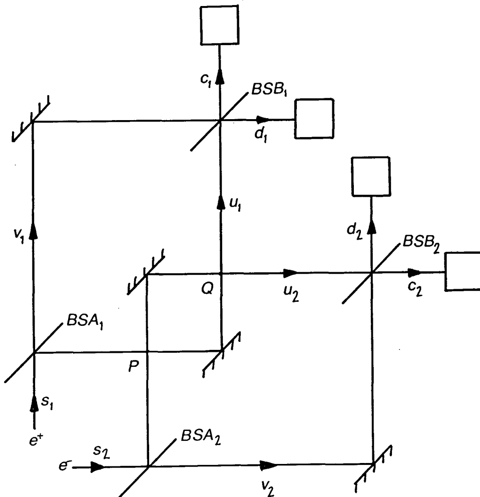
Fig. 9.3. Two overlapping interferometers, one for positrons and one for electrons.
