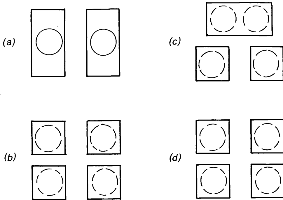
Fig. 8.3. The box shuffle for producing the two-atom entangled state that can be used to demonstrate Bell's theorem without inequalities.
