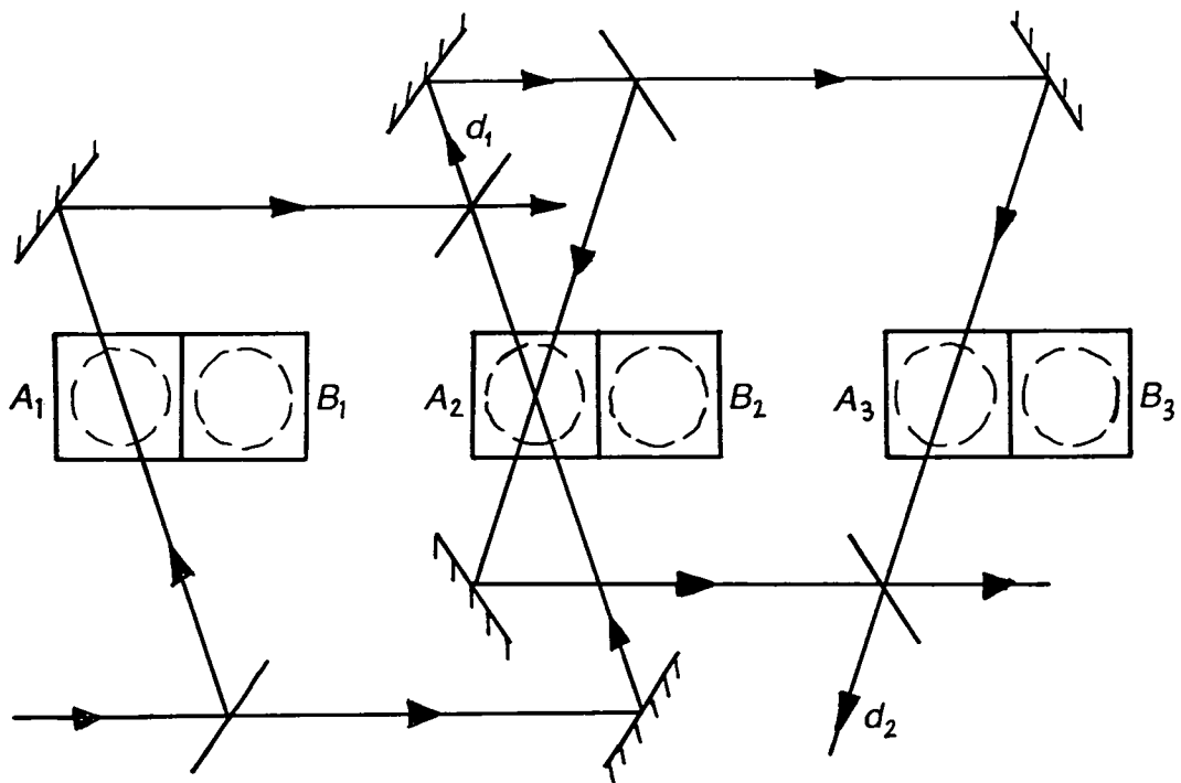
Fig. 7.1. Two entangled Mach-Zehnder interferometers arranged to produce a three atom entangled state.
