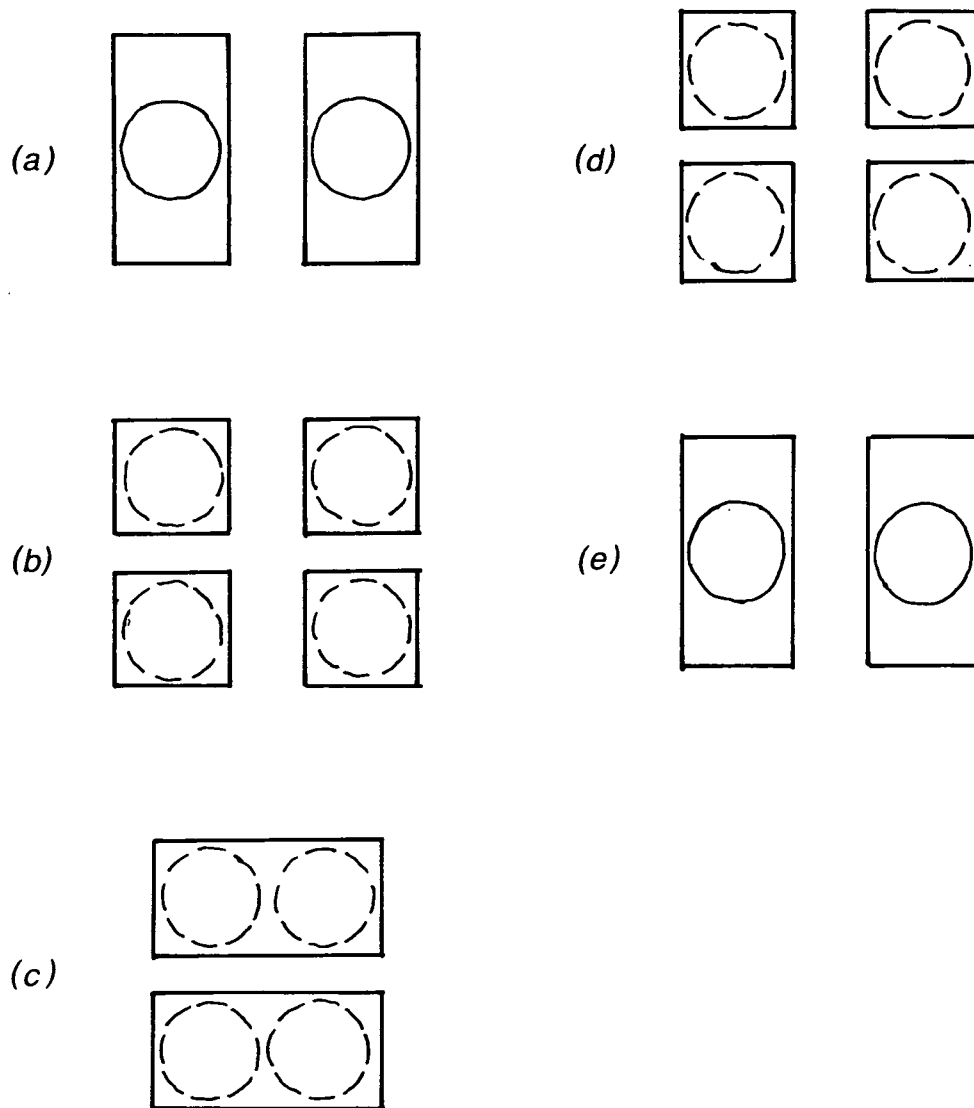
Fig. 5.3. Stages required to produce an entangled state by shuffling boxes.
