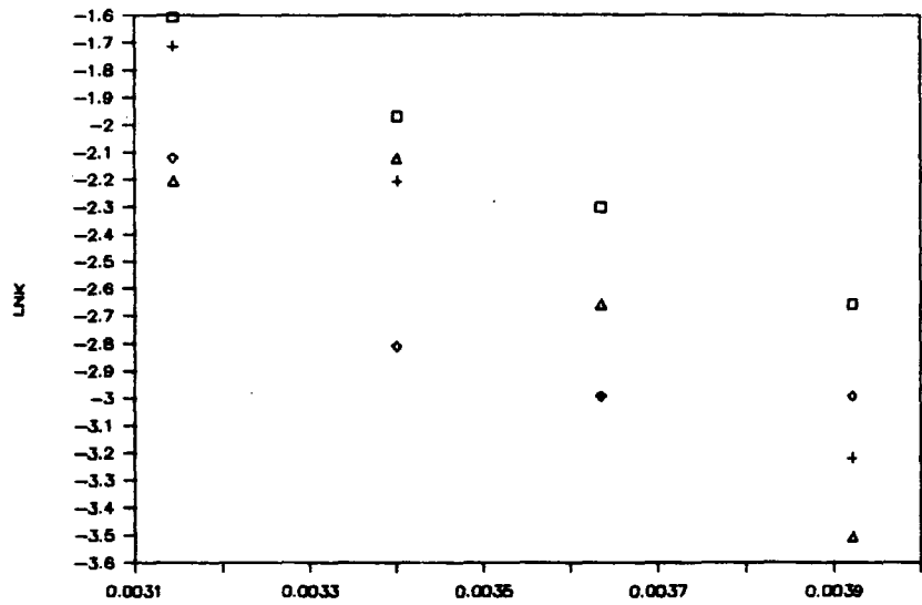
ARRHENIUS PLOT FOR SECOND PROCESS
