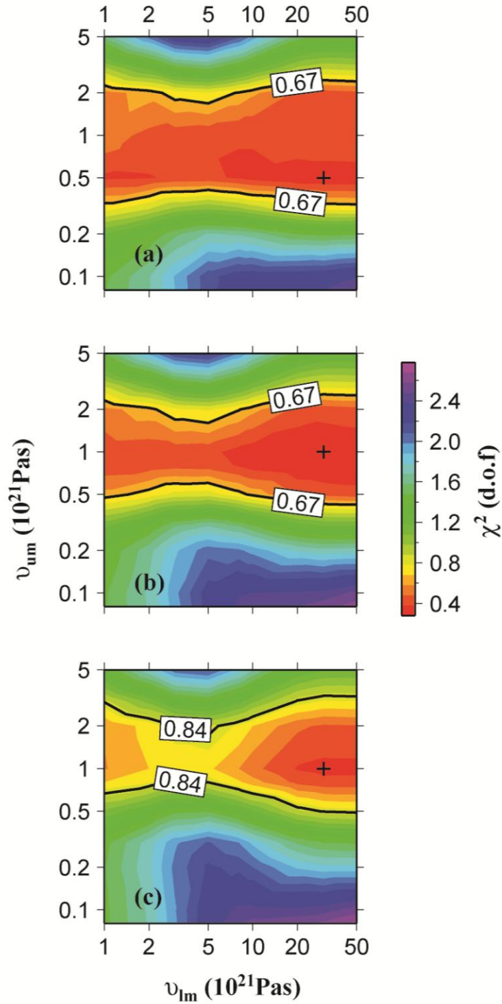
Fig. 3.3: \chi^2 values of data-model fit for a range of values for upper and lower mantle viscosity ( \nu_{um} and \nu_{lm} , respectively) and lithospheric thicknesses of (a) 71 km, (b) 96 km and (c) 120 km. The black line and cross in each frame represent, respectively, the \chi^2 value below which the quality of fit is equivalent at the 95% confidence level and the minimum value found
