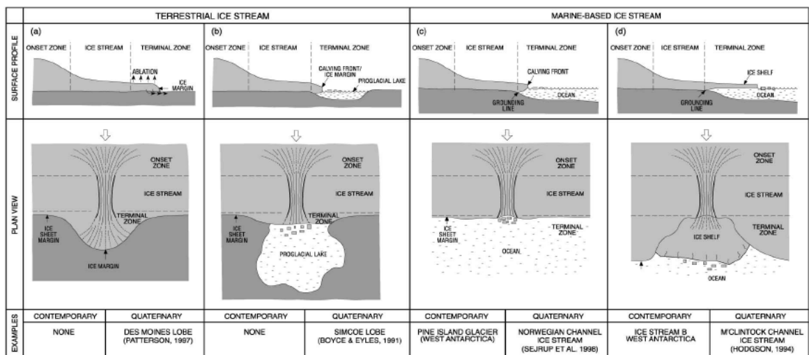
Figure.1. The two styles of ice streams. Both show clear flow convergence into a zone of rapid velocity that terminates in either a large lobate margin or calves into open water or an ice shelf. Marine based ice streams are easily able to remove material which renders them more susceptible to rapid velocity fluctuations (from Stokes and Clark, 2001)
